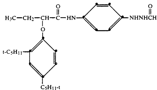
1-Formyl-2-phenylhydrazine
