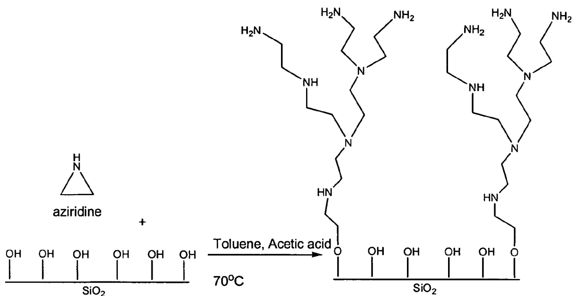
Scheme 1. Synthesis of Hyperbranched Ethylene-Amine-Grafted Silica Sorbents.
