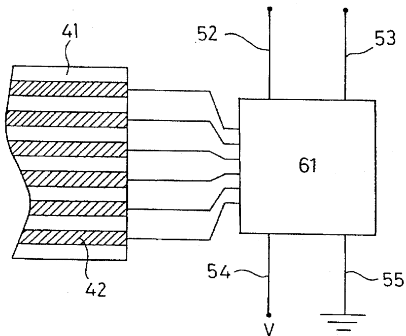
Fig.7 PRIOR ART
