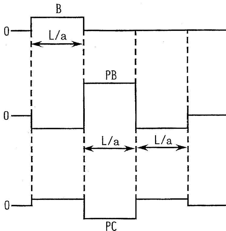
Fig.11 PRIOR ART
