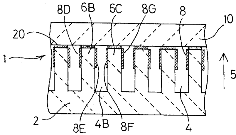
Fig.8 PRIOR ART
