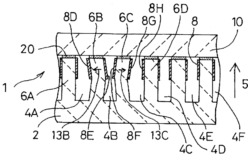
Fig.9 PRIOR ART
