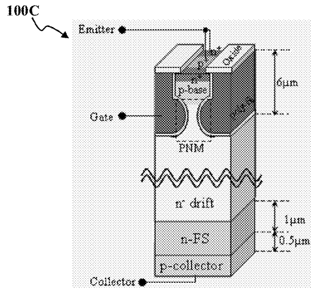
FIG. 1C (PRIOR ART)
