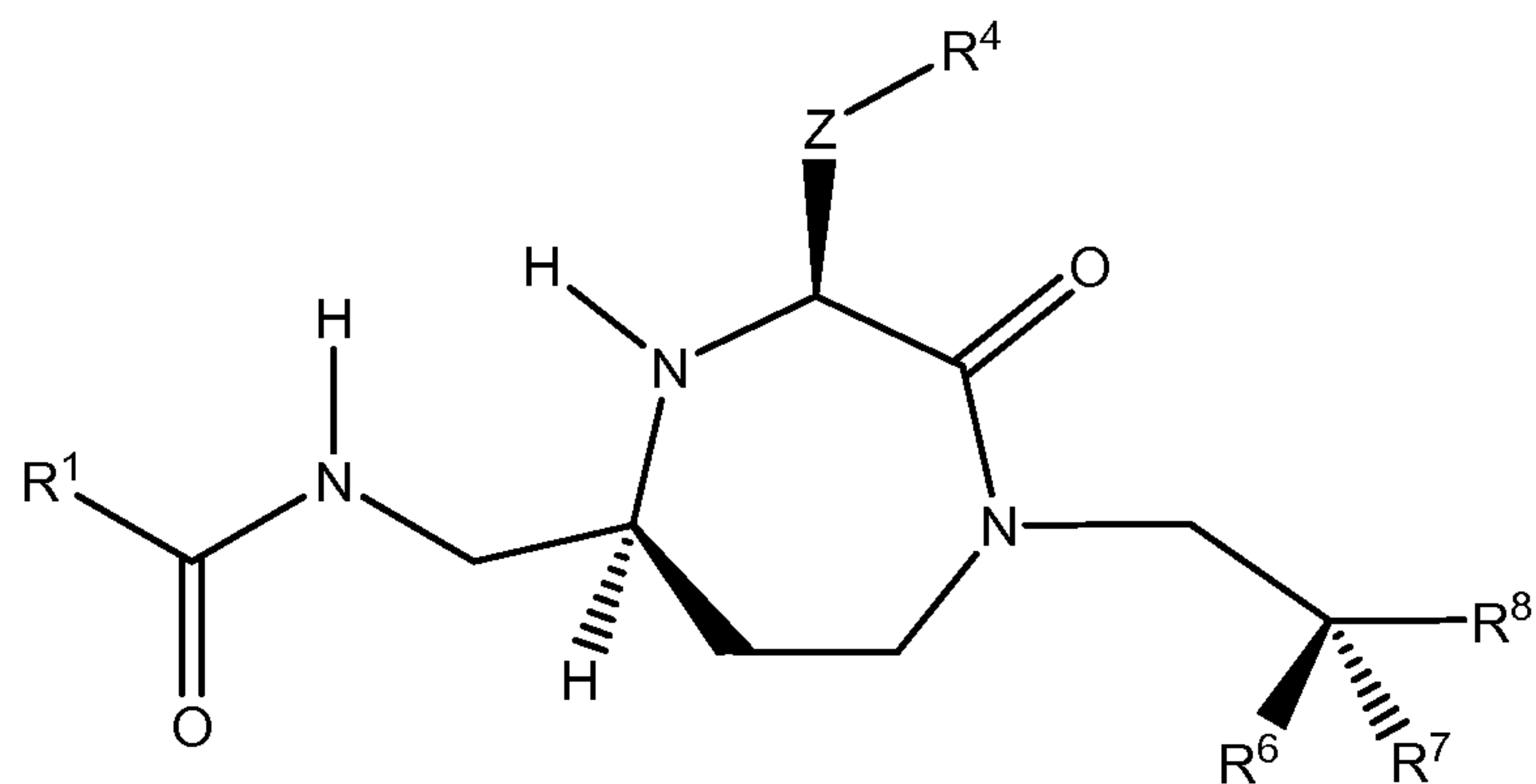
Formula (II)
