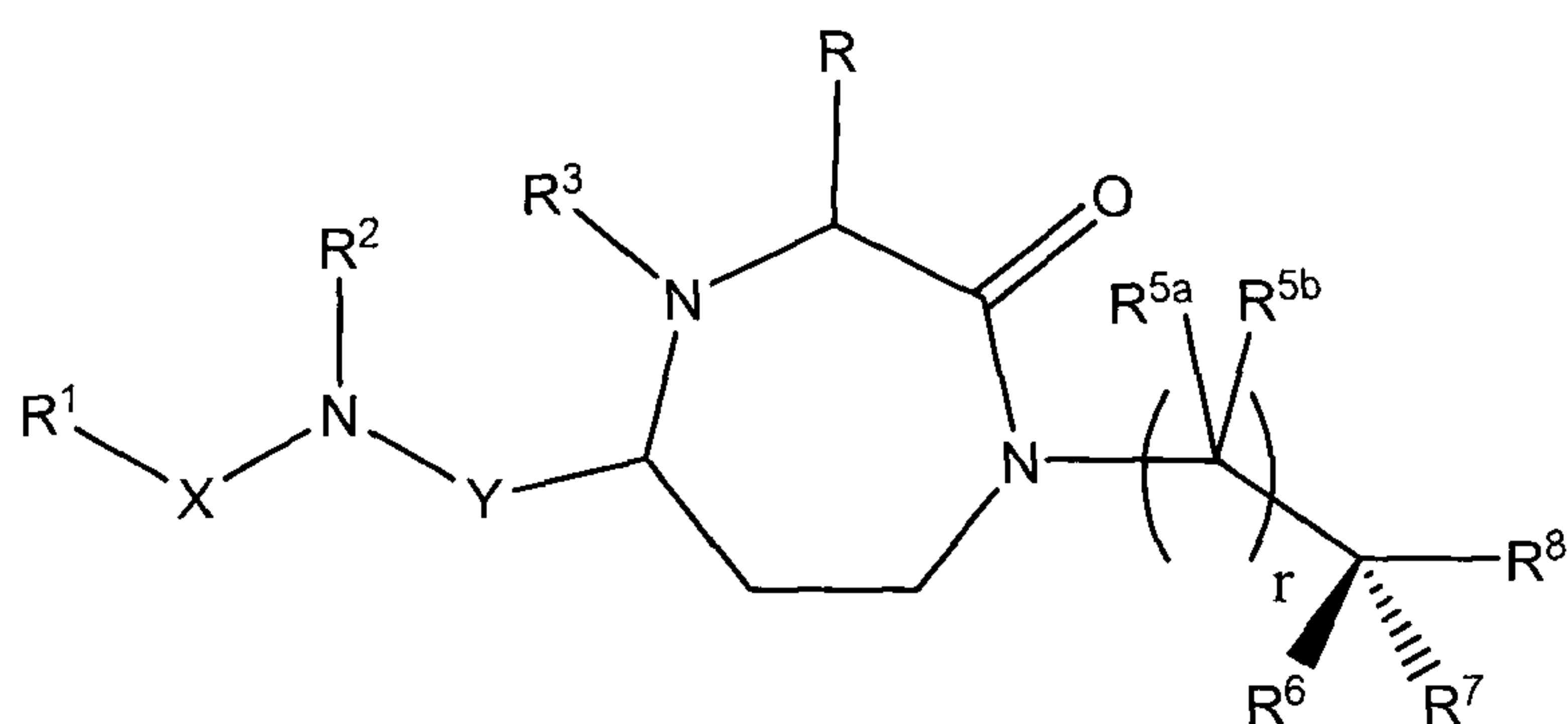
Formula (I)
