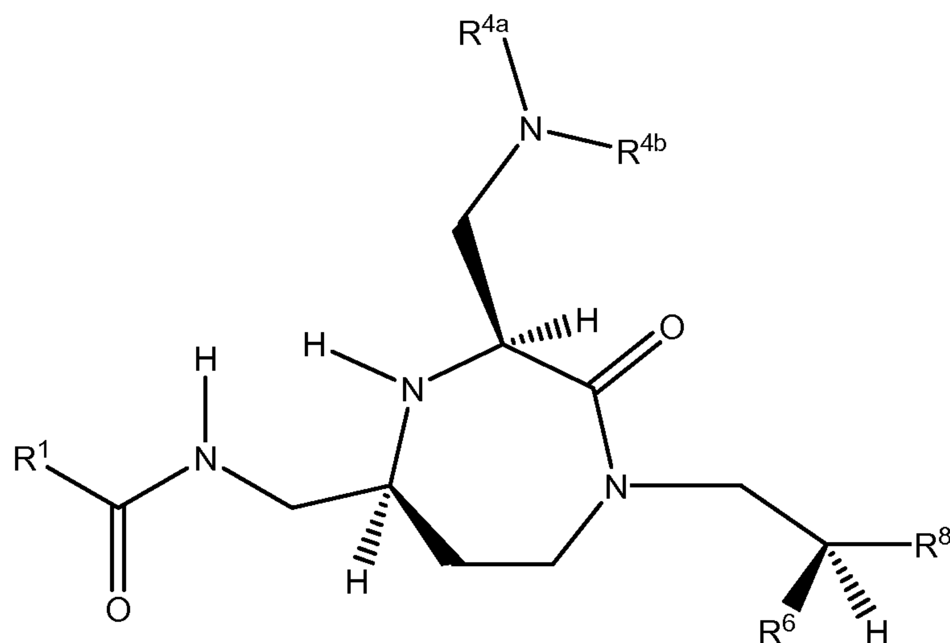
Formula (IIIa)
