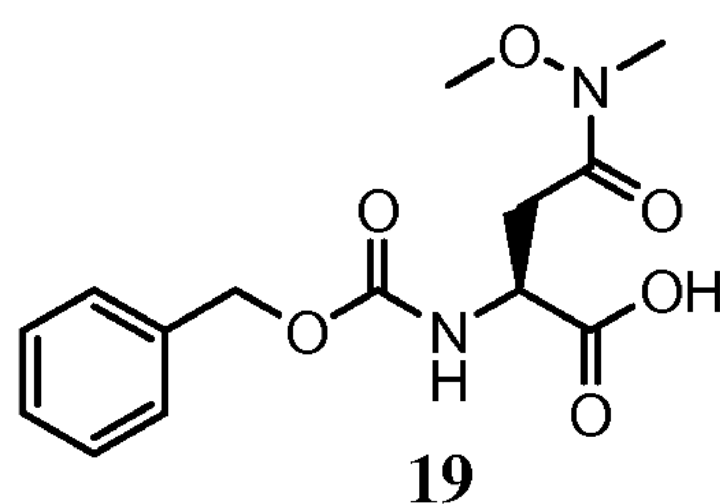
(S)-3-methyl-4,8-dioxo-10-phenyl-2,9-dioxa-3,7-diazadecane-6-carboxylic acid
