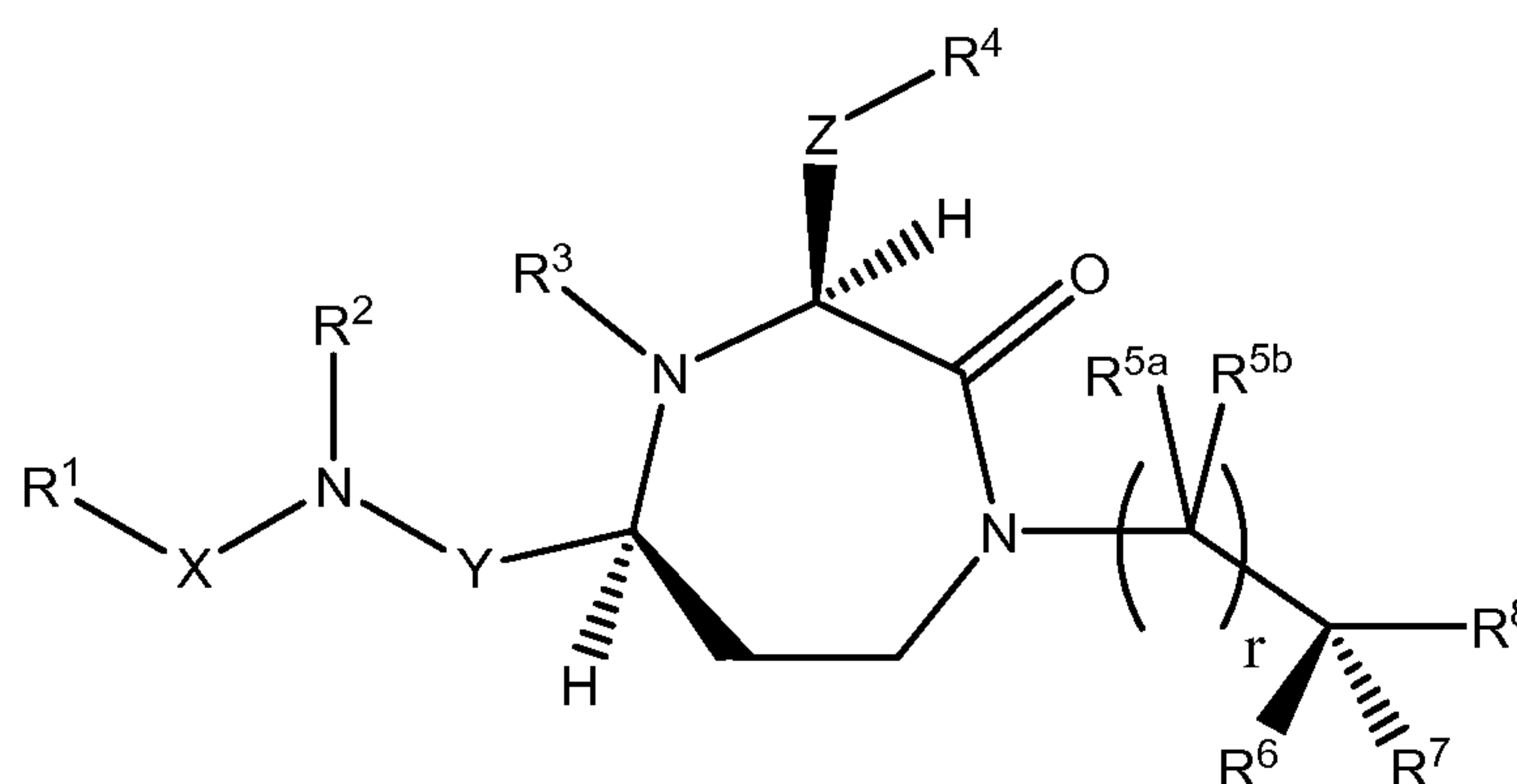
Formula (Ib)
