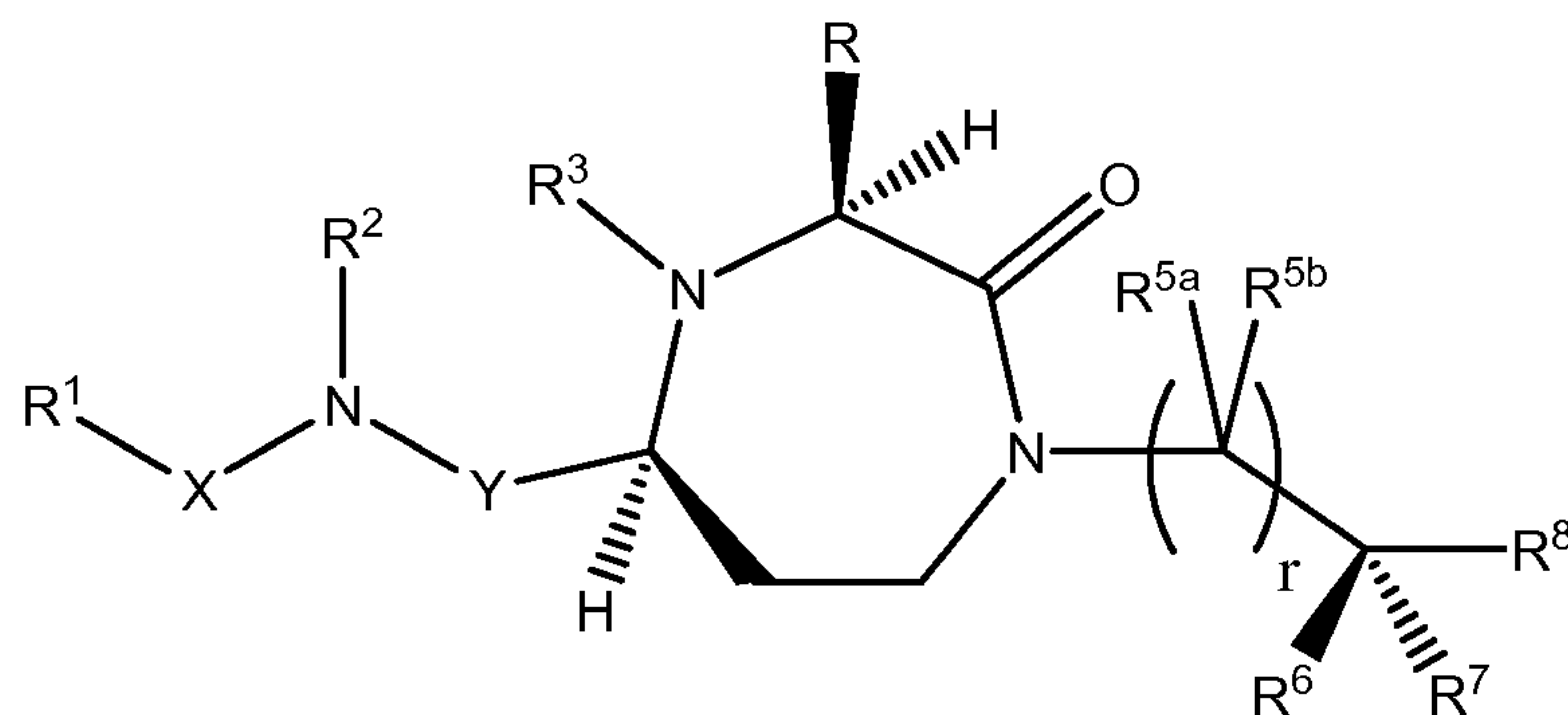
Formula (Ia)
