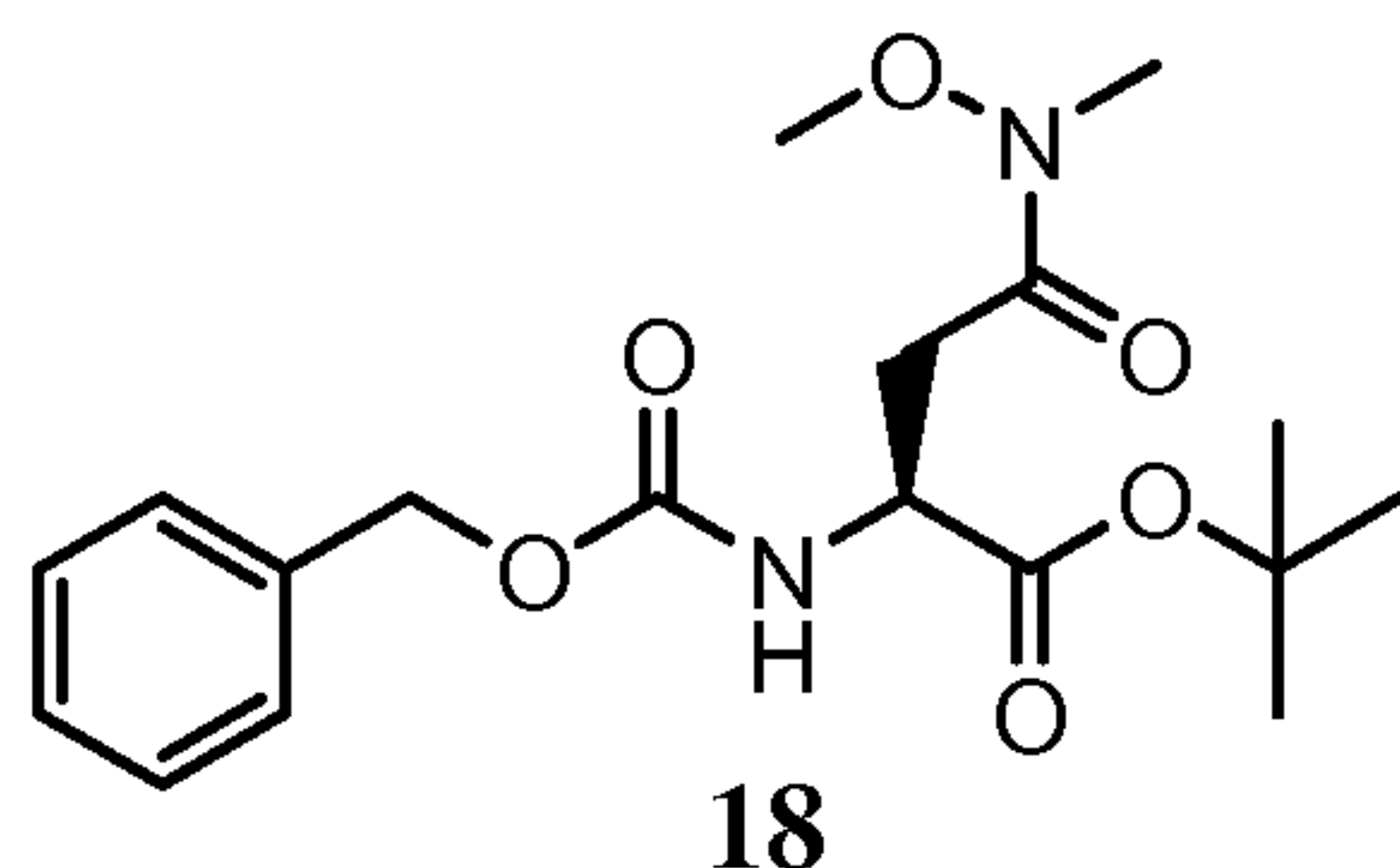
(S)-tert-butyl 3-methyl-4,8-dioxo-10-phenyl-2,9-dioxa-3,7-diazadecane-6-carboxylate
