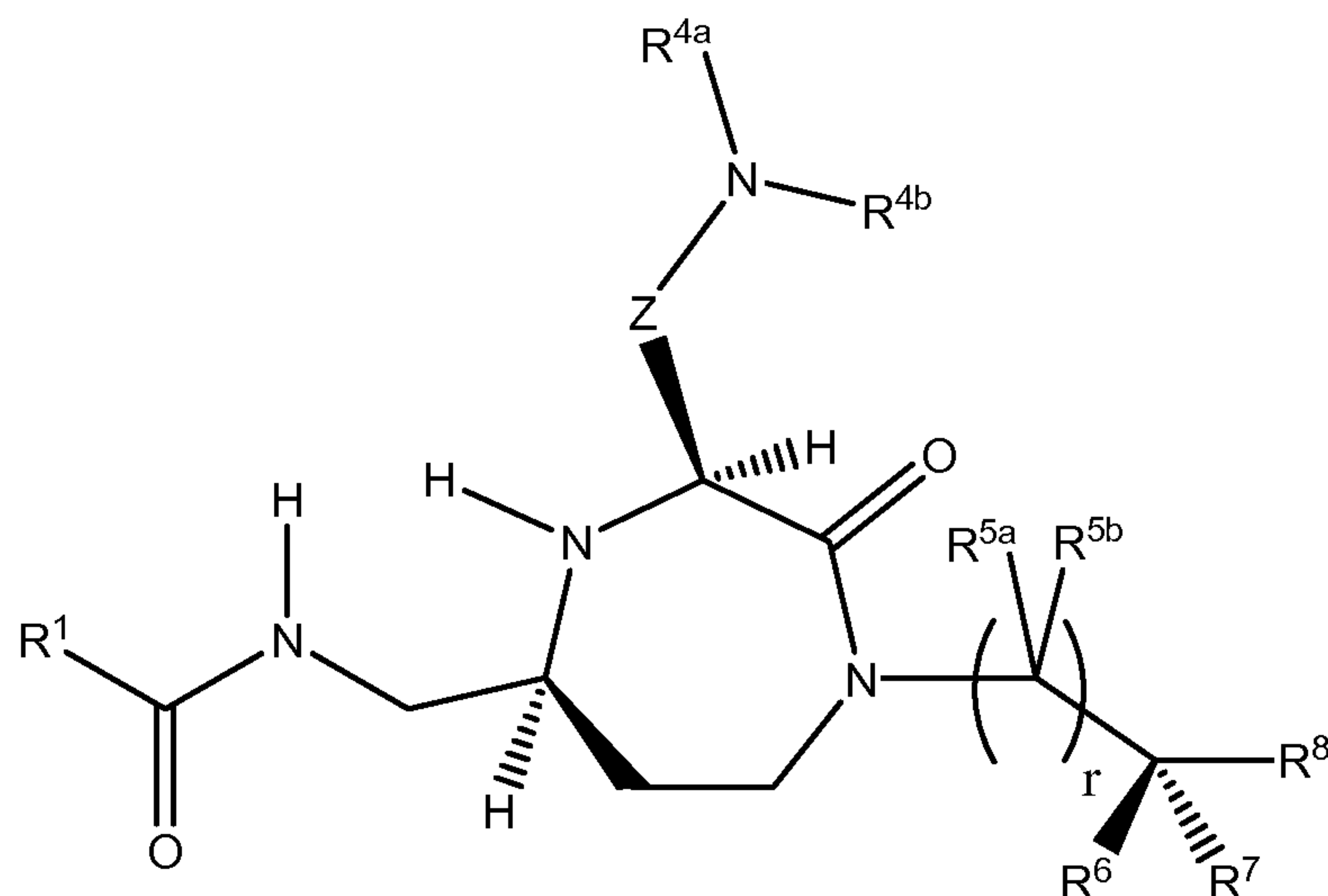
Formula (Id)
