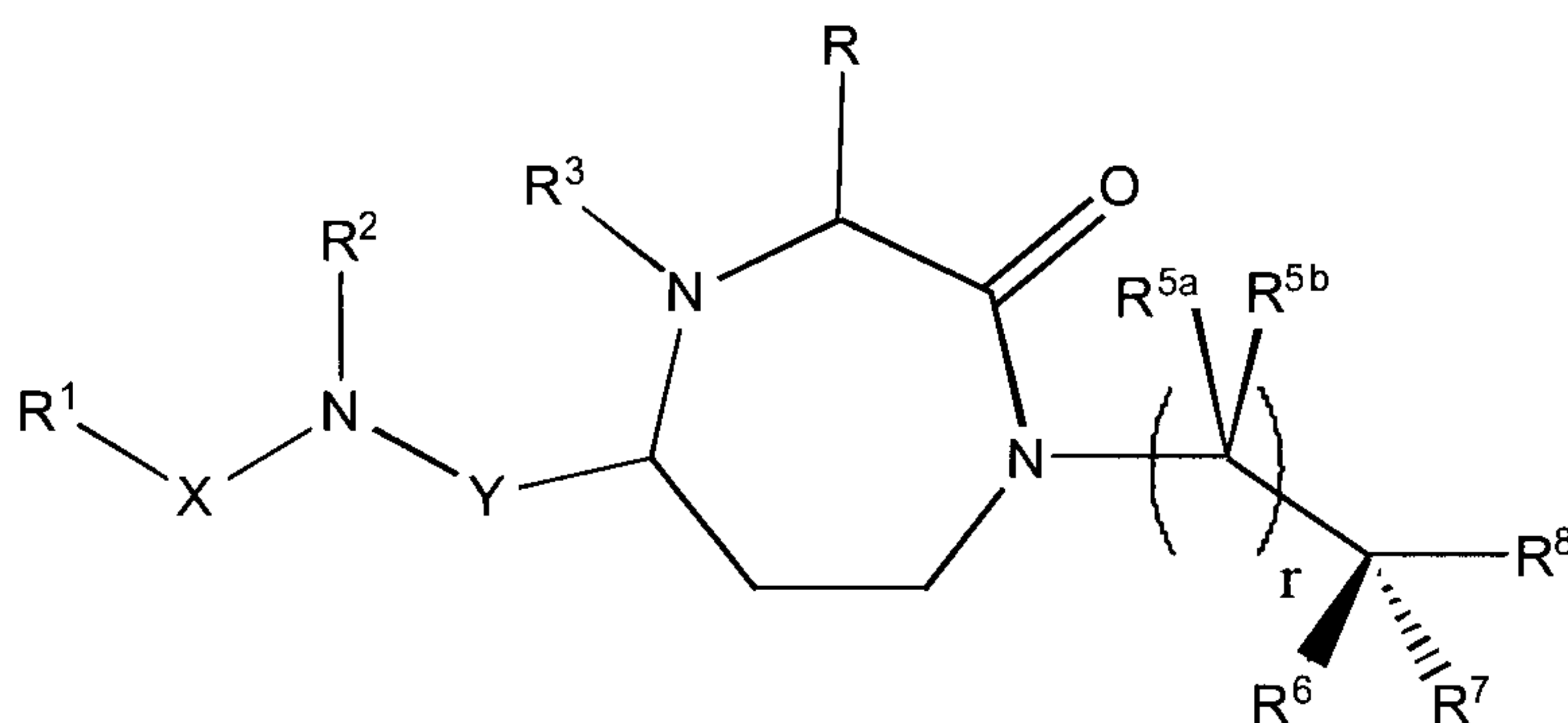
Formula (I)
