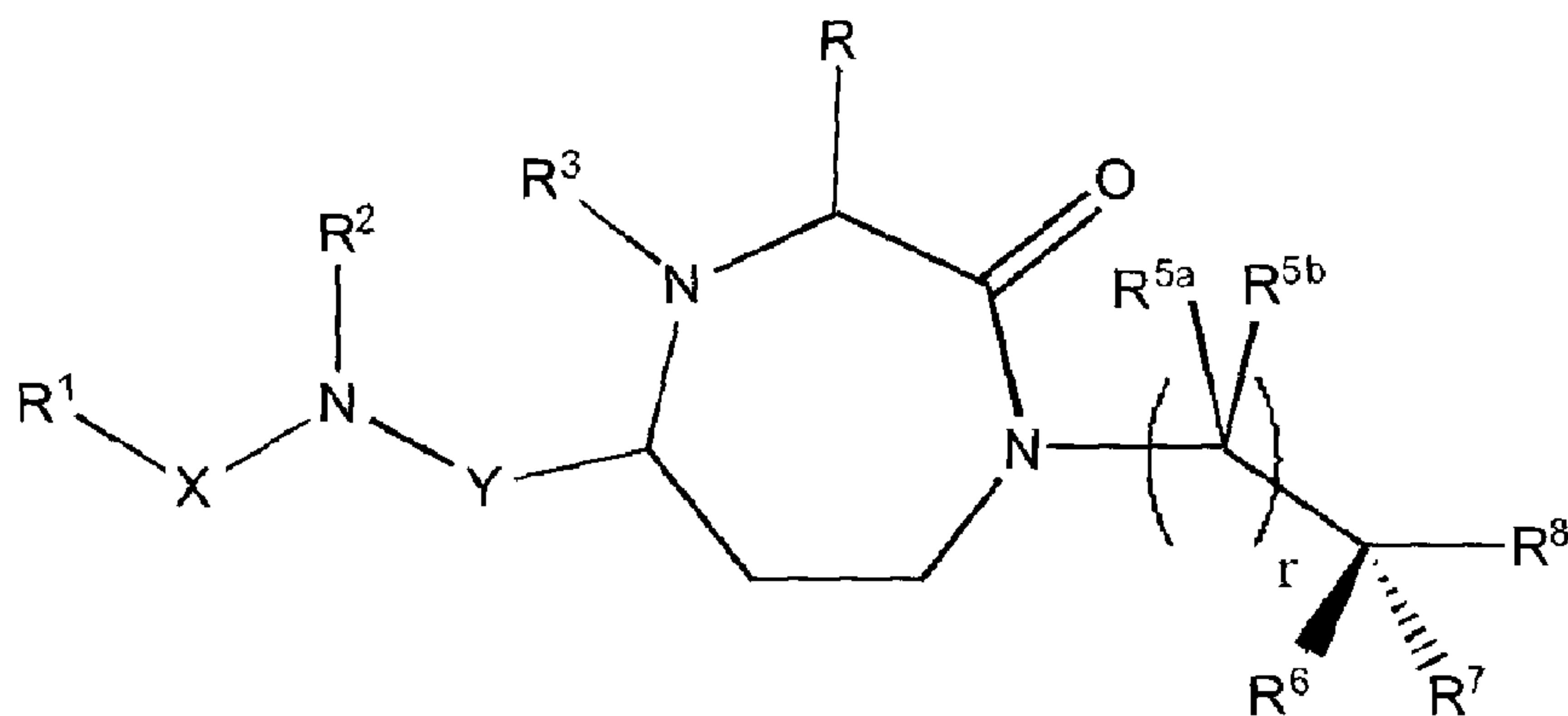
Formula (I)
