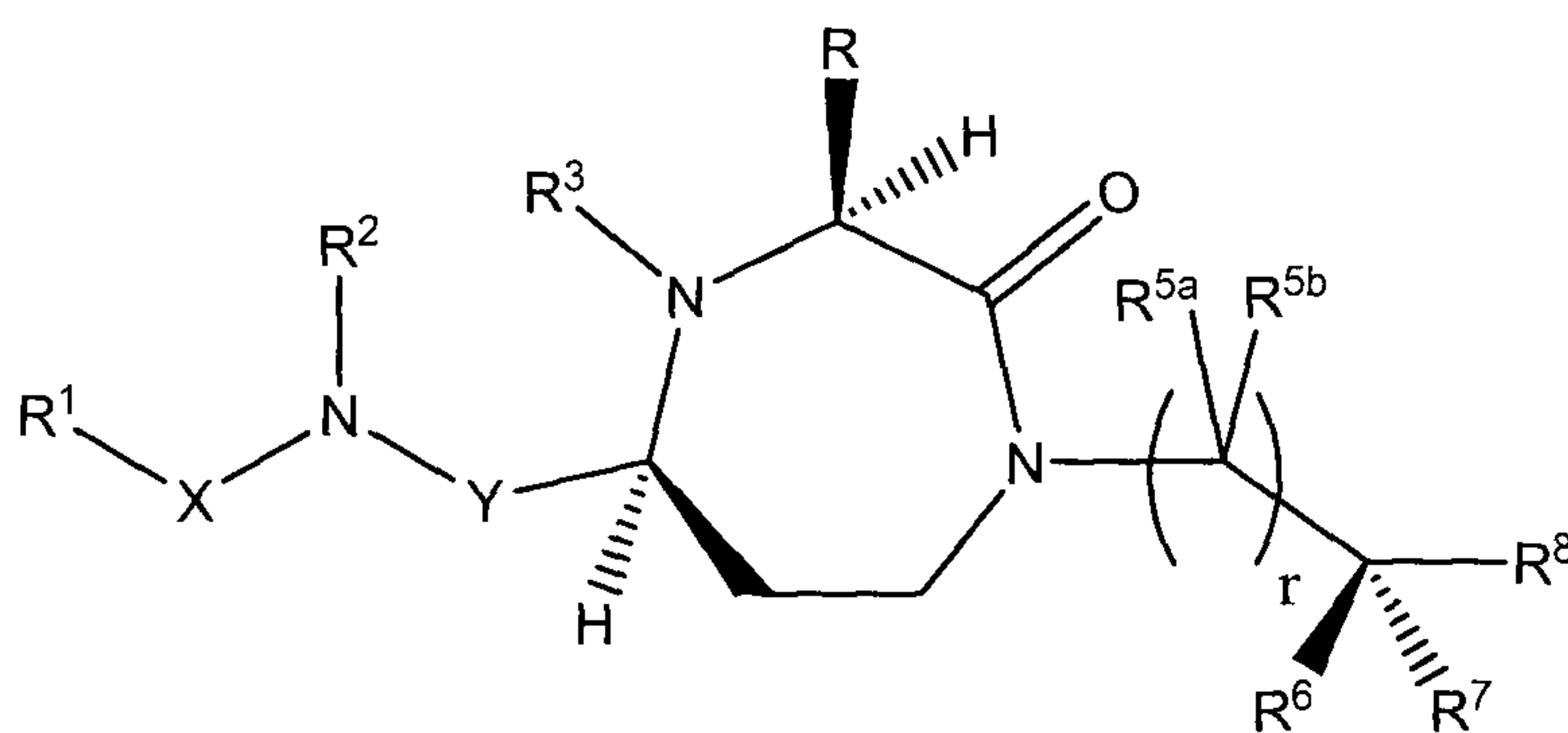
Formula (Ia)
