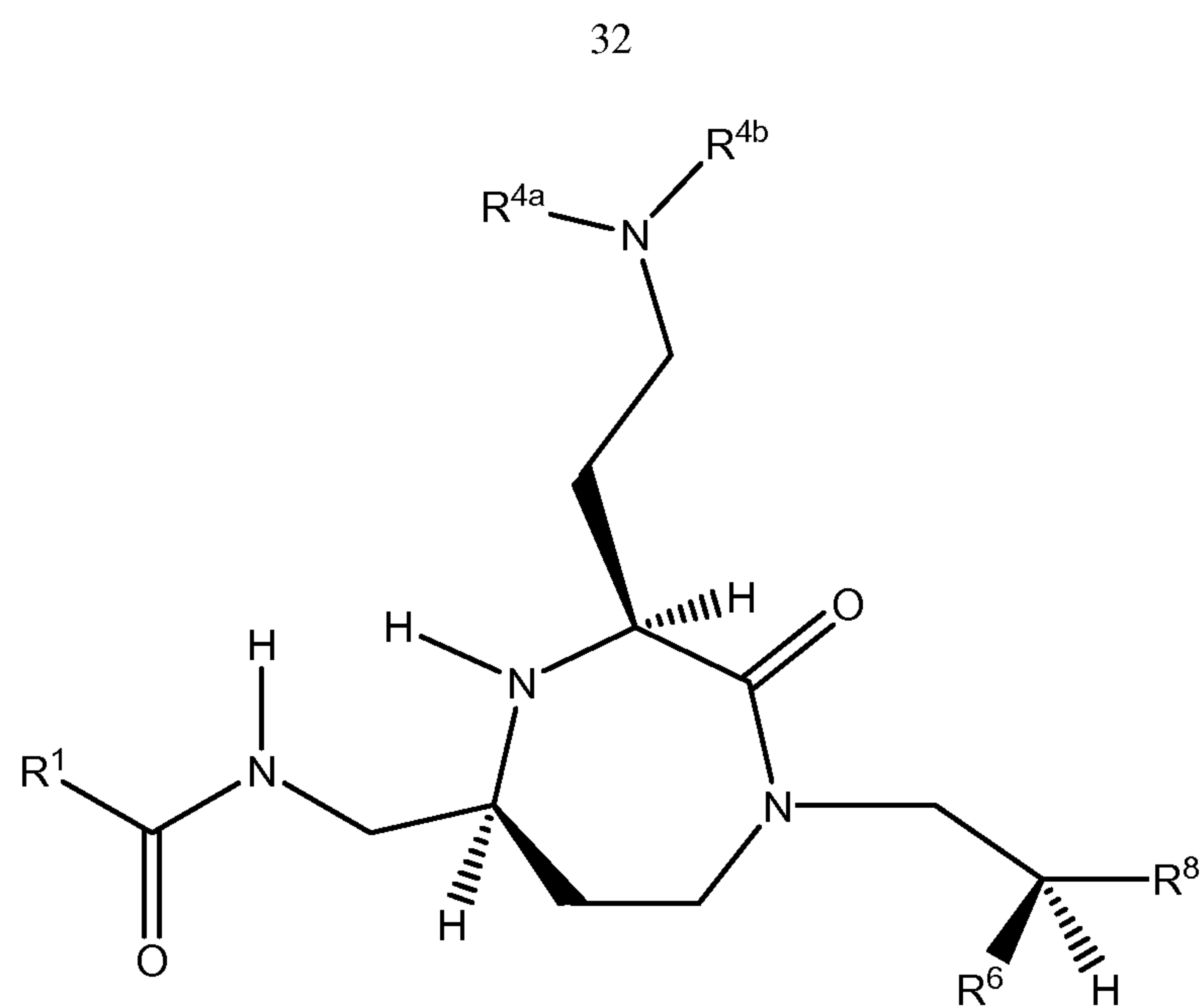
Formula (IIIb)
