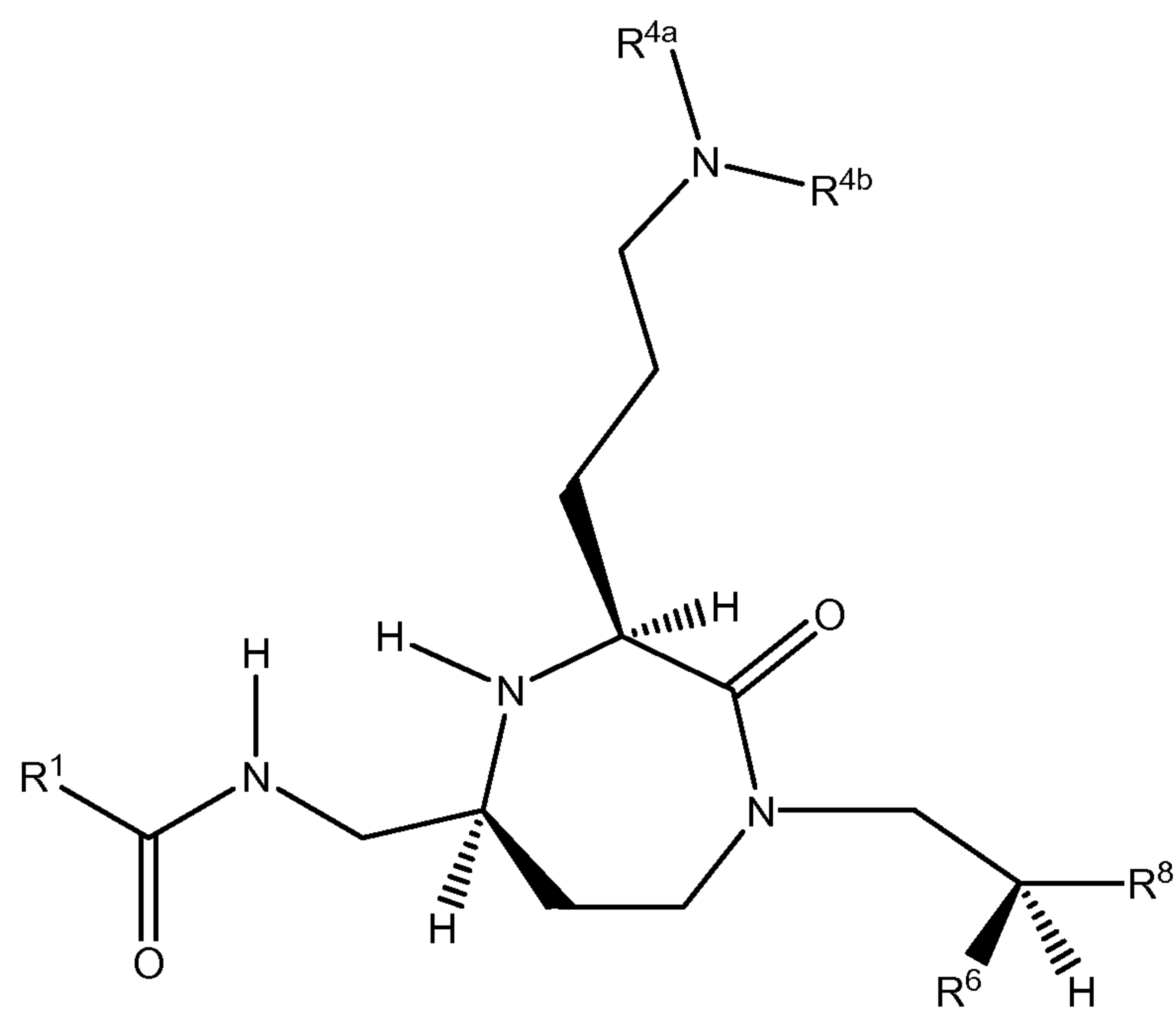
Formula (IIIc)
