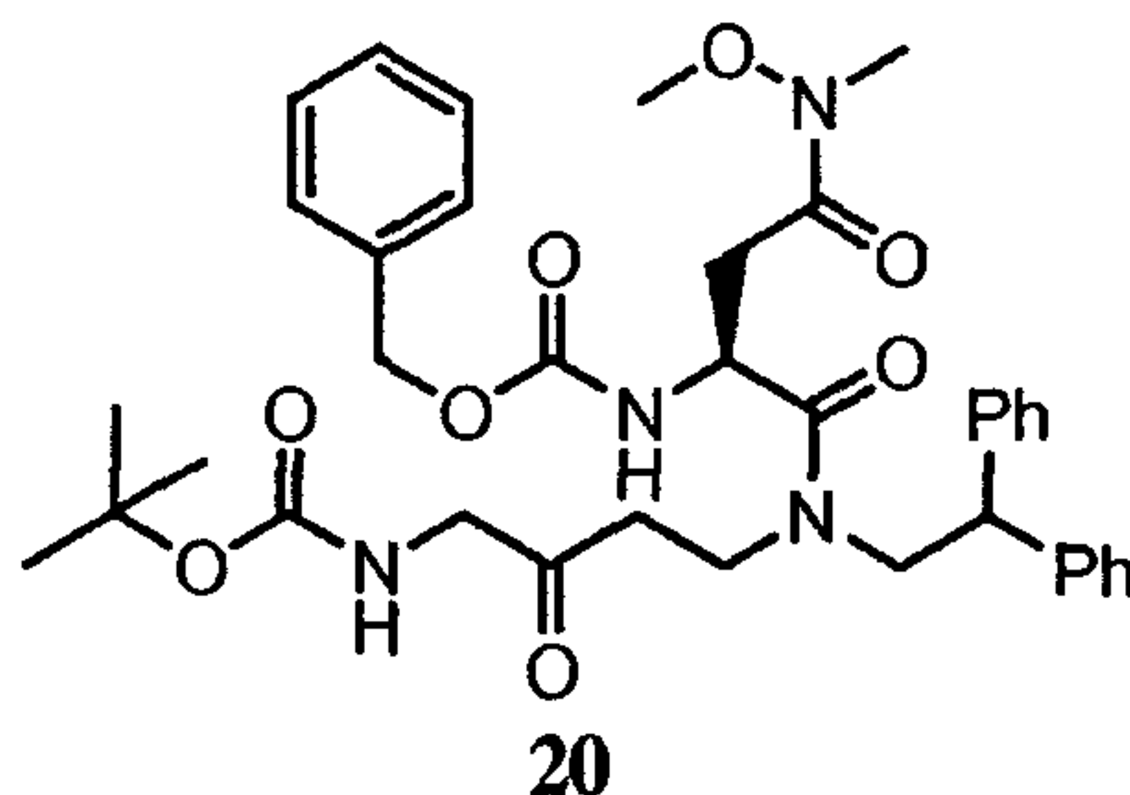
(S)-benzyl 8-(2,2-diphenylethyl)-3,16,16-trimethyl-4,7,11,14-tetraoxo-2,15-dioxa-3,8,13-triazaheptadecan-6-ylcarbamate
