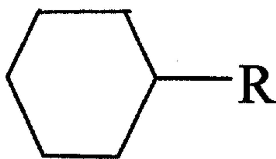
Alkylcyclohexane
