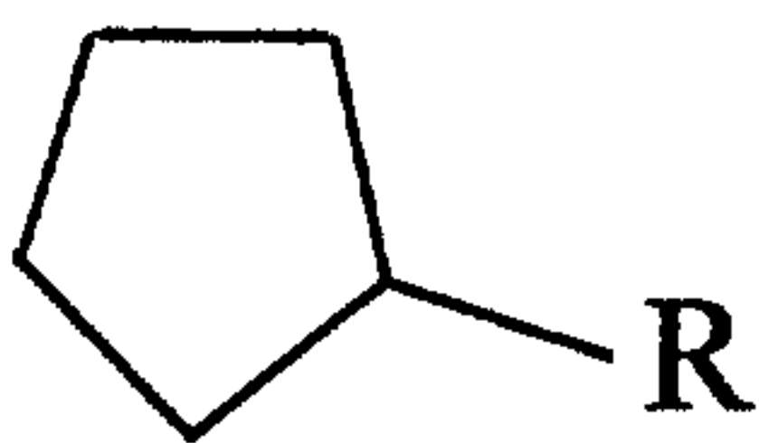
Alkylcyclopentane
