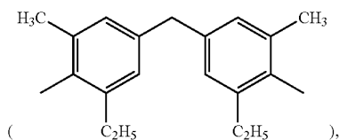
3,3'-dimethyl-5,5'-diethyl-4,4'-diphenylmethane group
