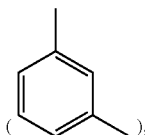
bisphenol A diphenyl ether group
