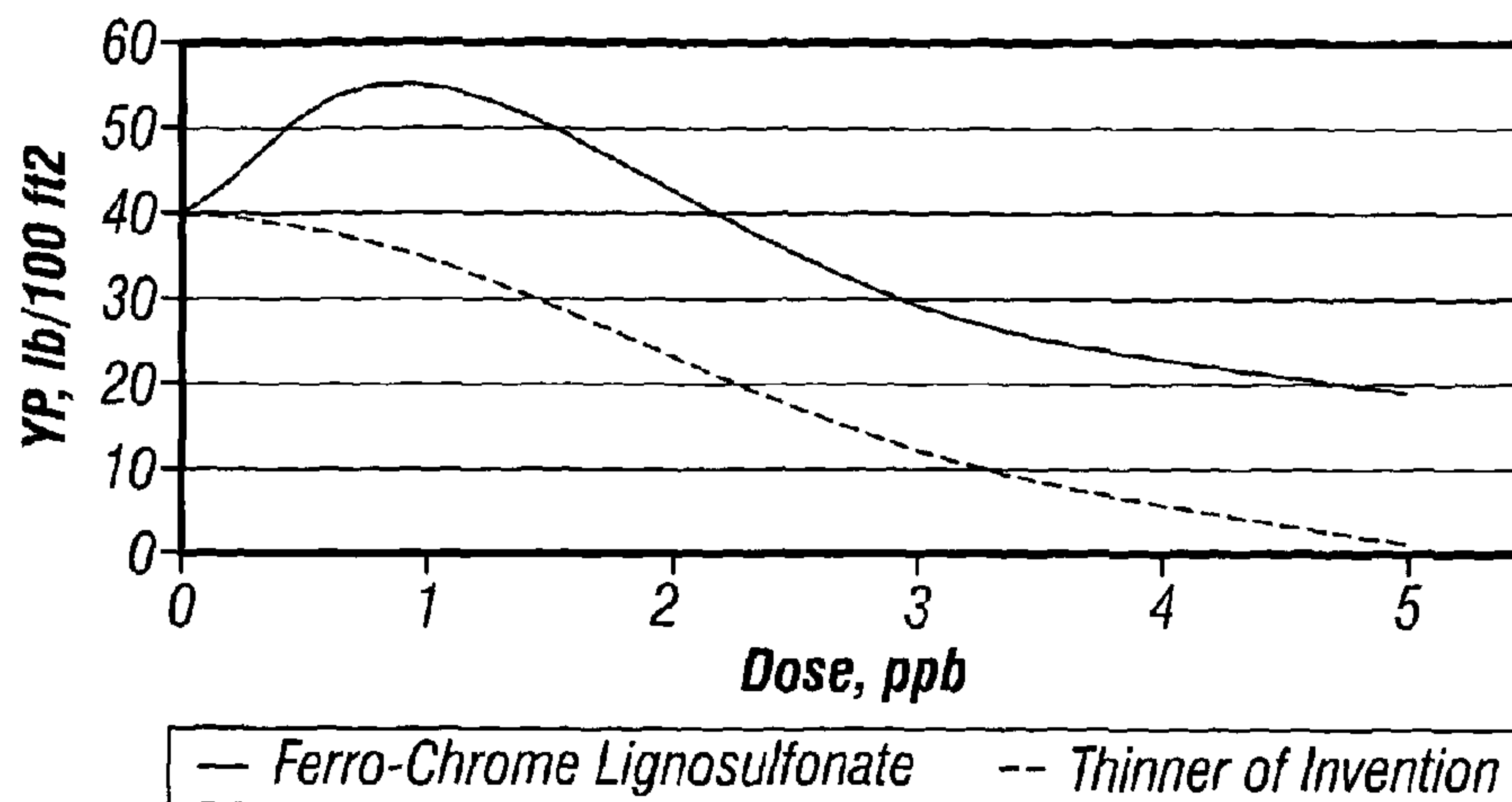
Yield Point vs Dispersant Concentration in Gypsum/Salt Water, 22lb/bbl AQUAGEL, 66lb/bbl Rev Dust, HR at 150°F (10 > pH > 9.2)
