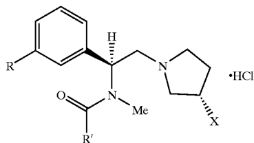
Compounds of Formula IIIA
