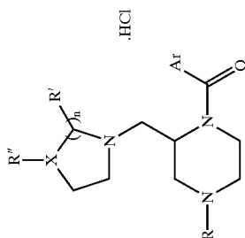
Compounds of Formula IA
