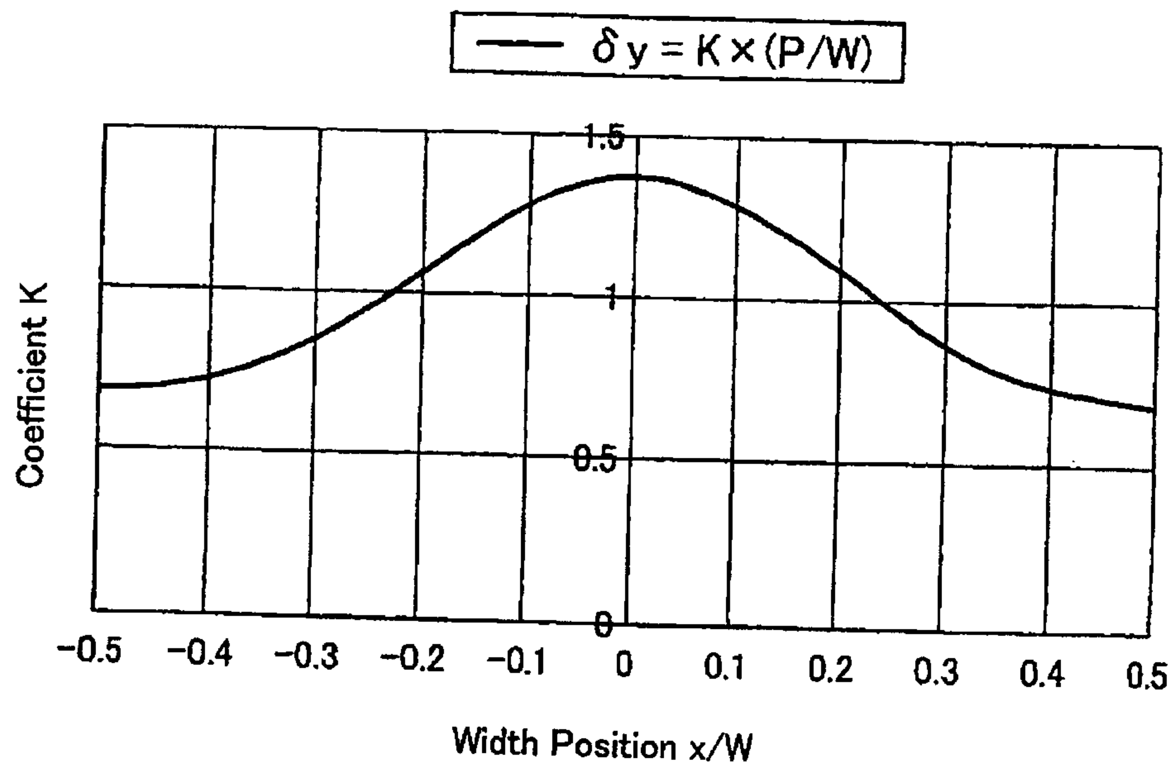
(b) Relationship between Width Position and Coefficient K at y = 0 when C = 0.5 W
