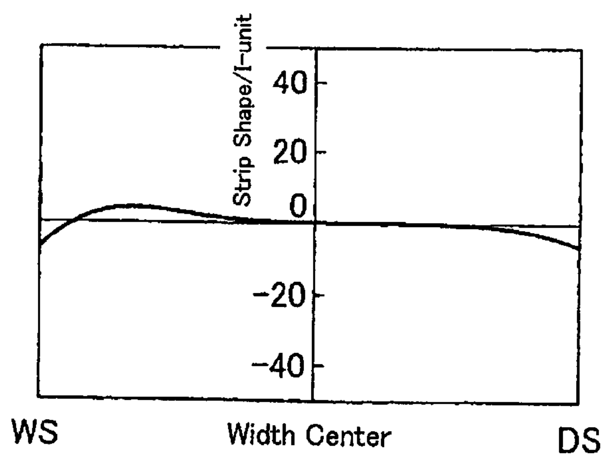
(c) Strip-Widthwise Distribution of Elongation difference
