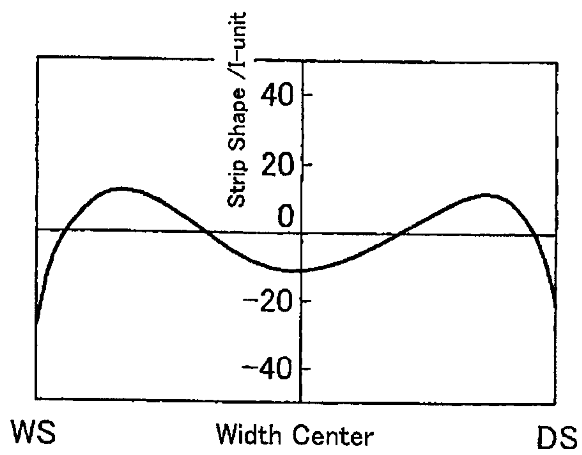
(a) Measurement Result of Shape Meter
