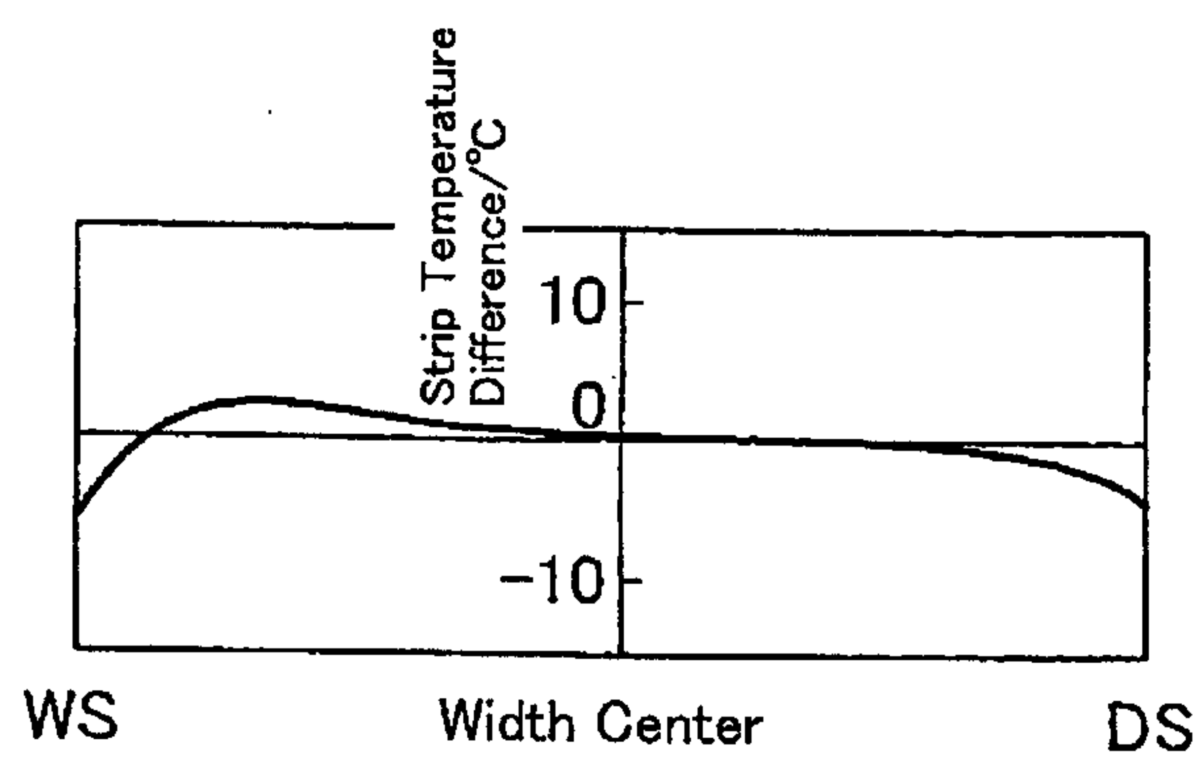
(b) Strip-Widthwise Temperature Distribution
