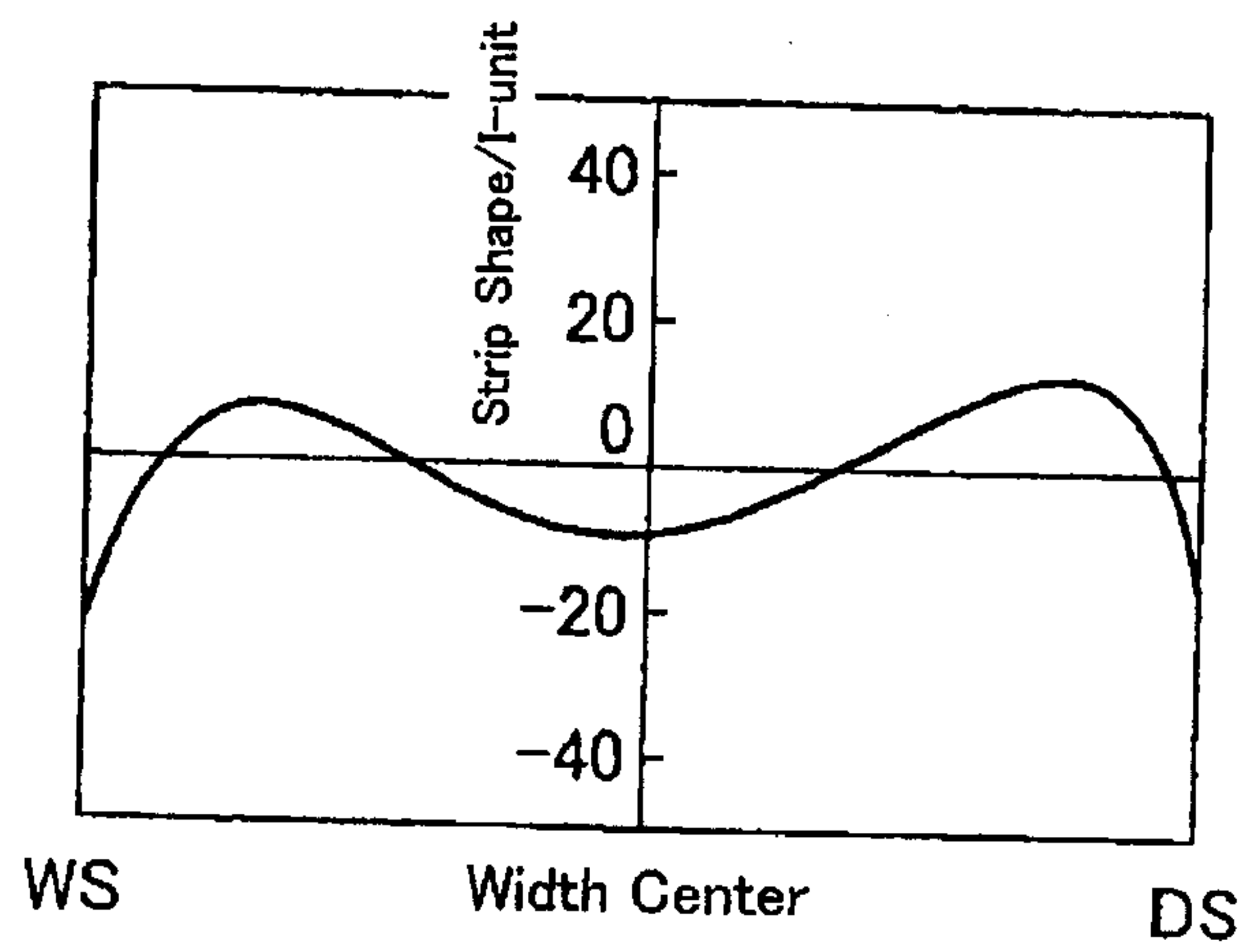
(d) Pre-Cooling Shape on Delivery Side of Finishing Mill Line
