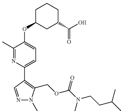
(1S,3S)-3-((6-(5-(((isopentyl)(methyl)carbamoyl)oxy)methyl)-1-methyl-1H-pyrazol-4-yl)-2-methylpyridin-3-yl)oxy)cyclohexane-1-carboxylic acid
