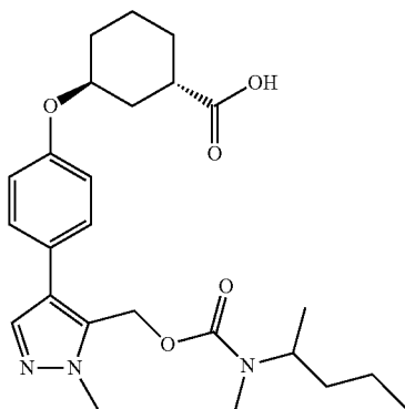
(1S,3S)-3-(4-(1-methyl-5-(((methyl(pentan-2-yl)carbamoyl)oxy)methyl)-1H-pyrazol-4-yl)phenoxy)cyclohexane-1-carboxylic acid
