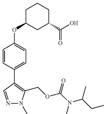
(1S,3S)-3-(4-(5-(((sec-butyl(methyl)carbamoyl)oxy)methyl)-1-methyl-1H-pyrazol-4-yl)phenoxy)cyclohexane-1-carboxylic acid
