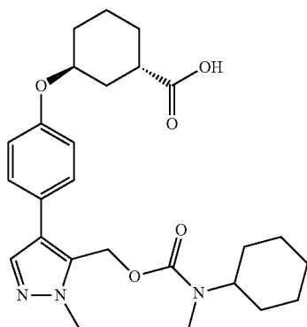
(±)-trans-3-(4-(5-(((cyclohexyl(methyl)carbamoyl)oxy)methyl)-1-methyl-1H-pyrazol-4-yl)phenoxy)cyclohexane-1-carboxylic acid
