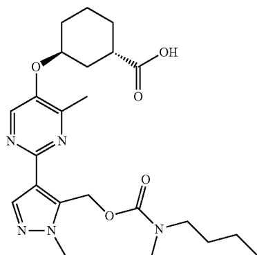
(1S,3S)-3-((2-(5-(((butyl(methyl)carbamoyl)oxy)methyl)-1-methyl-1H-pyrazol-4-yl)-4-methylpyrimidin-5-yl)oxy)cyclohexane-1-carboxylic acid
