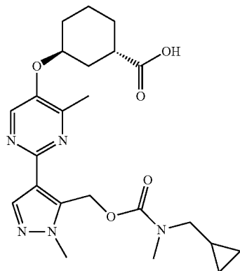
(1S,3S)-3-((2-(5-(((cyclopropylmethyl)(methyl)carbamoyl)oxy)methyl)-1-methyl-1H-pyrazol-4-yl)-4-methylpyrimidin-5-yl)oxy)cyclohexane-1-carboxylic acid
