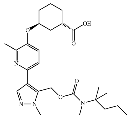
(rac)-trans-3-((2-methyl-6-(1-methyl-5-(((methyl(2-methylpentan-2-yl)carbamoyl)oxy)methyl)-1H-pyrazol-4-yl)pyridin-3-yl)oxy)cyclohexane-1-carboxylic acid
