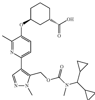
(1S,3S)-3-((6-(5-(((dicyclopropylmethyl)(methyl)carbamoyl)oxy)methyl)-1-methyl-1H-pyrazol-4-yl)-2-methylpyridin-3-yl)oxy)cyclohexane-1-carboxylic acid
