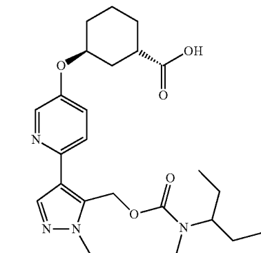
(1S,3S)-3-((6-(1-methyl-5-(((methyl(pentan-3-yl)carbamoyl)oxy)methyl)-1H-pyrazol-4-yl)pyridin-3-yl)oxy)cyclohexane-1-carboxylic acid
