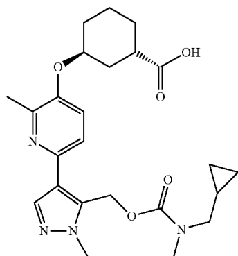
(1S,3S)-3-((6-(5-(((cyclopropylmethyl)(methyl)carbamoyl)oxy)methyl)-1-methyl-1H-pyrazol-4-yl)-2-methylpyridin-3-yl)oxy)cyclohexane-1-carboxylic acid
