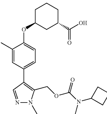
(1S,3S)-3-(4-(5-(((cyclobutyl(methyl)carbamoyl)oxy)methyl)-1-methyl-1H-pyrazol-4-yl)-2-methylphenoxy)cyclohexane-1-carboxylic acid
