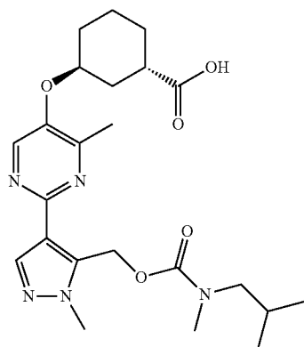
(1S,3S)-3-((2-(5-(((isobutyl(methyl)carbamoyl)oxy)methyl)-1-methyl-1H-pyrazol-4-yl)-4-methylpyrimidin-5-yl)oxy)cyclohexane-1-carboxylic acid
