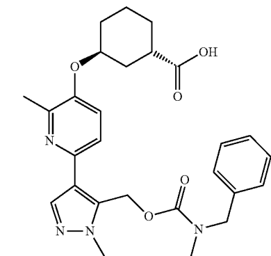
(rac)-trans-3-((6-(5-(((benzyl(methyl)carbamoyl)oxy)methyl)-1-methyl-1H-pyrazol-4-yl)-2-methylpyridin-3-yl)oxy)cyclohexane-1-carboxylic acid
