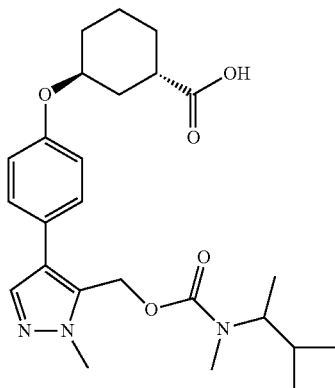
(1S,3S)-3-(4-(5-(((1-cyclobutylethyl)(methyl)carbamoyl)oxy)methyl)-1-methyl-1H-pyrazol-4-yl)phenoxy)cyclohexane-1-carboxylic acid
