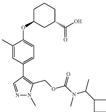
(1S,3S)-3-(4-(5-(((1-cyclobutyl-ethyl)(methyl)carbamoyl)oxy)methyl)-1-methyl-1H-pyrazol-4-yl)-2-methylphenoxy)cyclohexane-1-carboxylic acid
