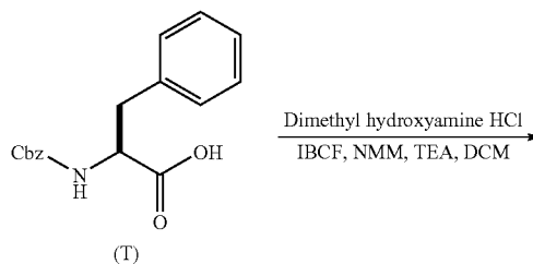
Scheme 4: Synthesis of Example 4
