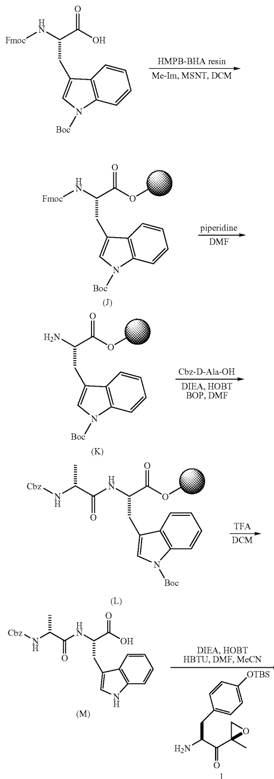
Scheme 2: Synthesis of Example 2
