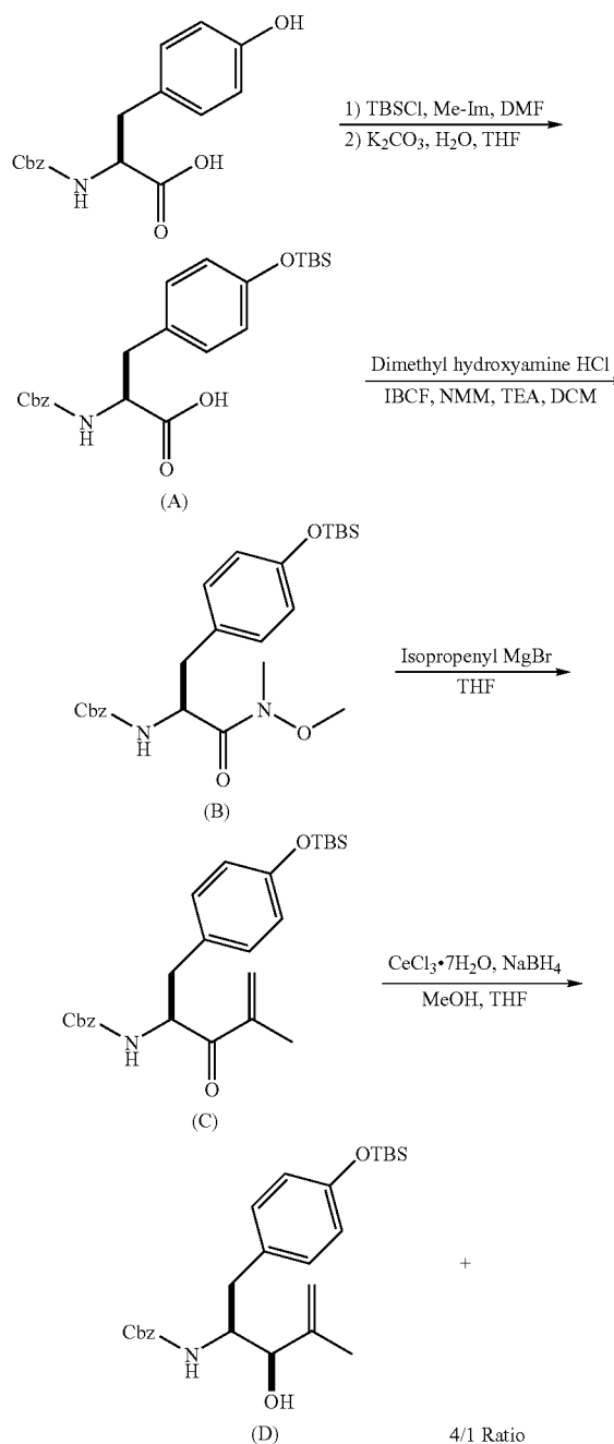
Scheme 1: Synthesis of Example 1
