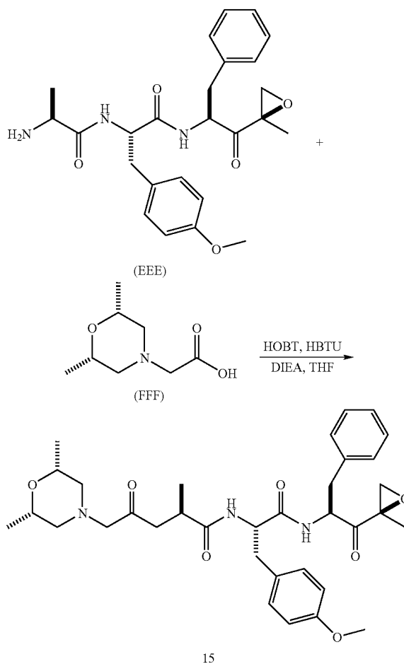
Scheme 15: Synthesis of Example 15
