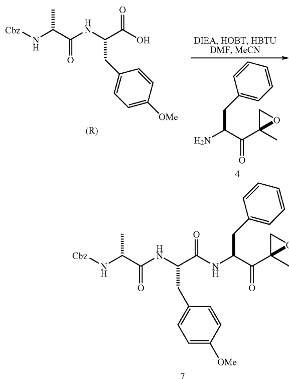
Scheme 7: Synthesis of Example 7
