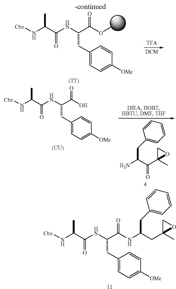
Scheme 12: Synthesis of Example 12
