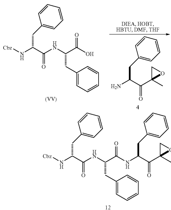
Scheme 12: Synthesis of Example 12
