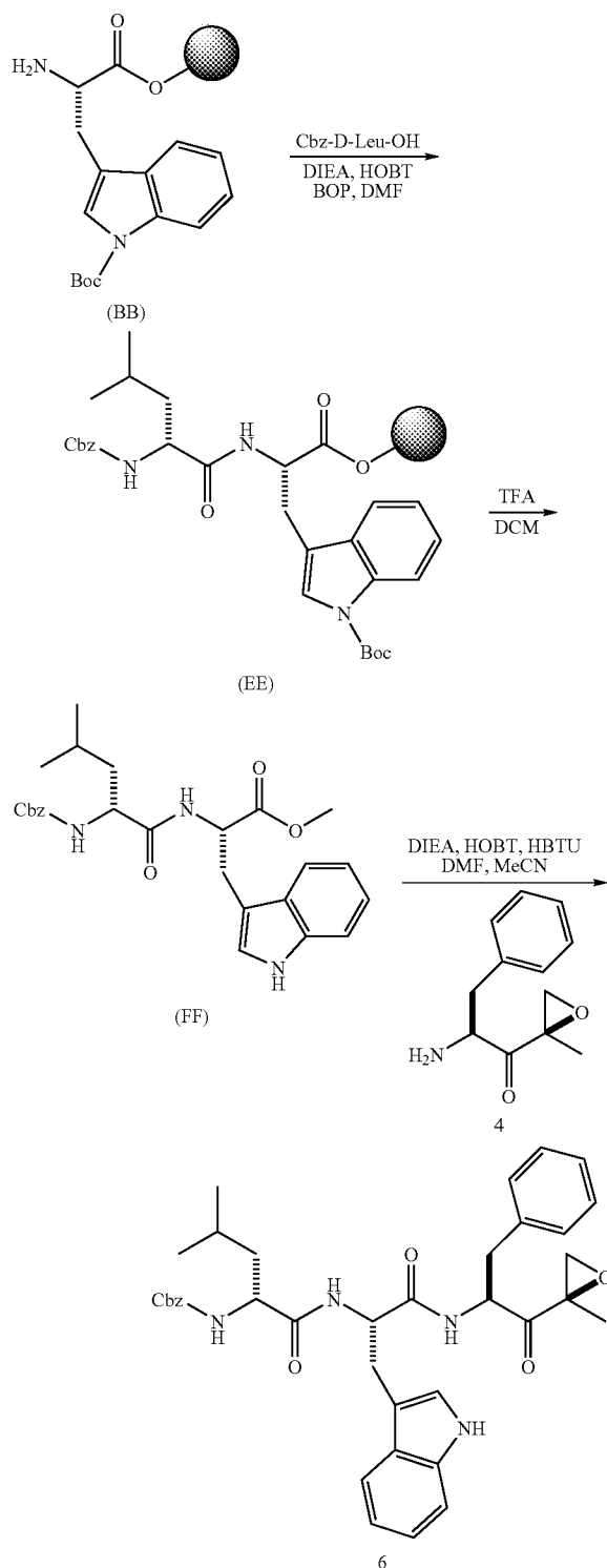
Scheme 6: Synthesis of Example 6
