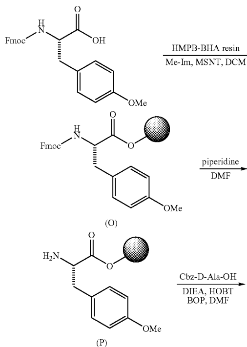
Scheme 3: Synthesis of Example 3
