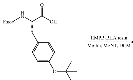
Scheme 13: Synthesis of Example 13
