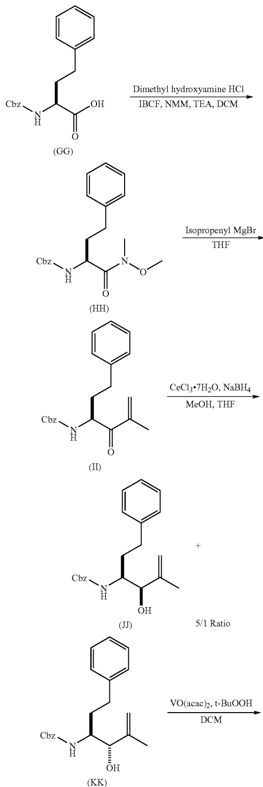
Scheme 8: Synthesis of Example 8
