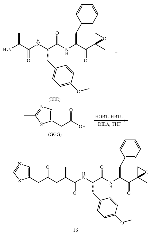
Scheme 16: Synthesis of Example 16
