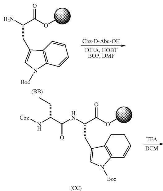
Scheme 5: Synthesis of Example 5
