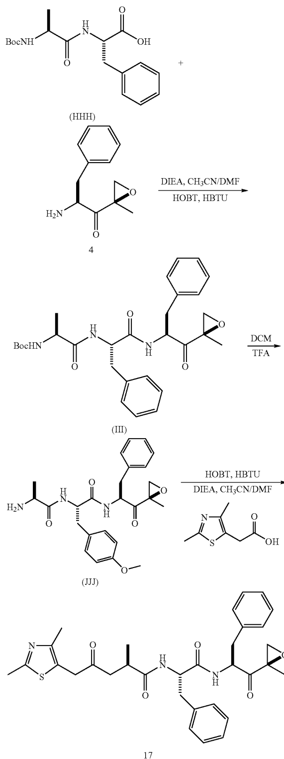
Scheme 17: Synthesis of Example 17
