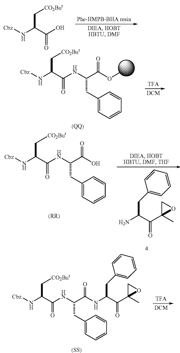
Scheme 10: Synthesis of Example 10
