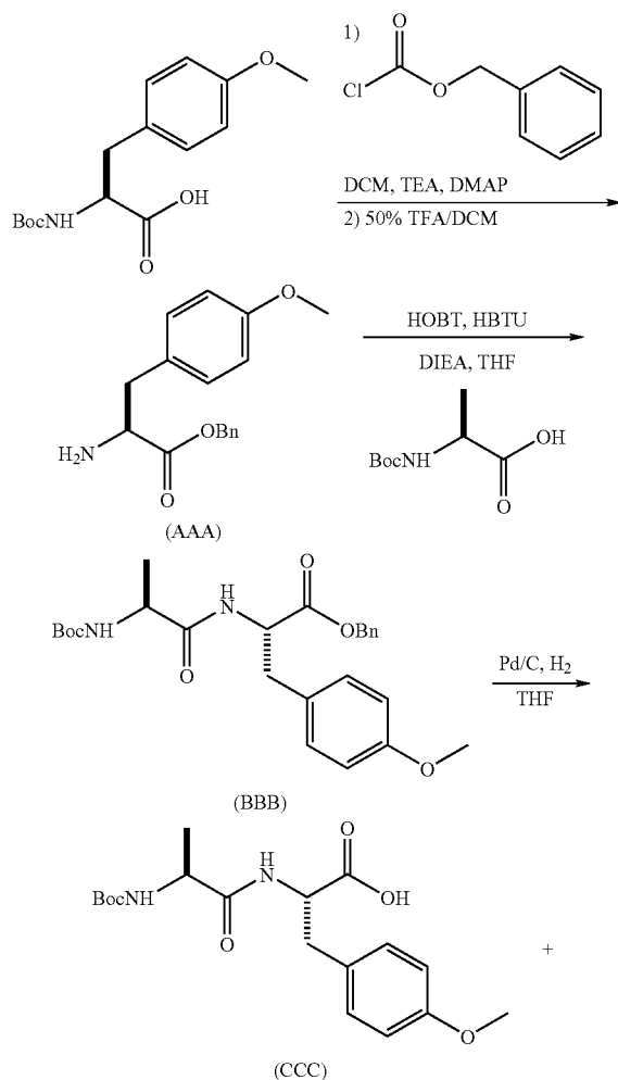
Scheme 14: Synthesis of Example 14
