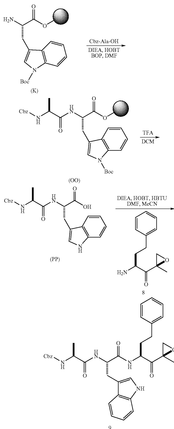
Scheme 9: Synthesis of Example 9
