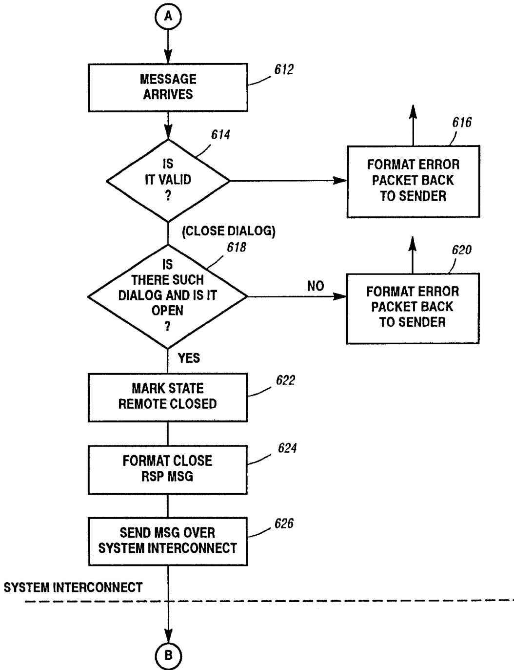
Dialog Termination (MSS) Figure 27(b)
