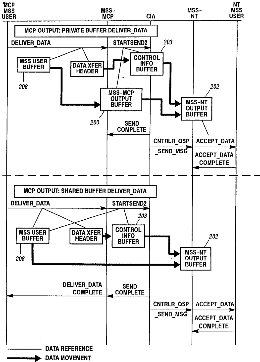
CIA-Based Output Data Transfer Flow Diagram
