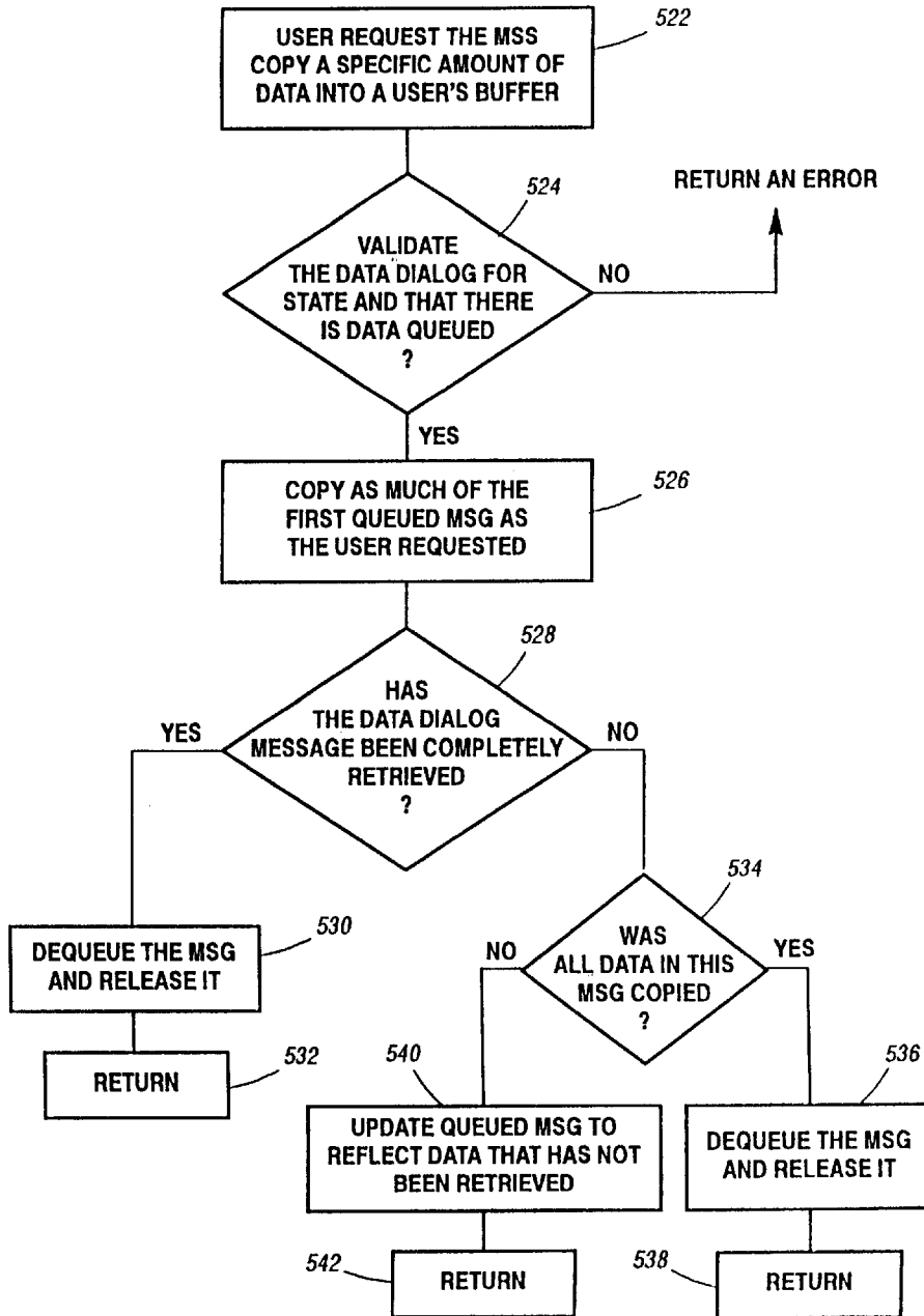
Input From MSS Figure 26(b)
