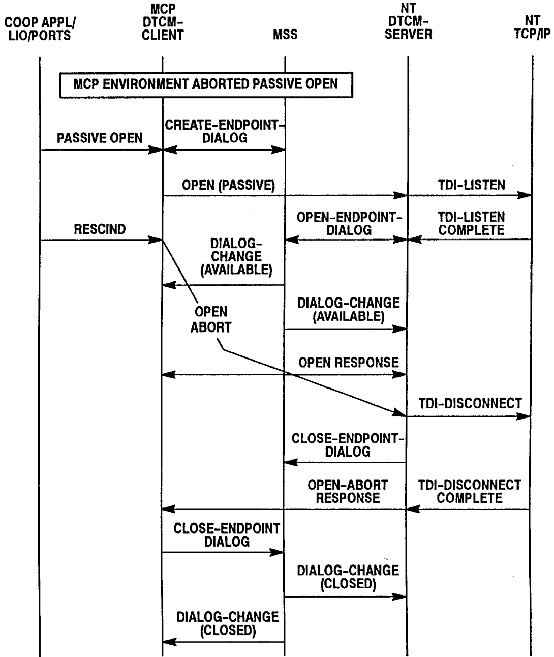
MCP Aborted Passive Open Figure 30
