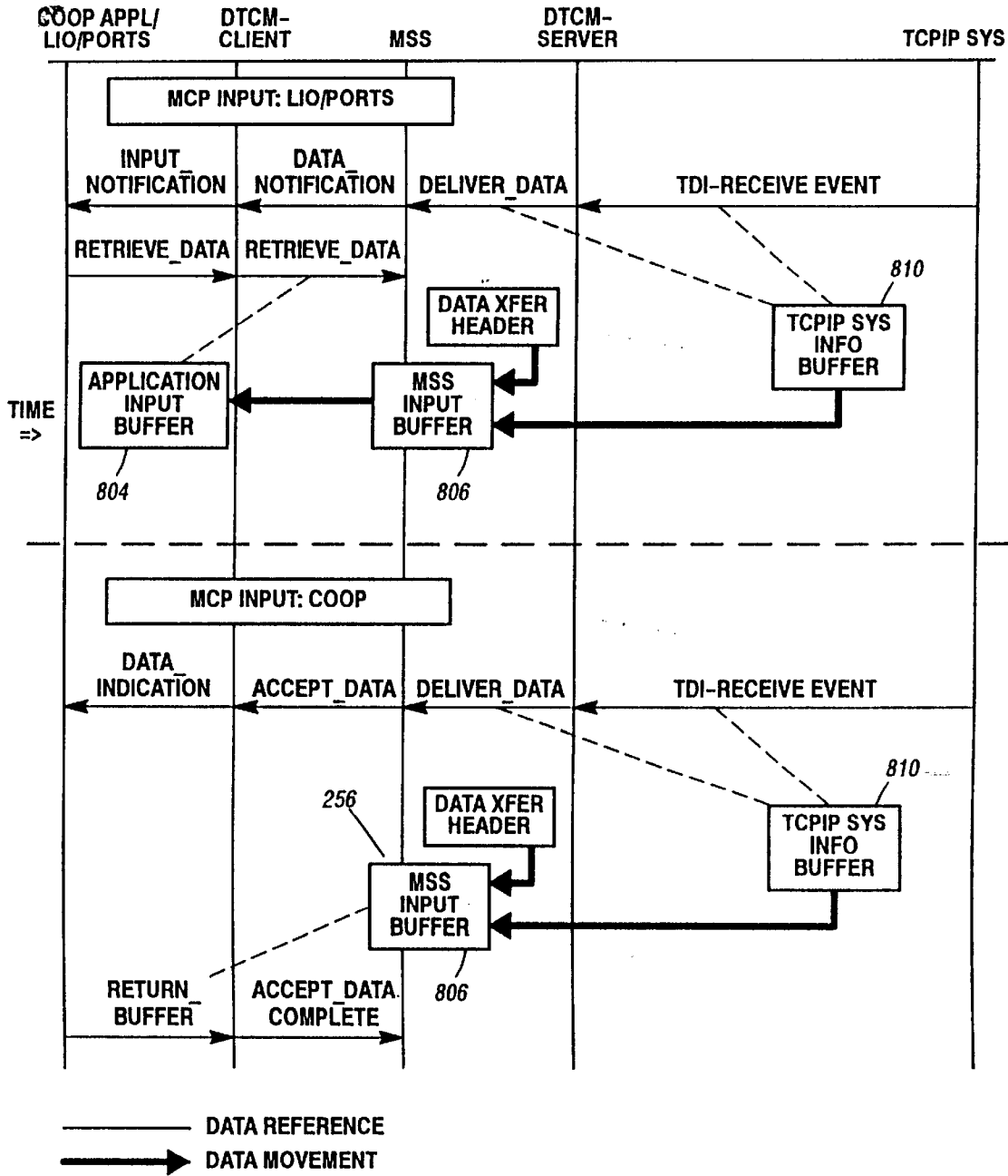
General Input Data Transfer Flow Diagram Figure 35
