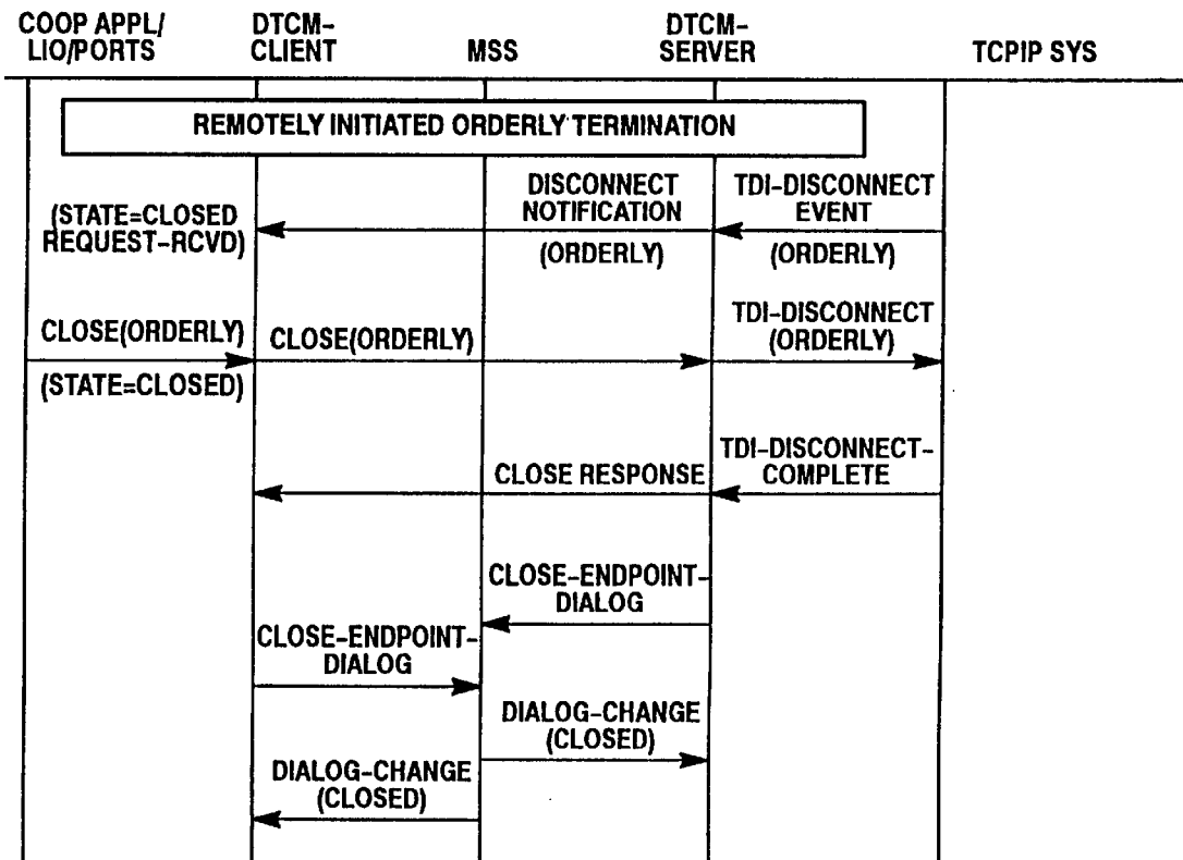
Remotely Initiated Orderly Dialog Termination Figure 37
