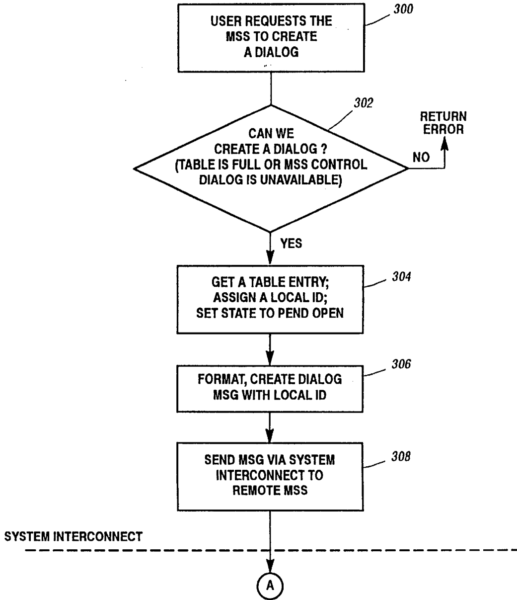
Dialog Establishment (MSS) Figure 24(a)
