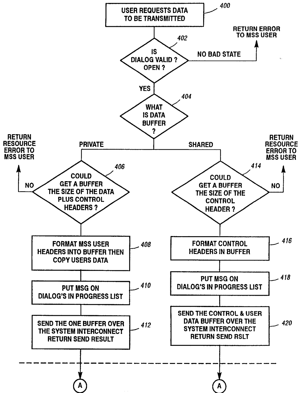
Output Over MSS Figure 25(a)
