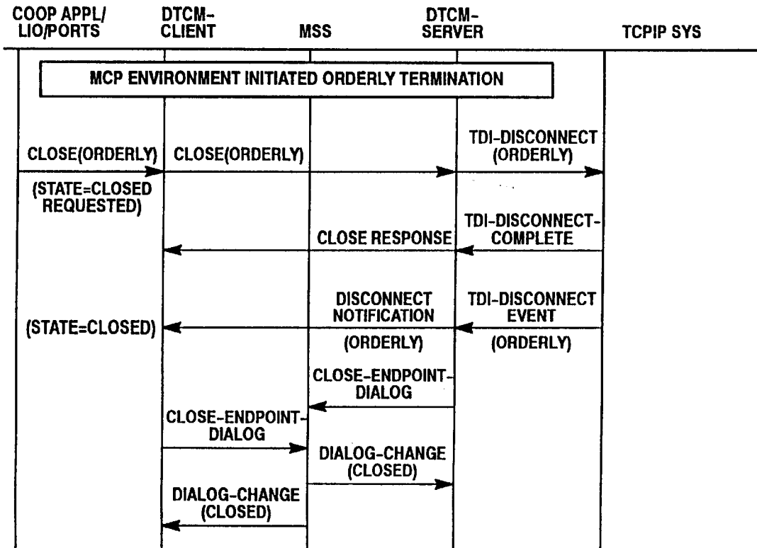
MCP Environment Initiated Orderly Dialog Termination Figure 36
