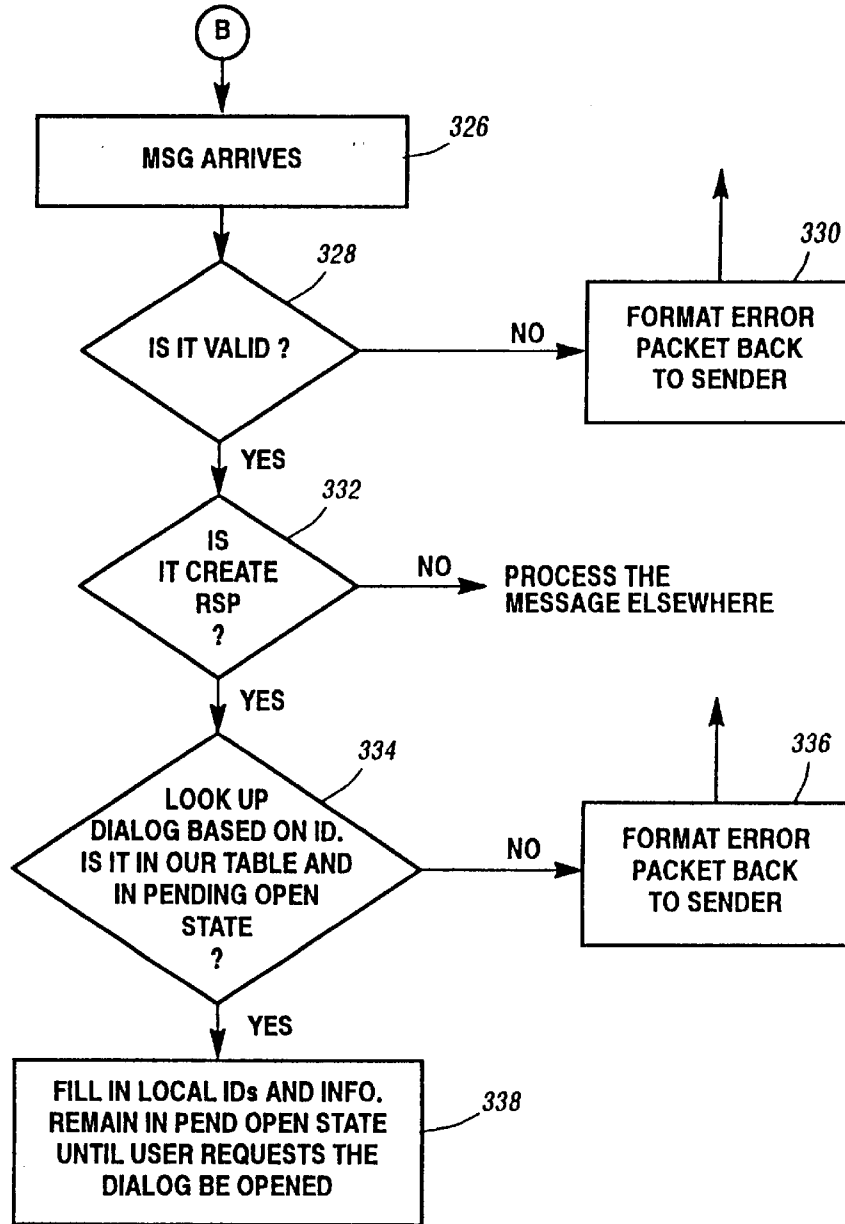
Dialog Establishment (MSS) Figure 24(c)
