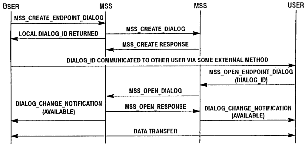
MSS Endpoint Dialog Creation Figure 21
