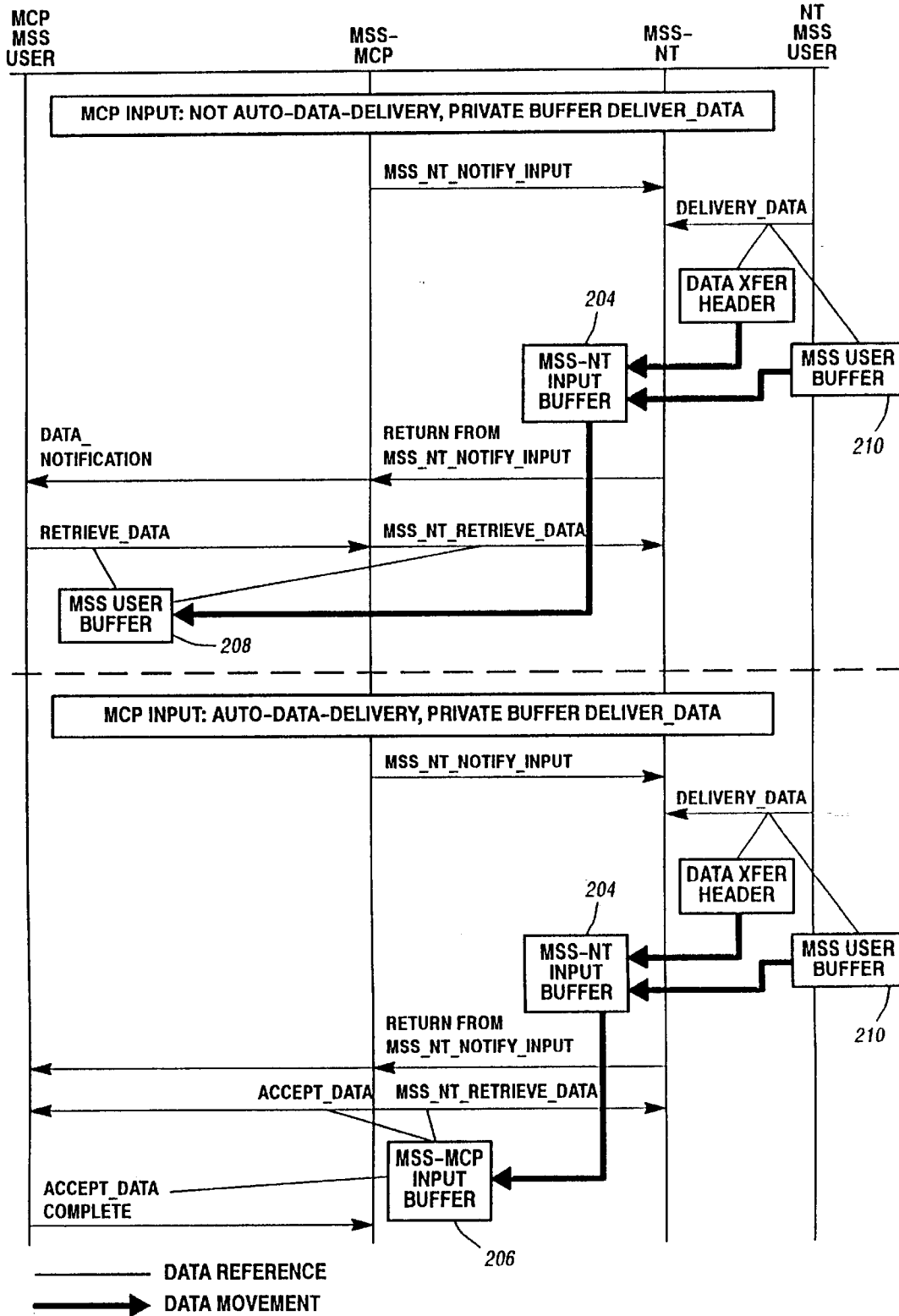
Emulation-Based Input Data Transfer Flow Diagram Figure 15
