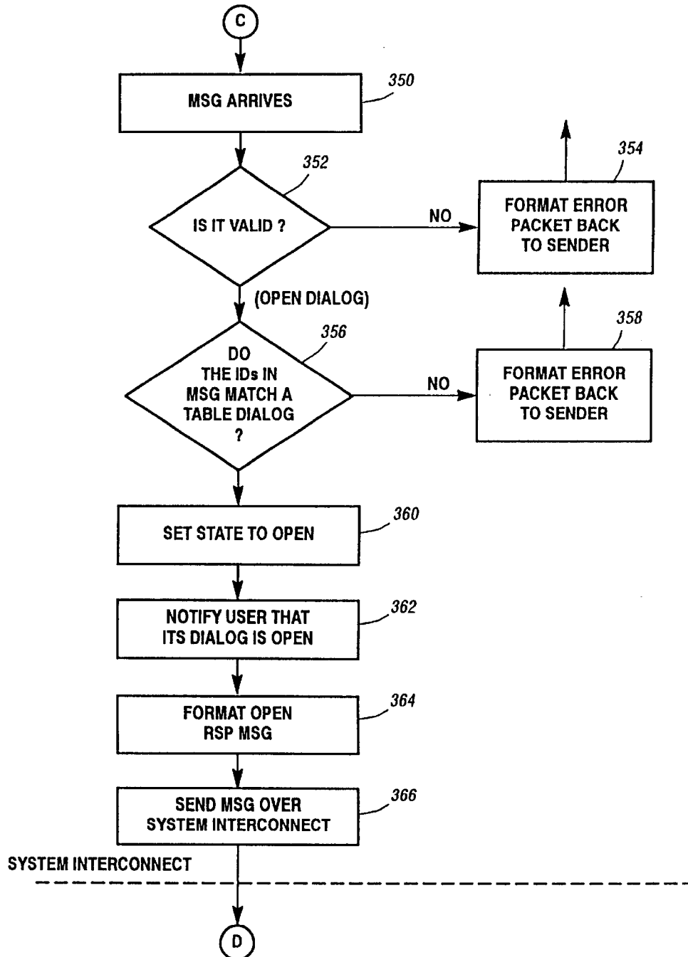
Dialog Establishment Figure 24(e)
