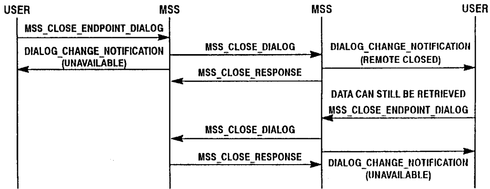
MSS Endpoint Dialog Termination (Normal Close) Figure 22
