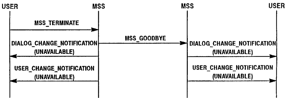
MSS Termination Figure 19
