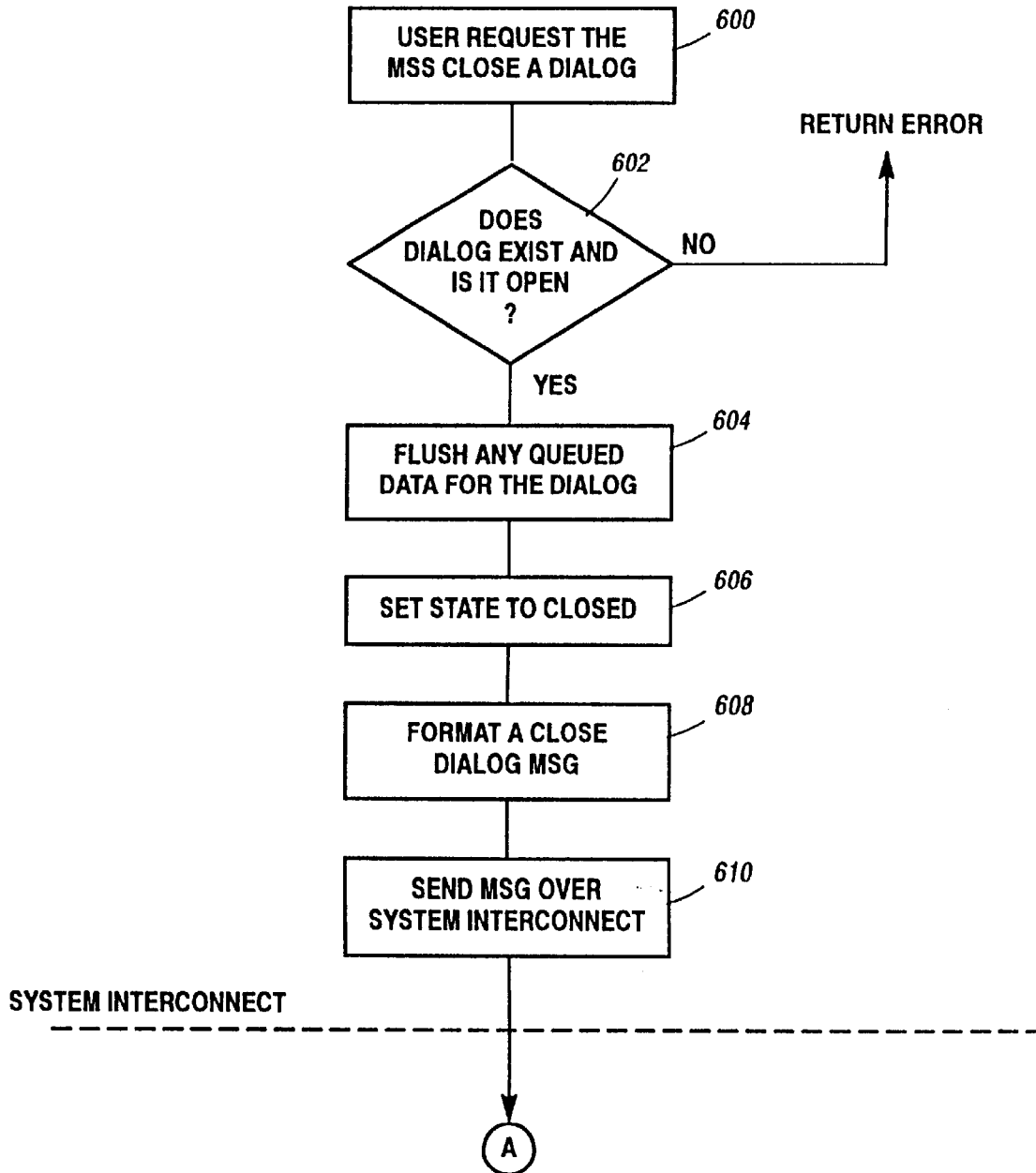
Dialog Termination (MSS) Figure 27(a)
