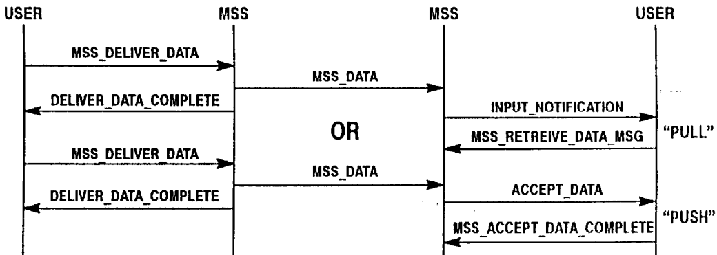
MSS Termination Figure 19
