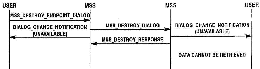
MSS Endpoint Dialog Termination (Destroy) Figure 23
