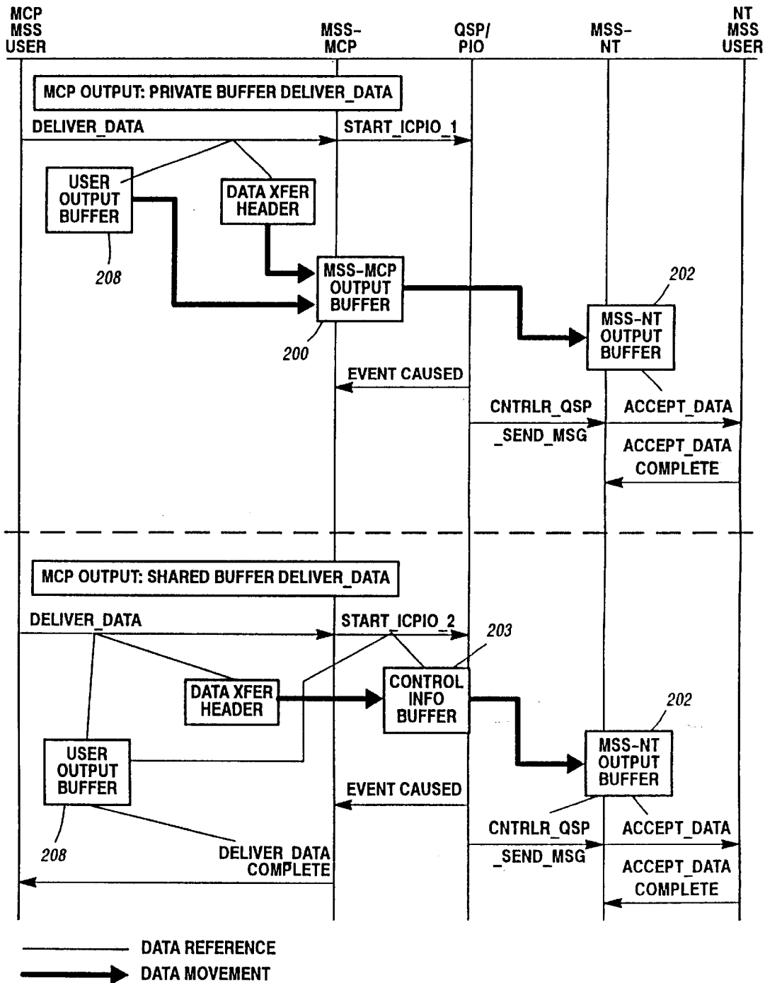
QSP-Based Output Data Transfer Flow Diagram
