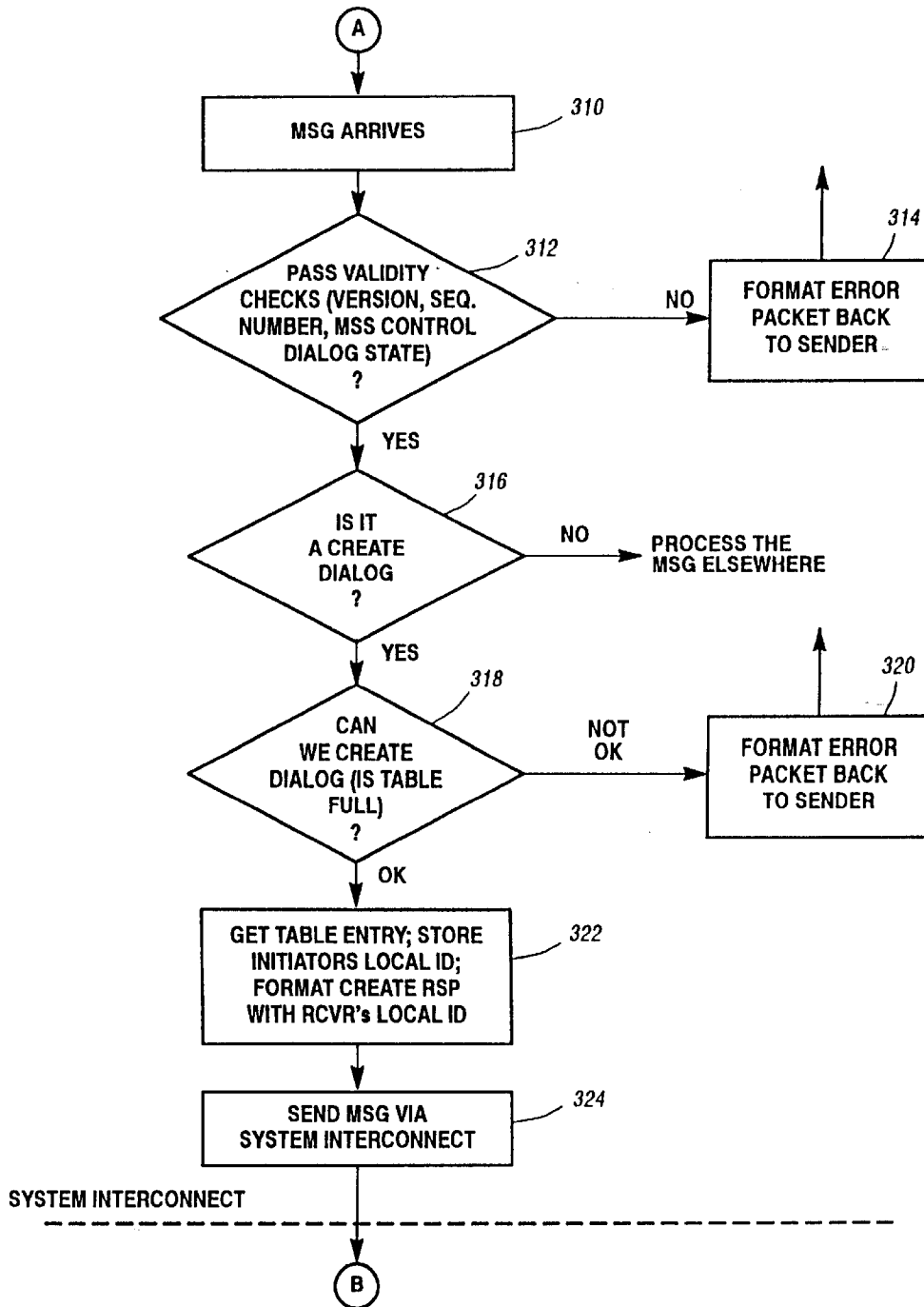
Dialog Establishment (MSS) Figure 24(b)
