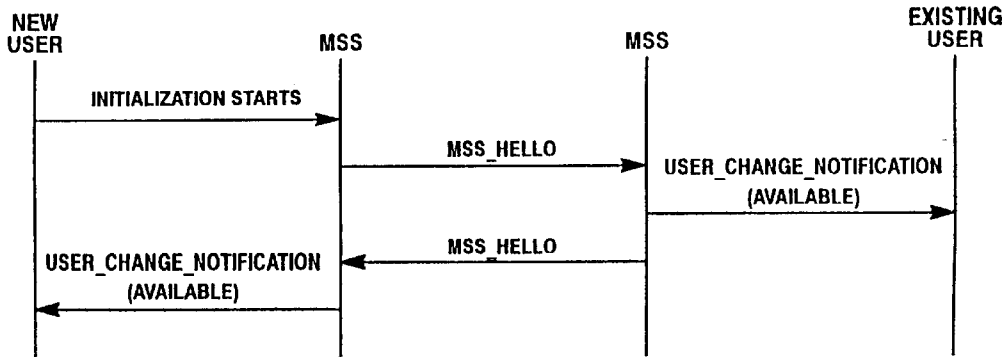
MSS Initialization / Greeting Figure 18
