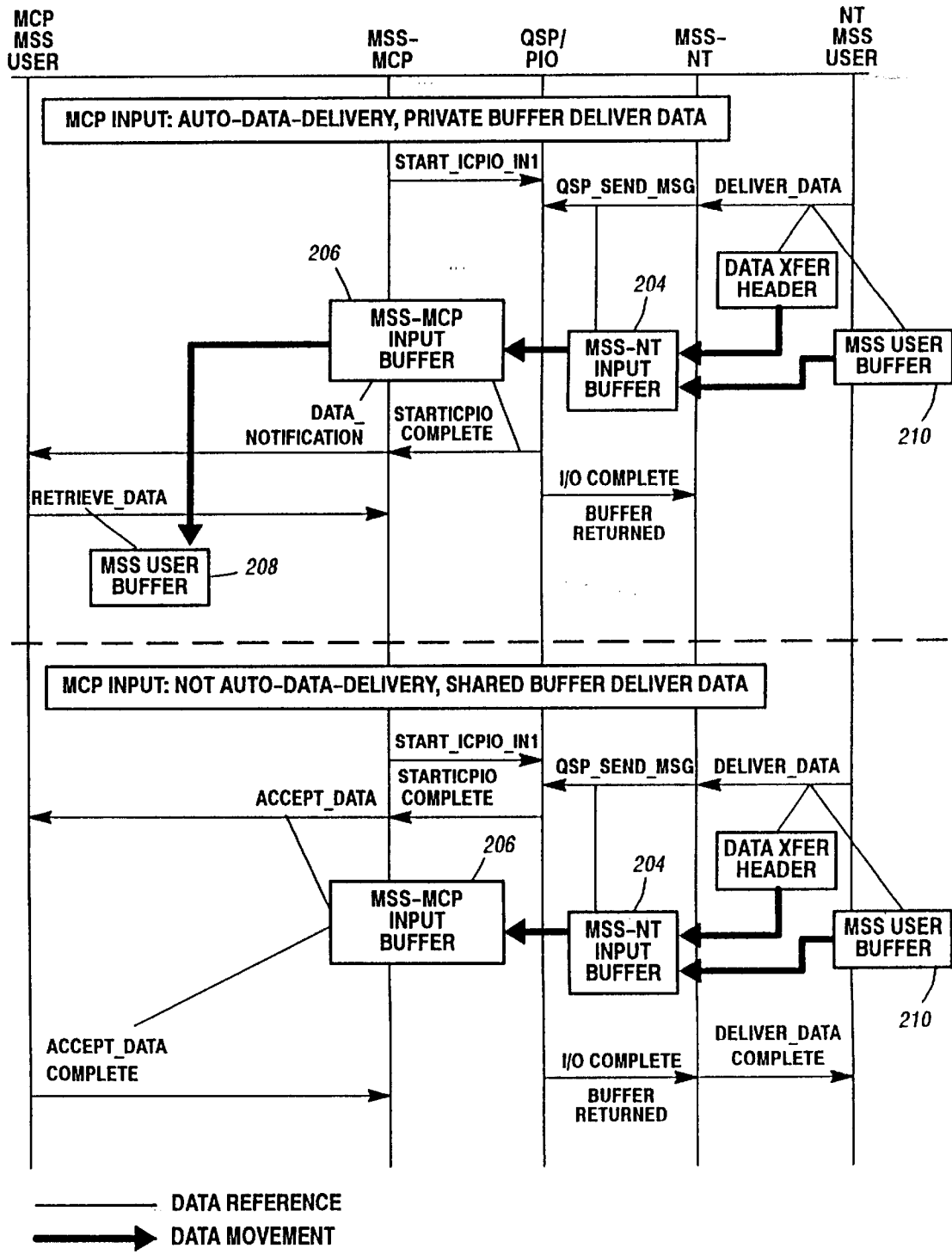
QSP-Based Input Data Transfer Flow Diagram Figure 13
