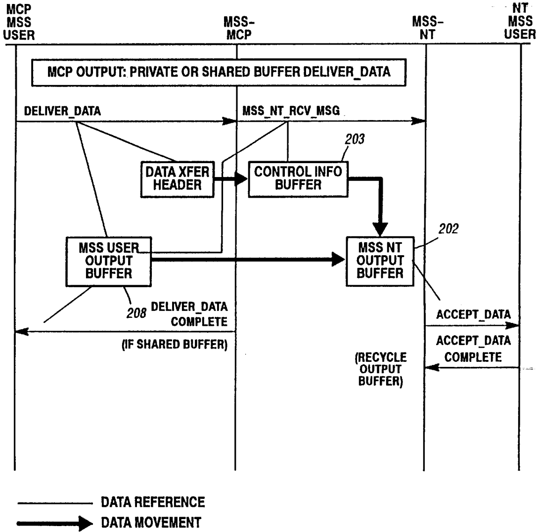
Emulation-Based Output Data Transfer Flow Diagram Figure 14
