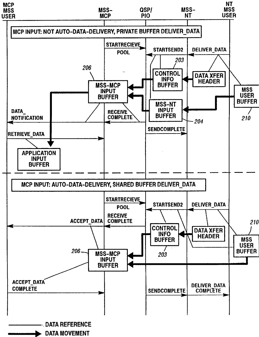
CIA-Based Input Data Transfer Flow Diagram Figure 17
