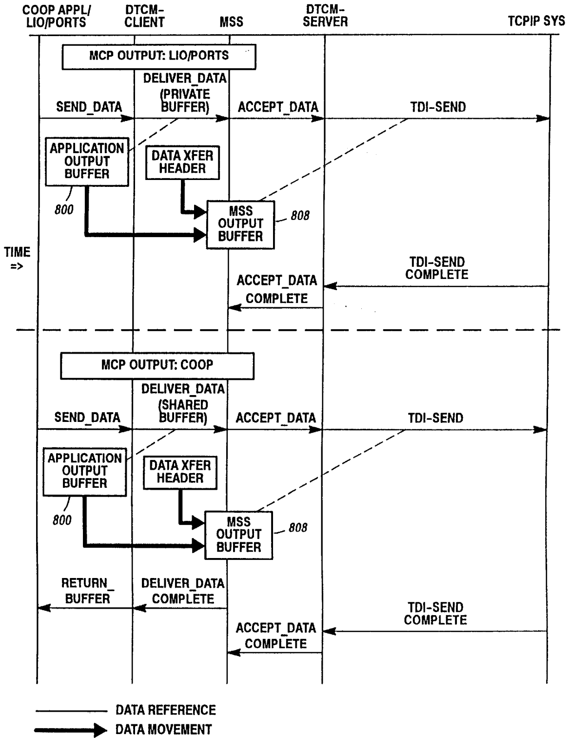
General Output Data Transfer Flow Diagram Figure 34
