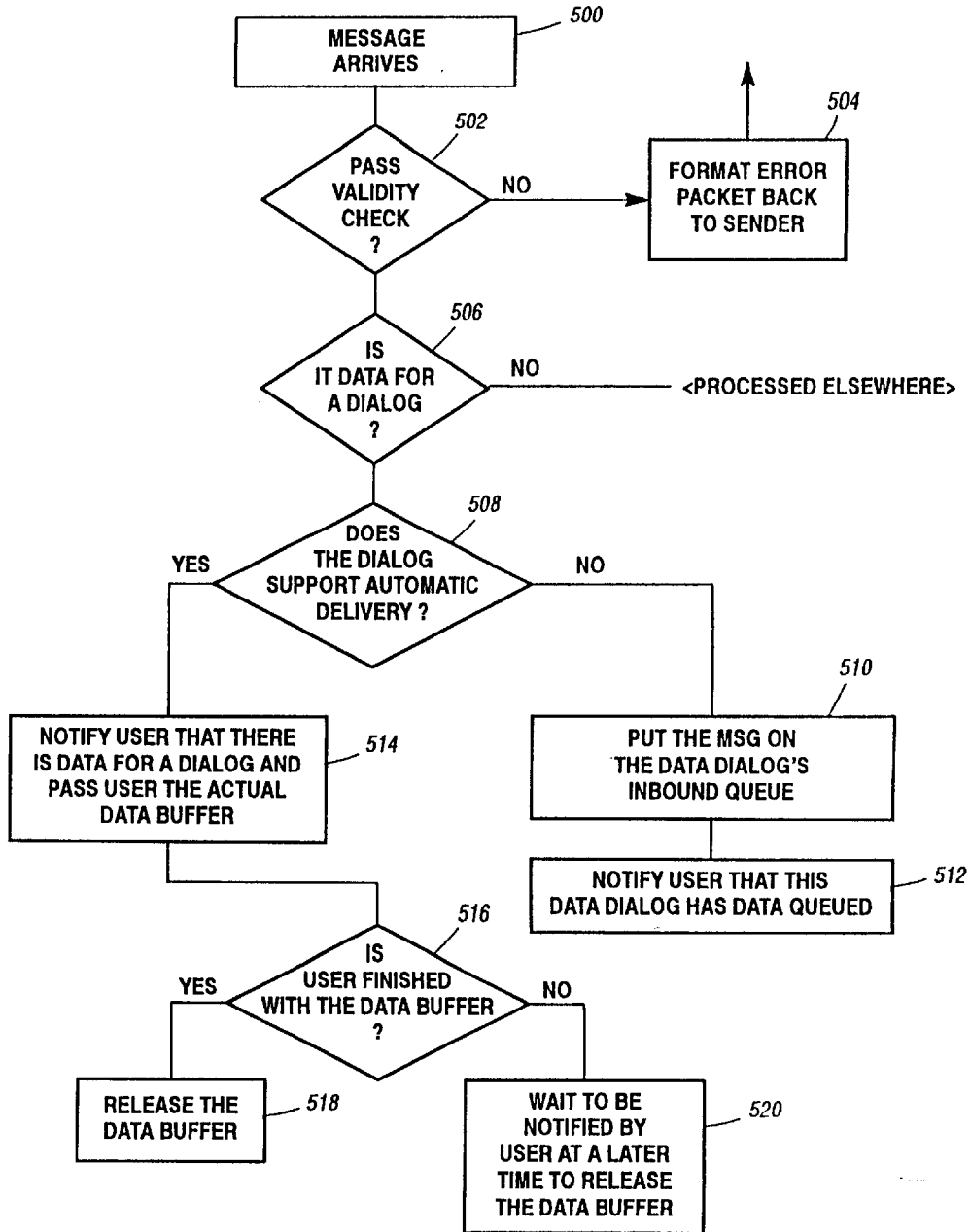
Input From MSS Figure 26(a)
