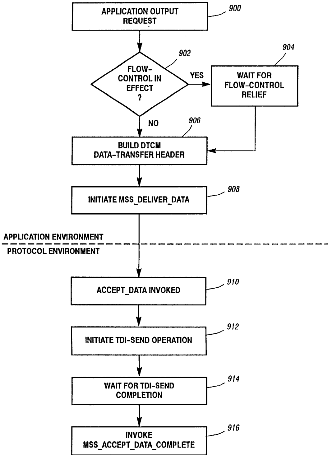
DTCM-Client Output Figure 33
