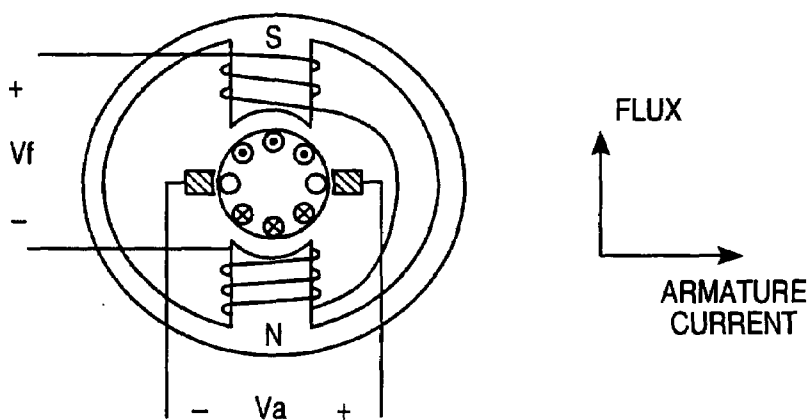
FIG. 4 (PRIOR ART)
