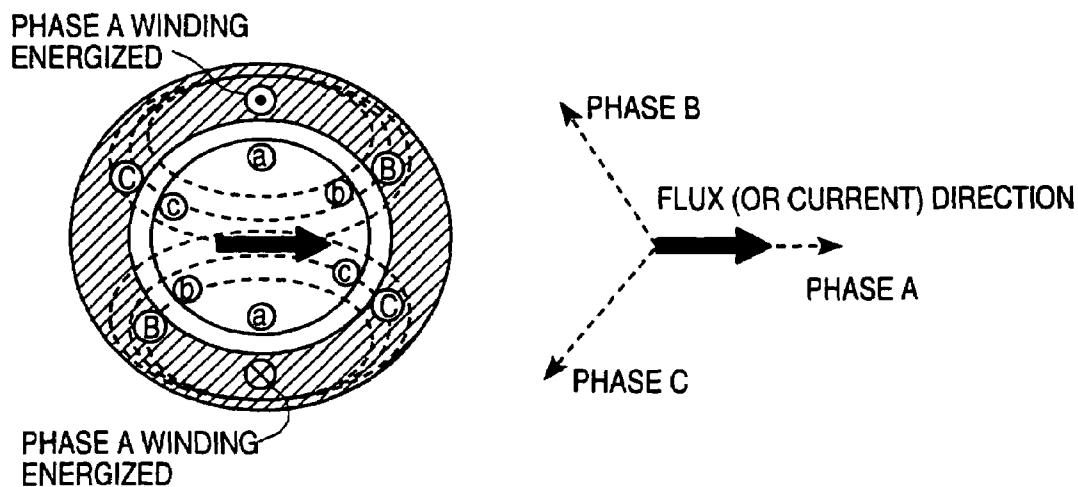
FIG. 5 (PRIOR ART)
