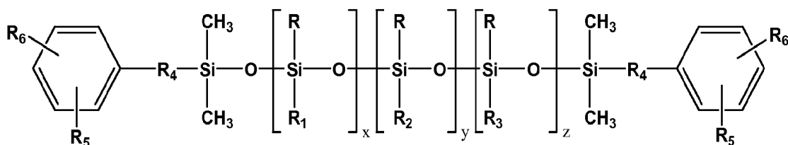
(Formula I)
