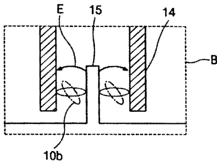
(prior art) FIG. 9B
