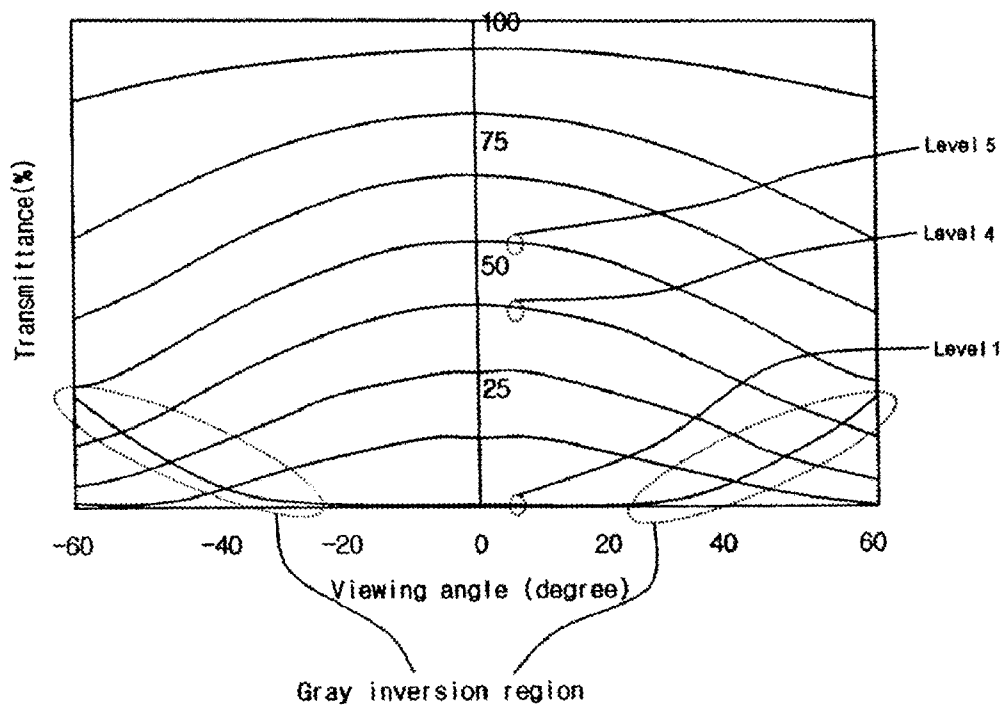
(prior art) FIG. 7
