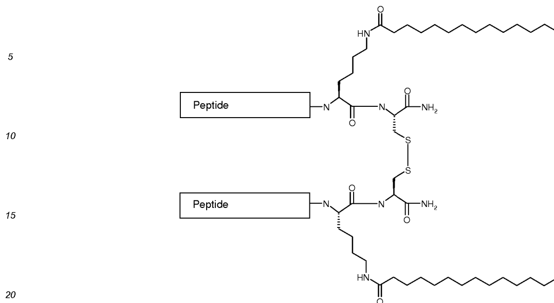
Disulfide dimer
