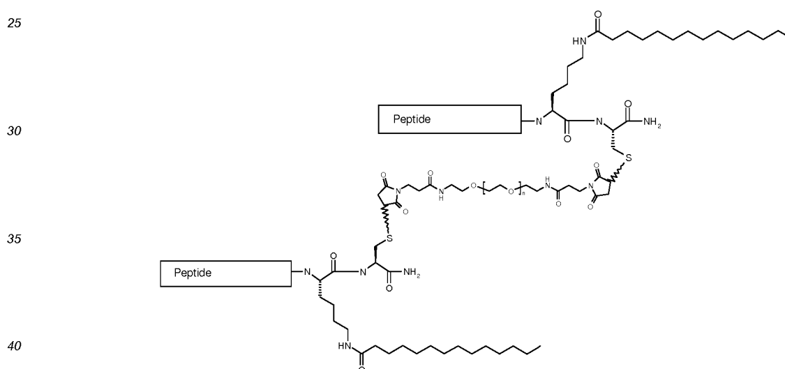
Structure B
