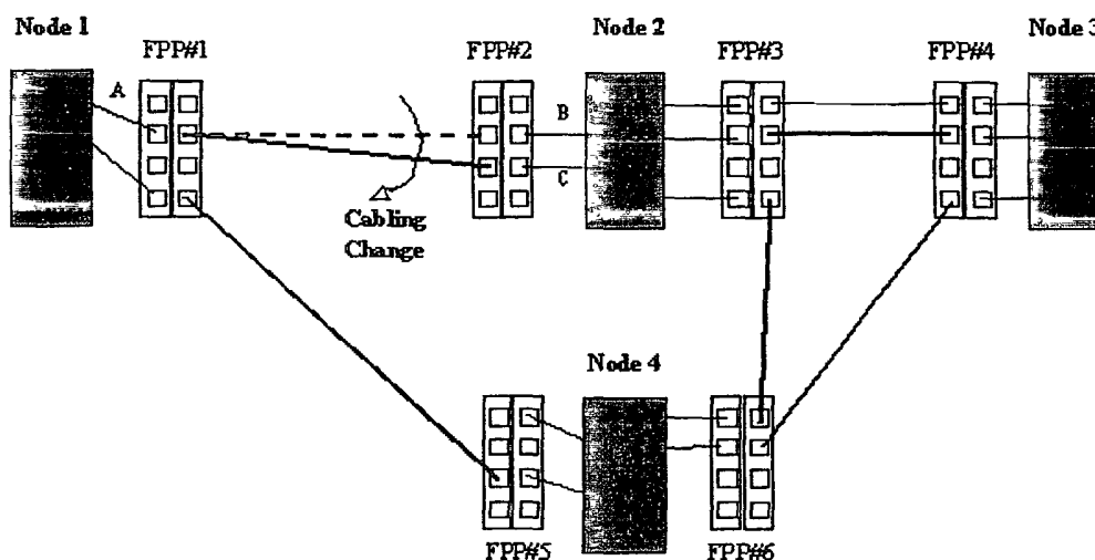
Simple Fiber Cable Change Example
