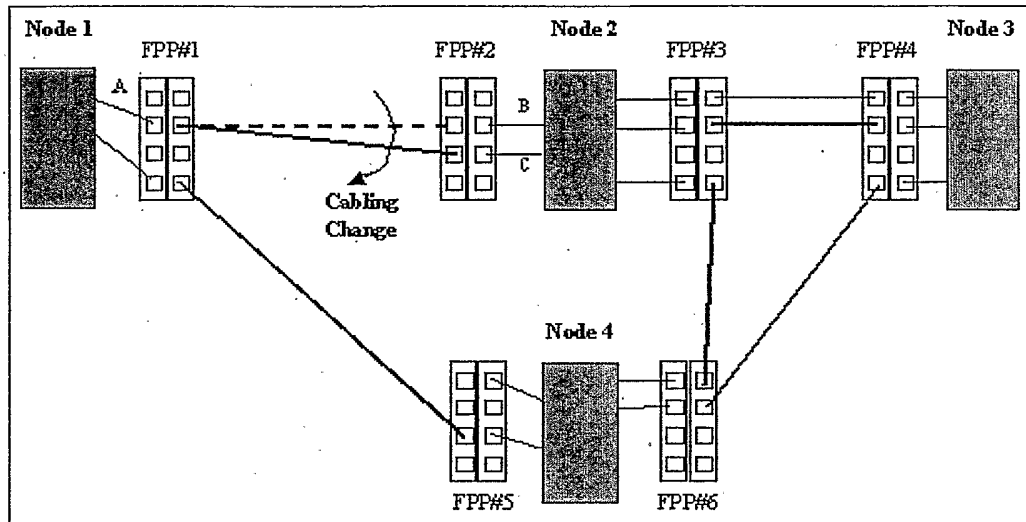
Figure#1 – Simple Fiber Cable Change Example
