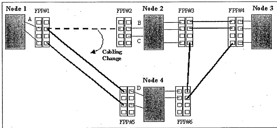
Figure #3 – Complex Fiber Cable Change Example
