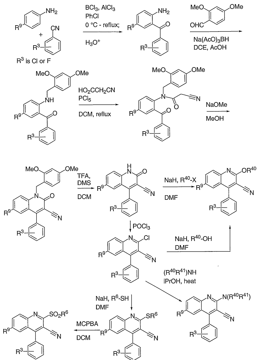
Scheme 1
