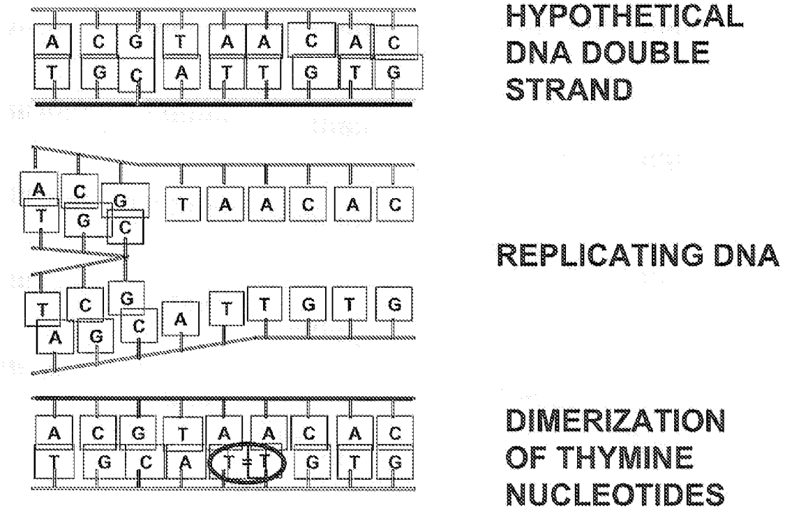
Figure 1: Dimer Formation by UV Photon (by permission of ERG @ UNH)
