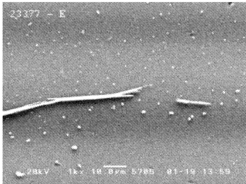
Figure 2: Bacillus atrophaeus after FUV photon impact
