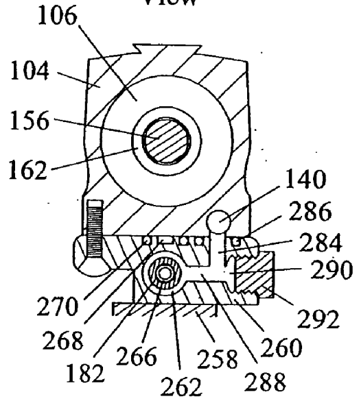
Rear Sectional View
