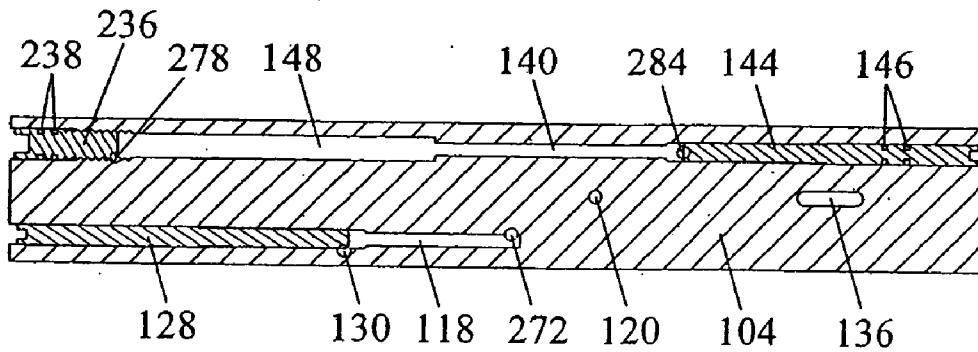
Top Sectional View
