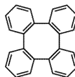
(aa) Tetraphenylene
