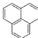
(al) Phenalene
