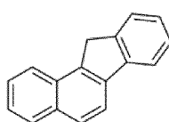
(ac) Benzo(a)fluorene
