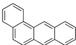
(ab) Benz(a)anthracene
