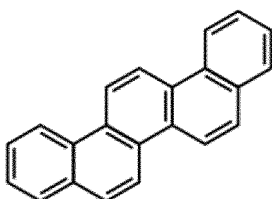
(z) Picene
