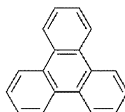
(al) Phenalene
