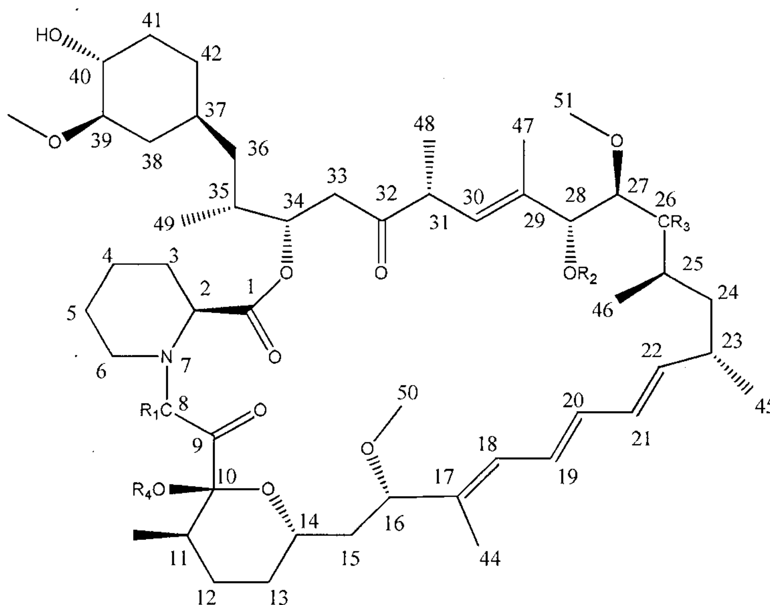
Formula II
