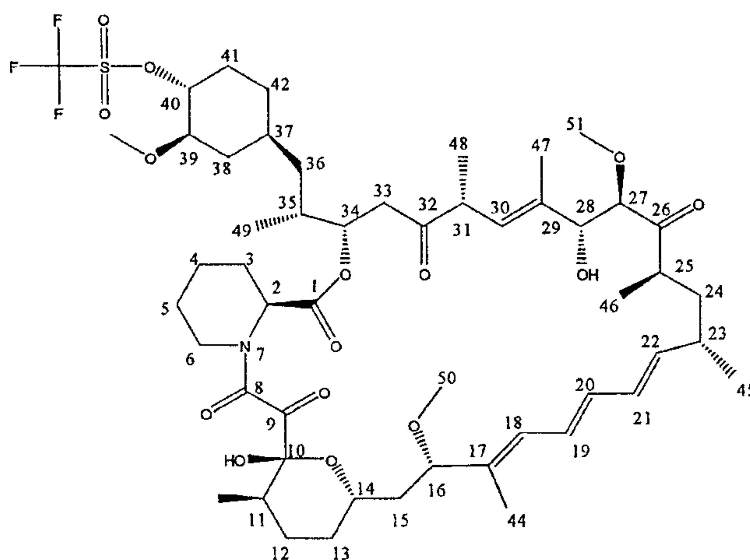
Formula VII
