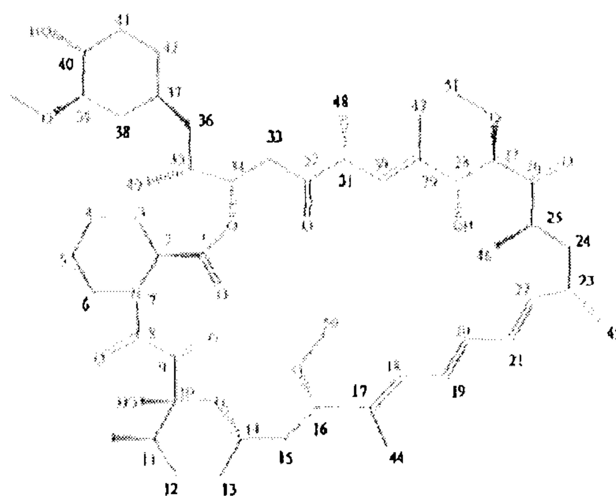
Formula VI
