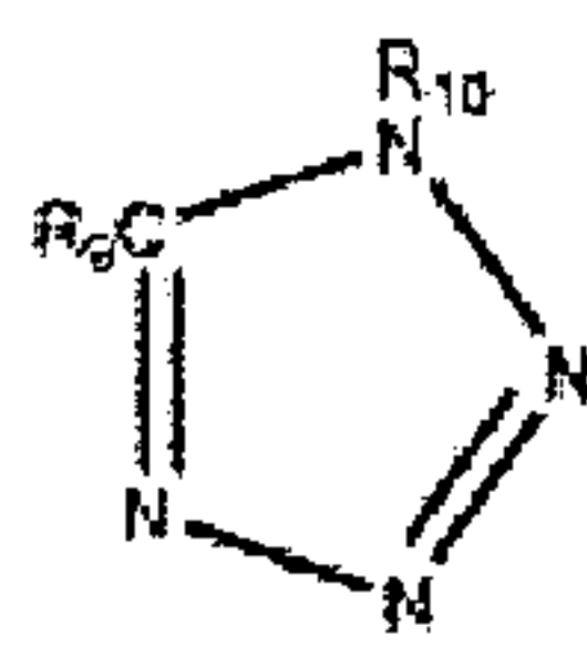
Formula IV
