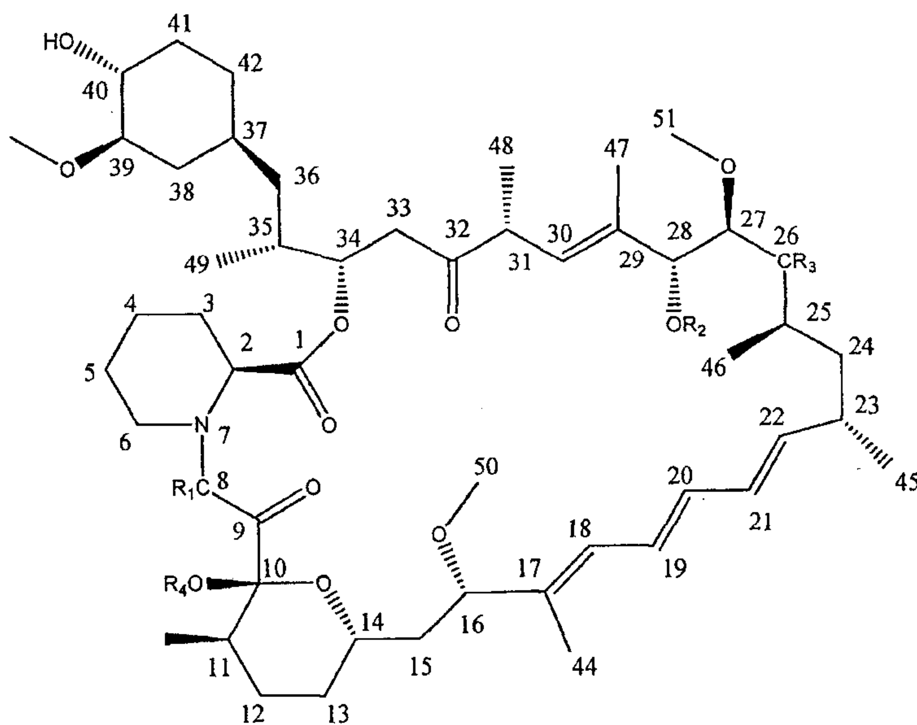
Formula II
