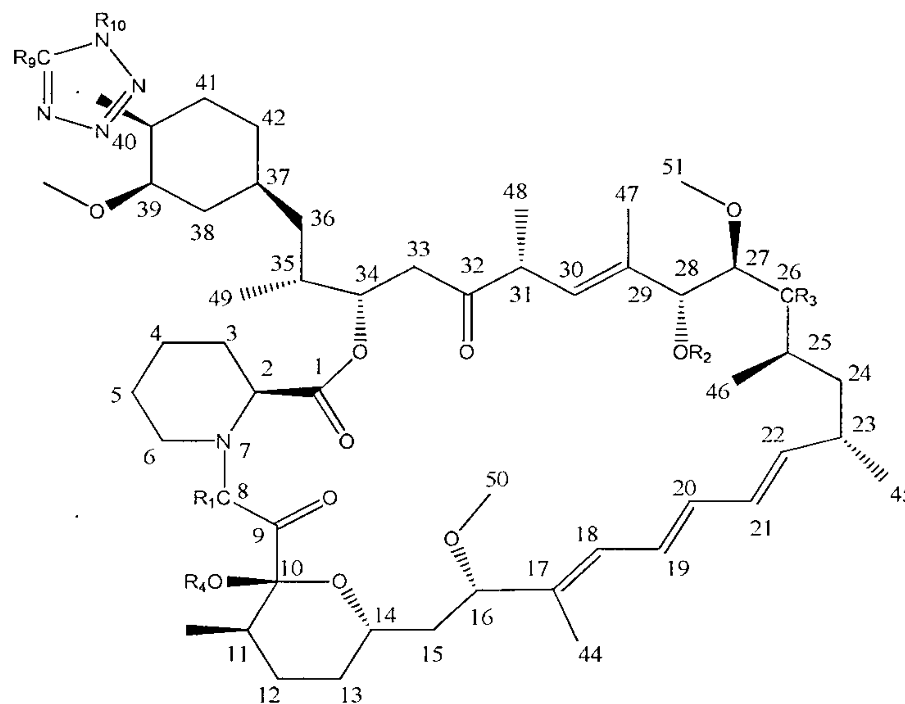
Formula I
