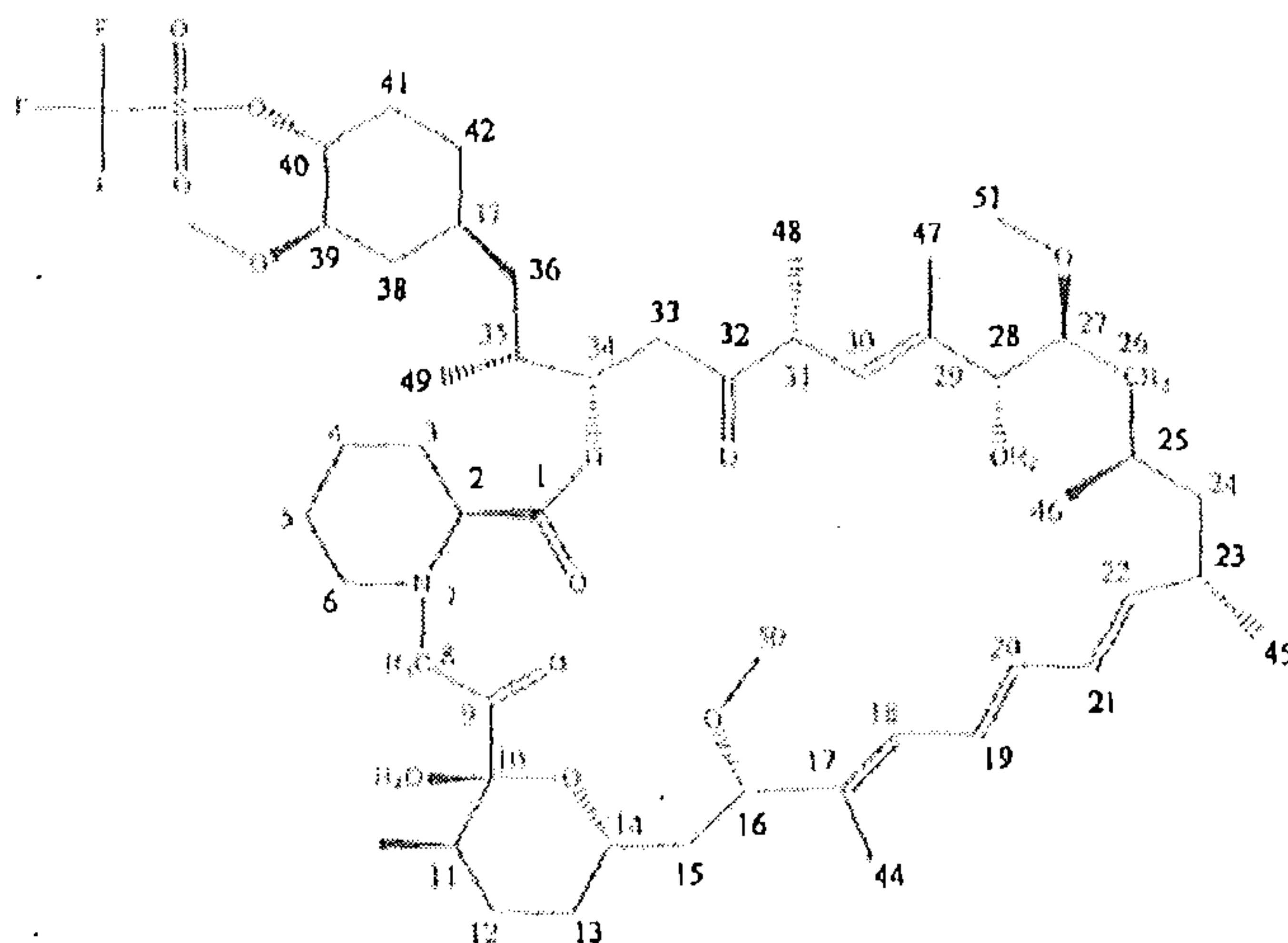
Formula III
