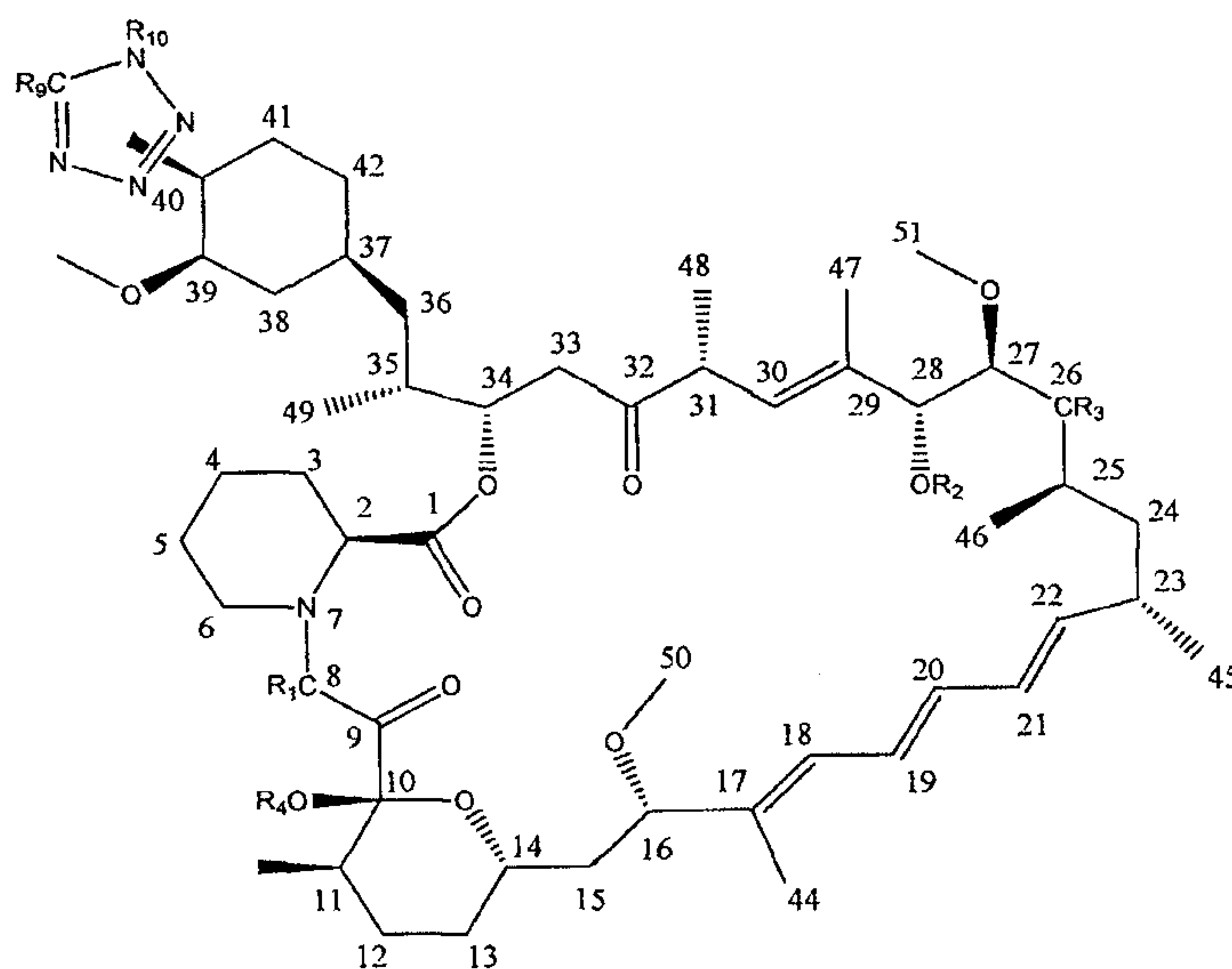
Formula I
