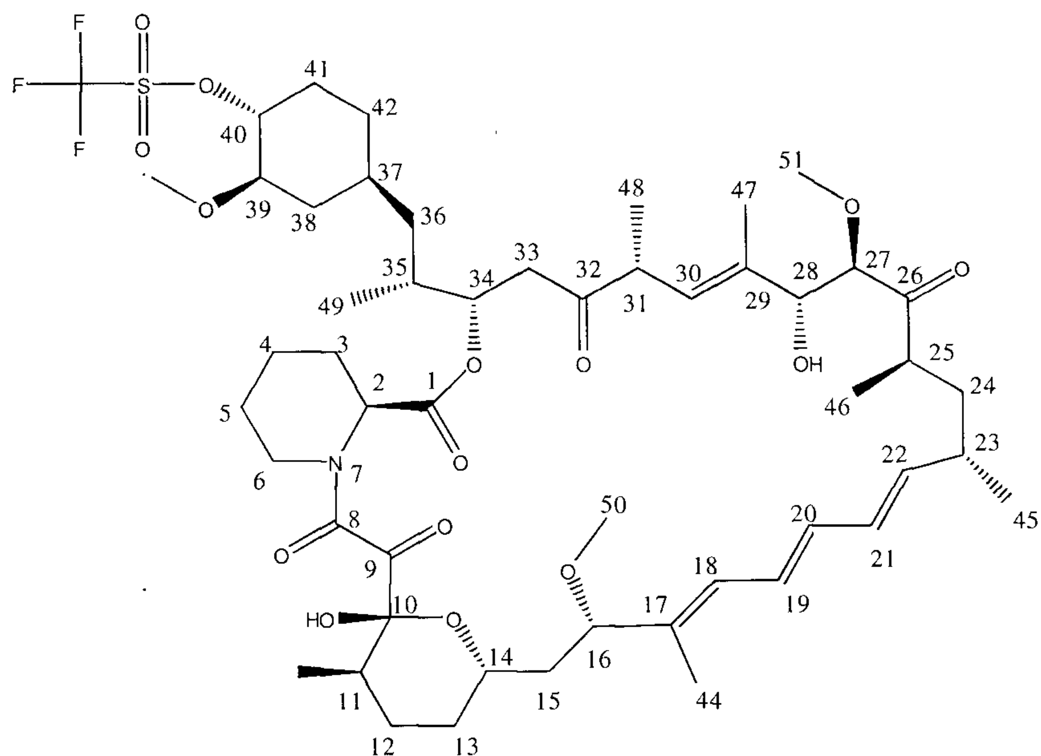
Formula VII
