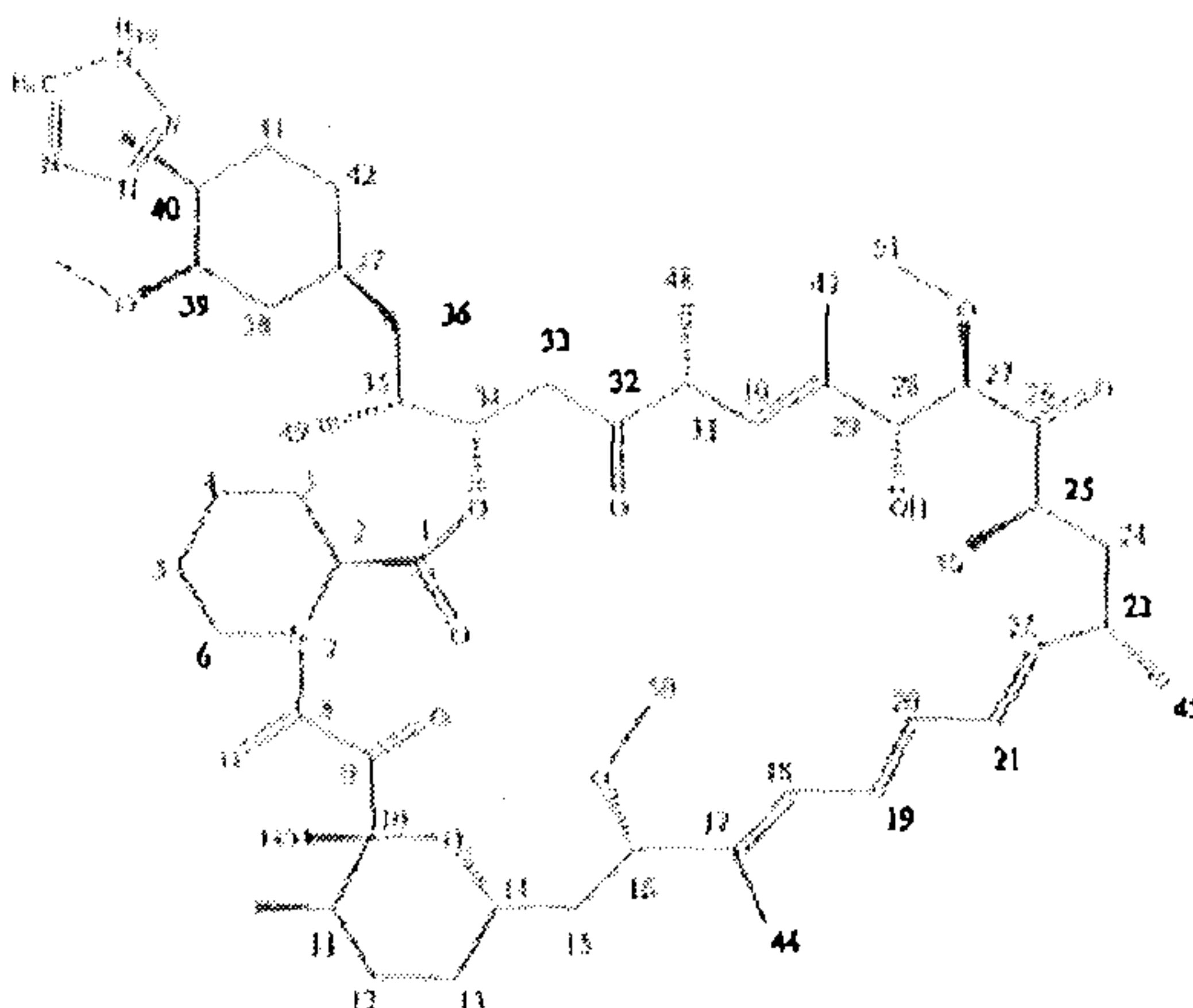
Formula V
