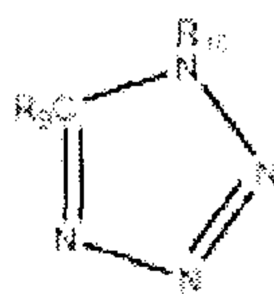
Formula IV
