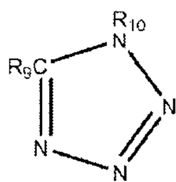
Formula IV
