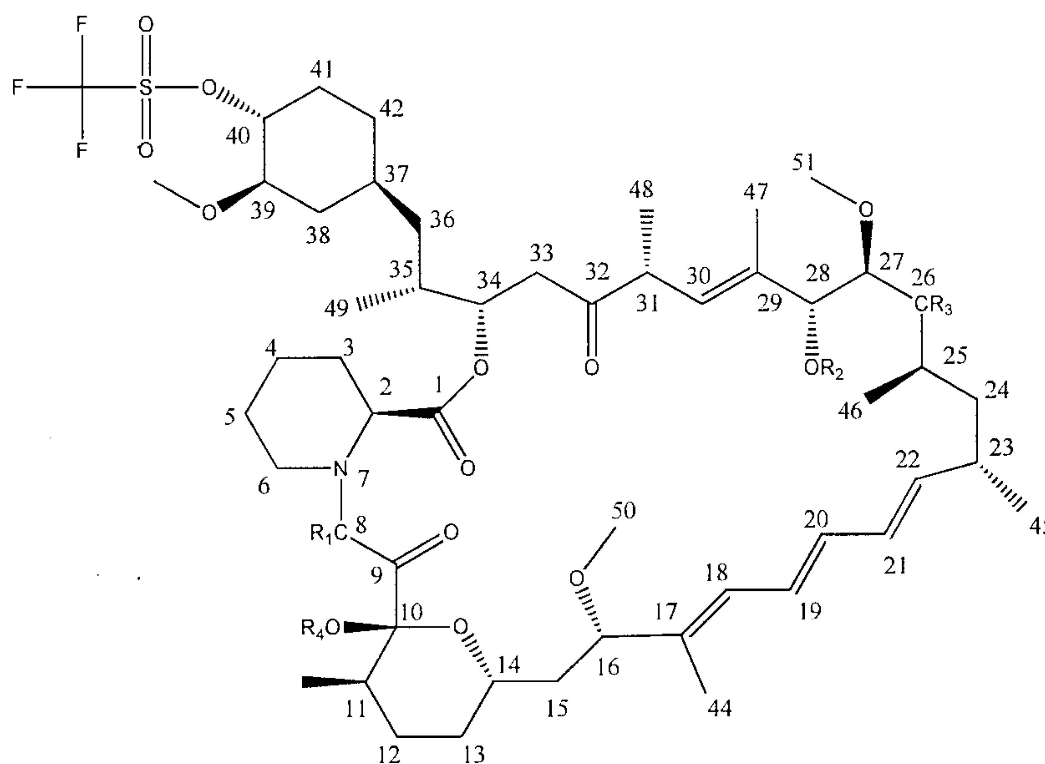
Formula III
