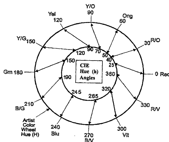
Artists' Color Wheel vs. CIE Hue Angle
