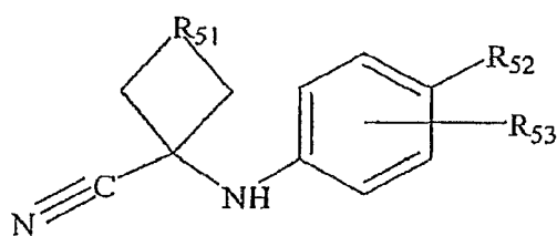
Compound II
