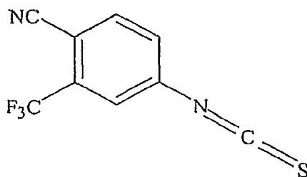
Compound I
