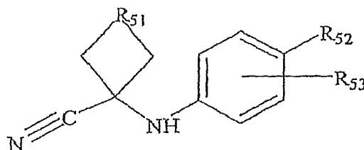
Compound II
