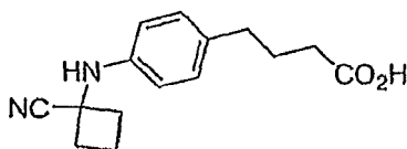
Formula 50
