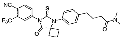
NC56 Formula 49
