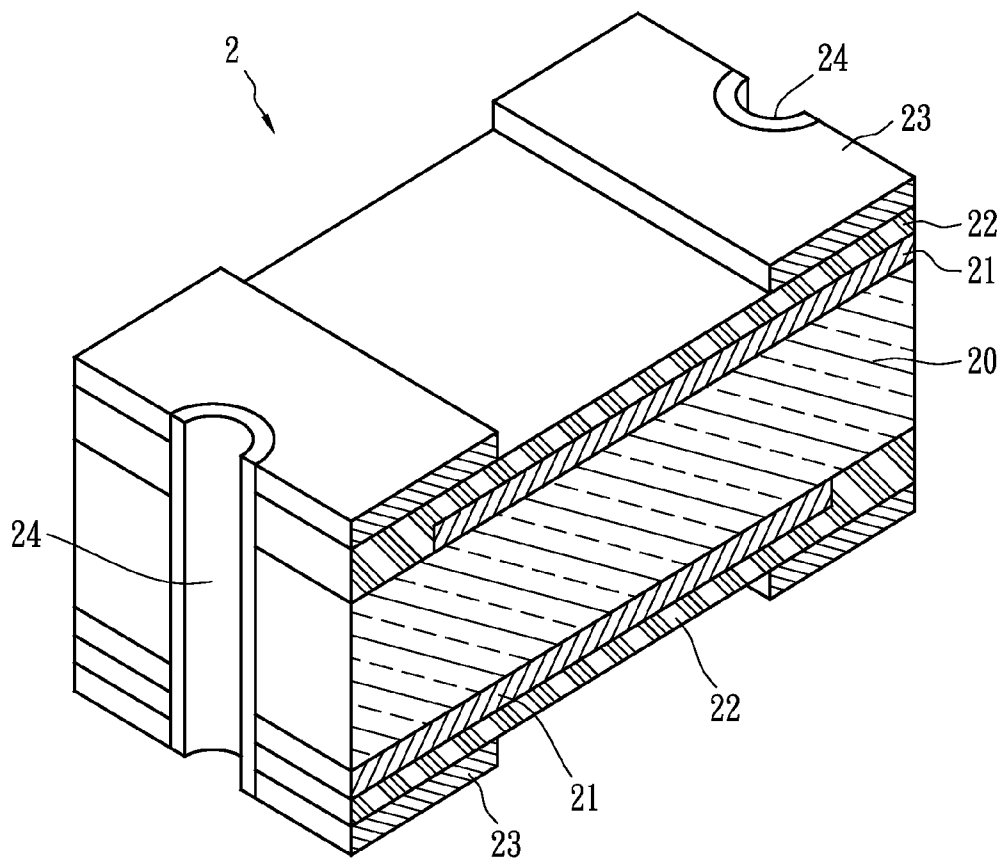
FIG. 2 (Prior Art)
