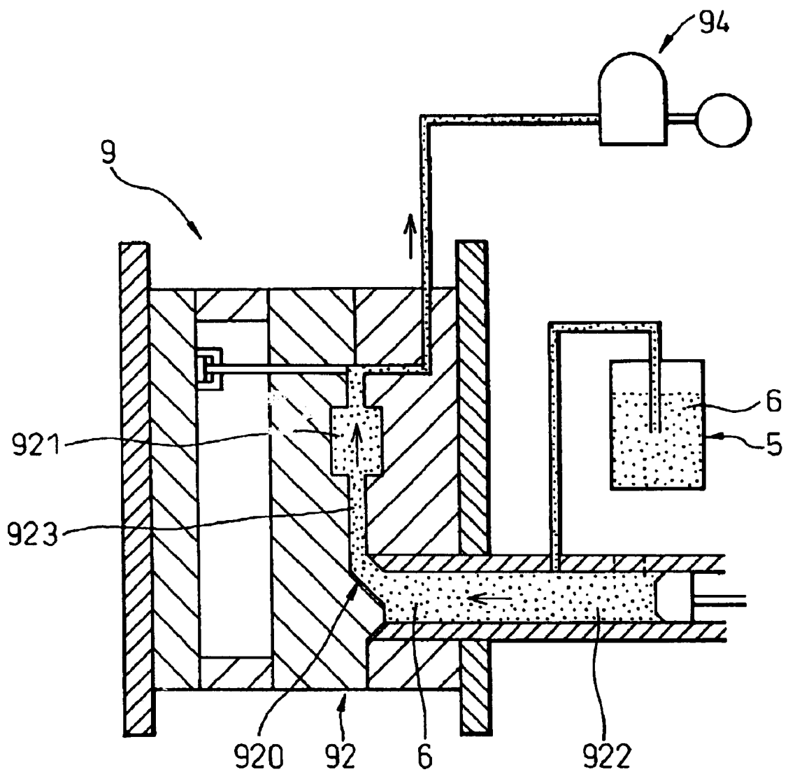
Fig.14 PRIOR ART
