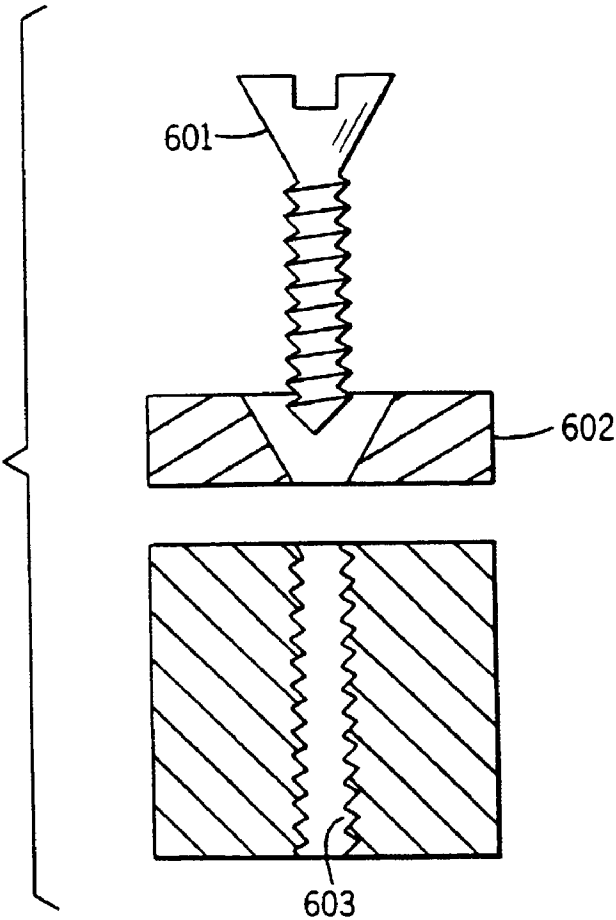
FIG. 27a PRIOR ART
