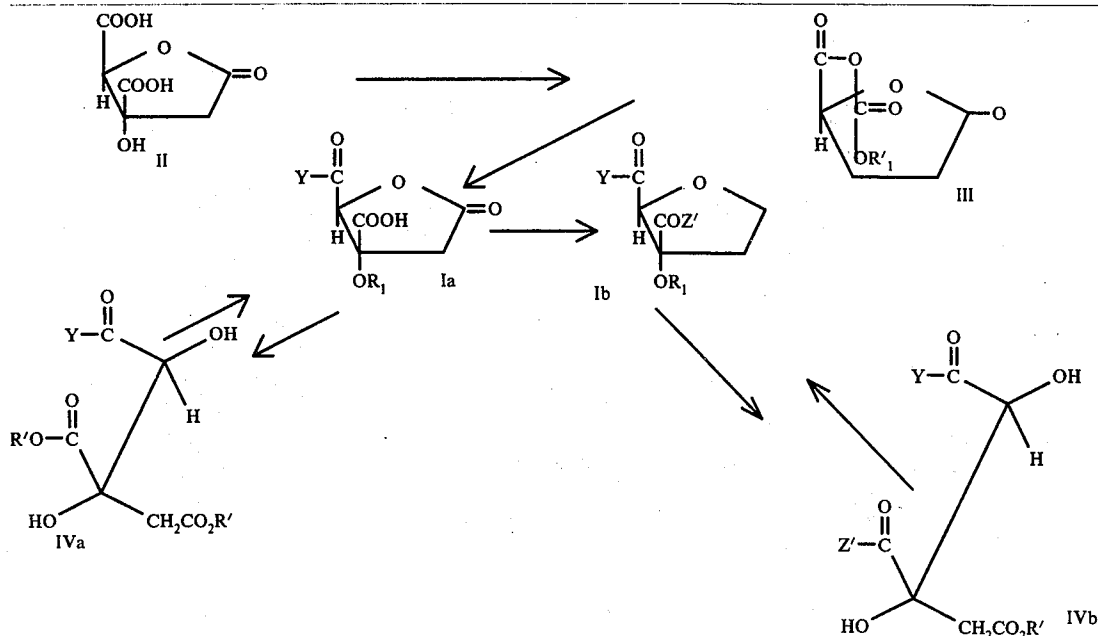
REACTION SCHEME A
