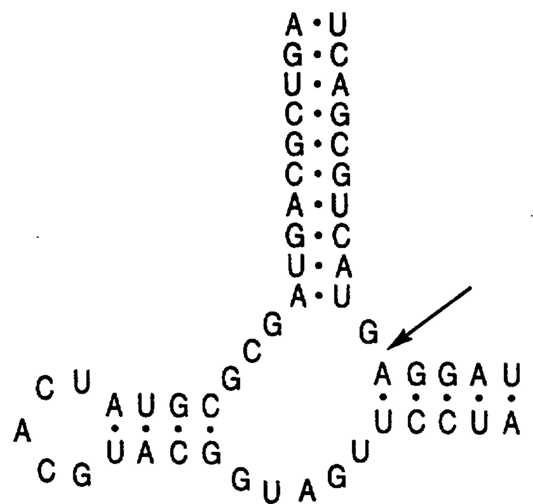
G-CLEAVING RIBOZYME-B
