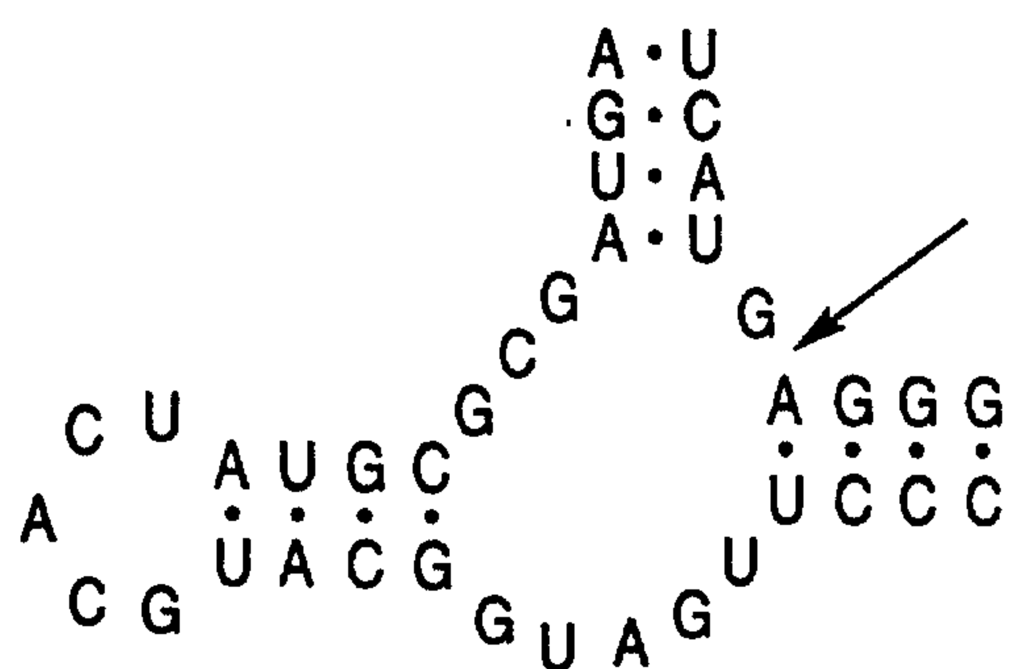
G-CLEAVING RIBOZYME-C
