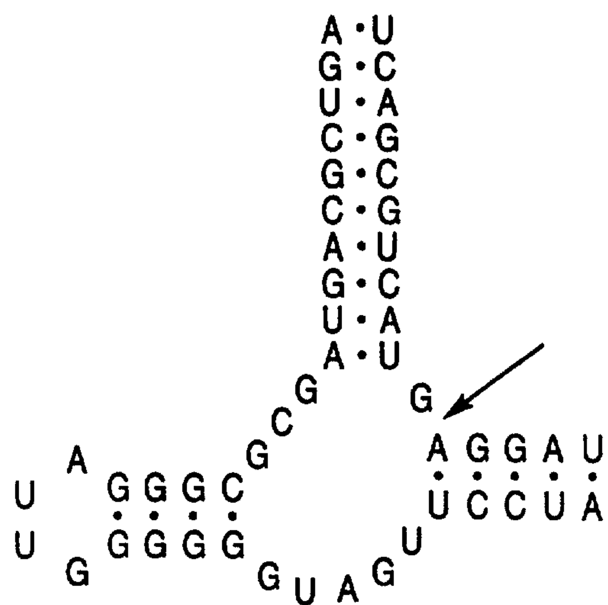
G-CLEAVING RIBOZYME-A
