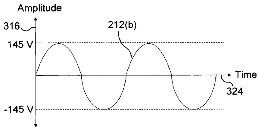
Fig. 8A RF Signal X
