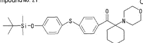
Compound No. 21
