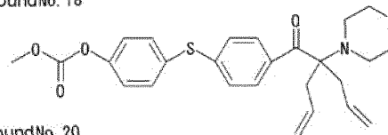
Compound No. 20
