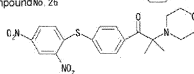
Compound No. 26
