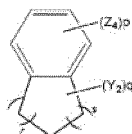
Chemical Formula 14
