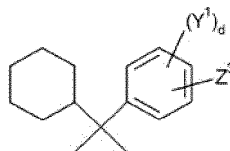
Chemical Formula 12
