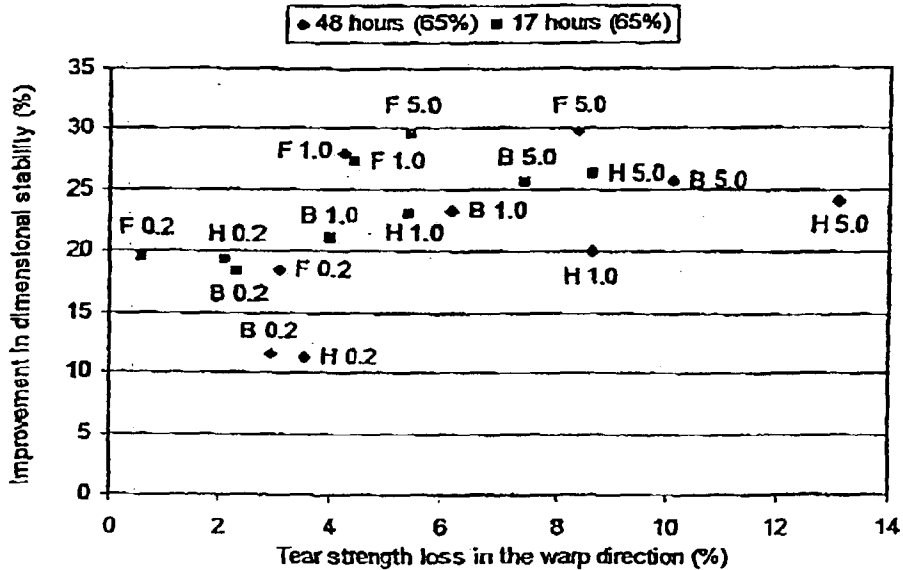
Figure 2 - Percentage improvement (relative to a control treated only with buffer) in dimensional stability v percentage tear strength loss (in the warp direction) of a RS fabric batched for 17 and 48 hours with 0.2, 1.0 and 5.0 mg of Biotouch L, cellulase F and cellulase H per g of fabric (pick-up rate of 65%).
