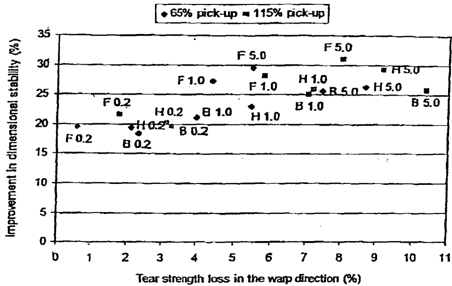
Figure 1 - Percentage improvement (relative to a control treated only with buffer) in dimensional stability v percentage tear strength loss (in the warp direction) of an RS fabric batched for 17 hours with 0.2, 1.0 and 5.0 mg of Biotouch L, cellulase F and cellulase H per g of fabric at different pick-up rates.
