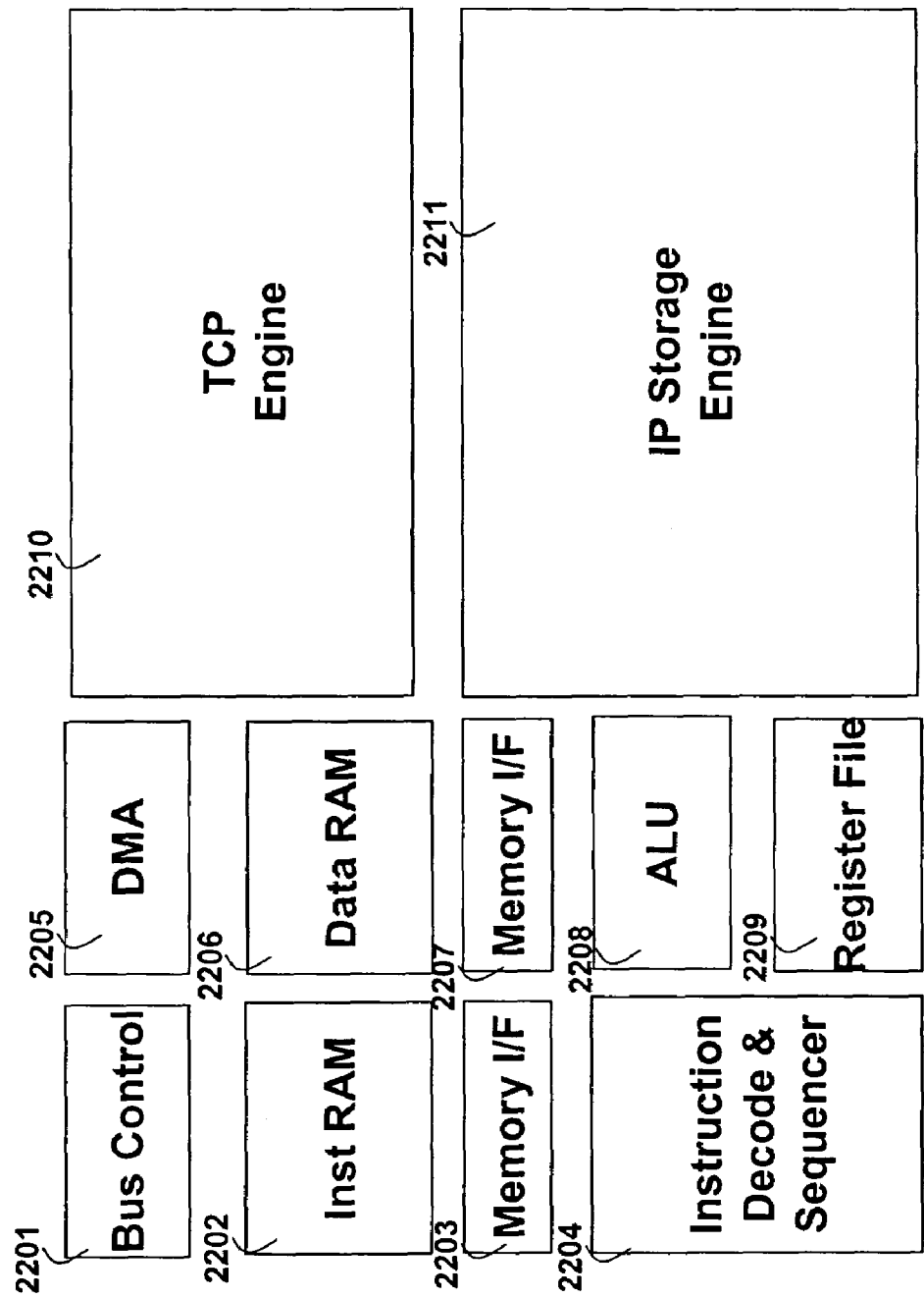
Fig. 22 SAN Packet Processor
