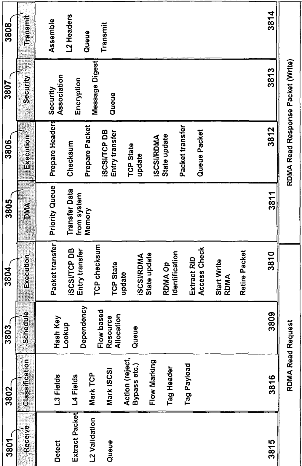
Fig. 38 Write Data Packet Flow (RDMA)
