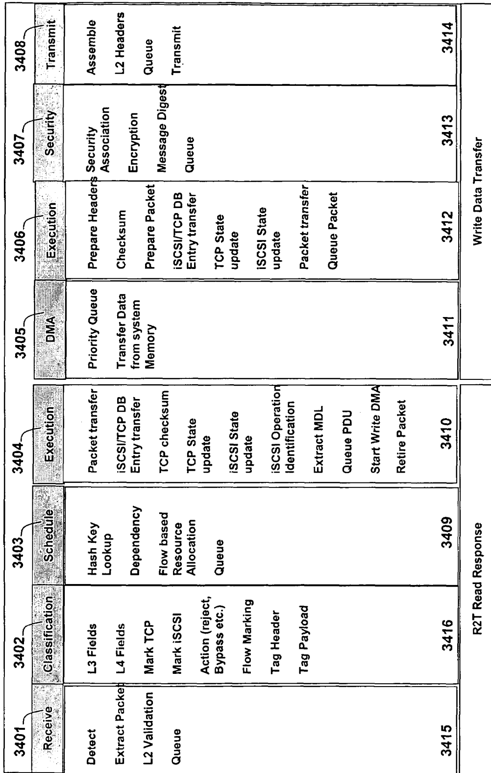
Fig. 34 Write Data Packet Flow
