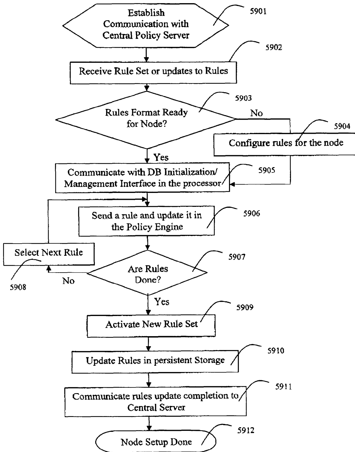
Control Plane Processor/Policy Driver Flow
