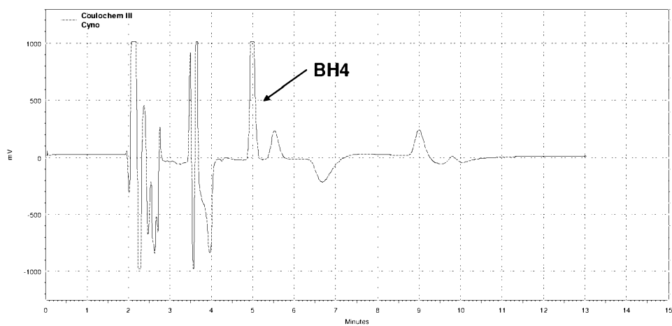
FIGURE 16 - BH4 Chromatogram from Plasma of Cynomolgus Monkeys, 2 hours Post-Administration of the Compound of Example 5 (2% MeOH Mobile Phase)
