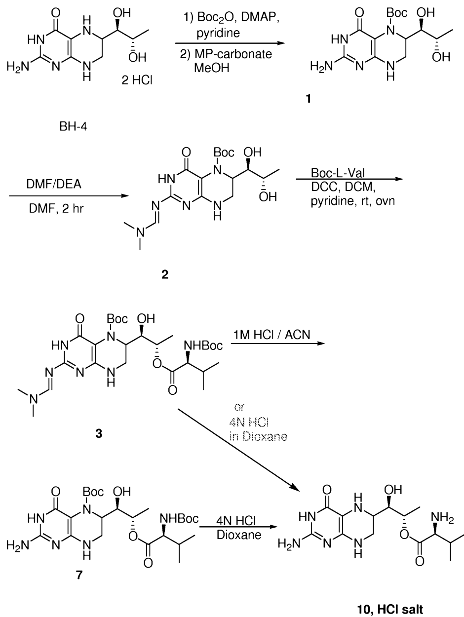
Reaction Scheme (IA')
