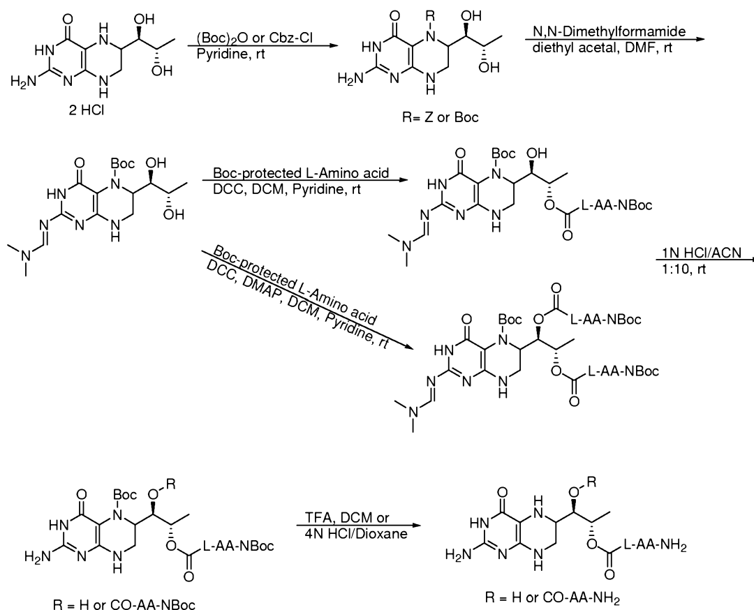
Reaction Scheme (IA)
