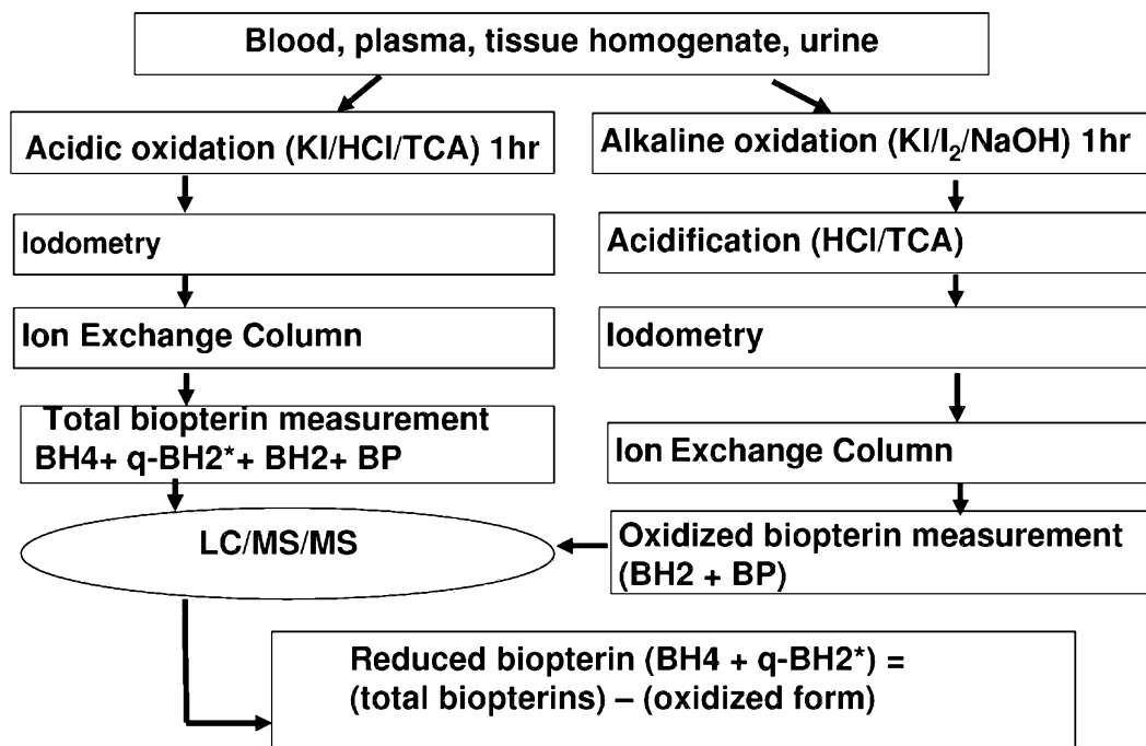
FIGURE 1 - Flow chart of bipterin measurement
