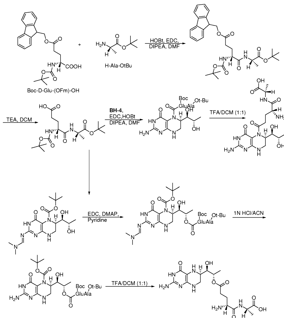
Reaction Scheme (IB)
