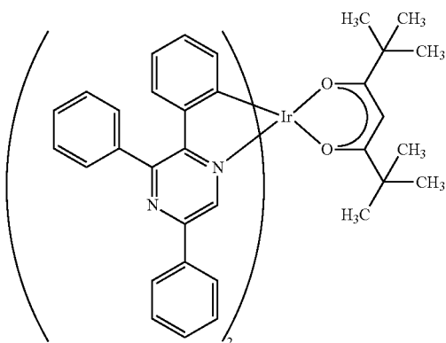
(v) [Ir(tppr) 2 (dpm)]
