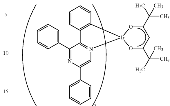
(v) [Ir(tppr) 2 (dpm)]
