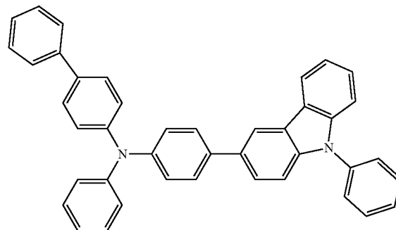
(v) [Ir(tppr) 2 (dpm)]
