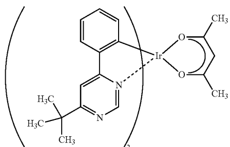
(xi) [Ir(tBuppm) 2 (acac)]
