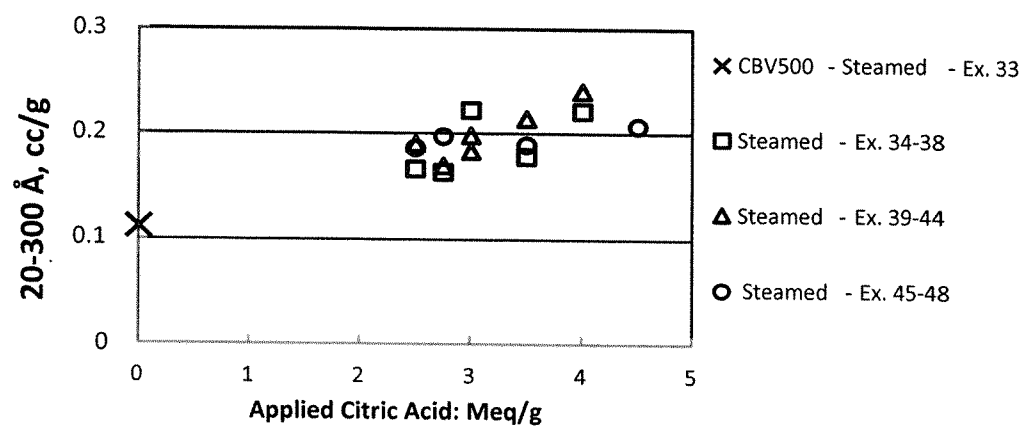
20 – 300 Å Mesopore Variation Associated with the Citric Acid Concentration in the “Steamed” Samples
