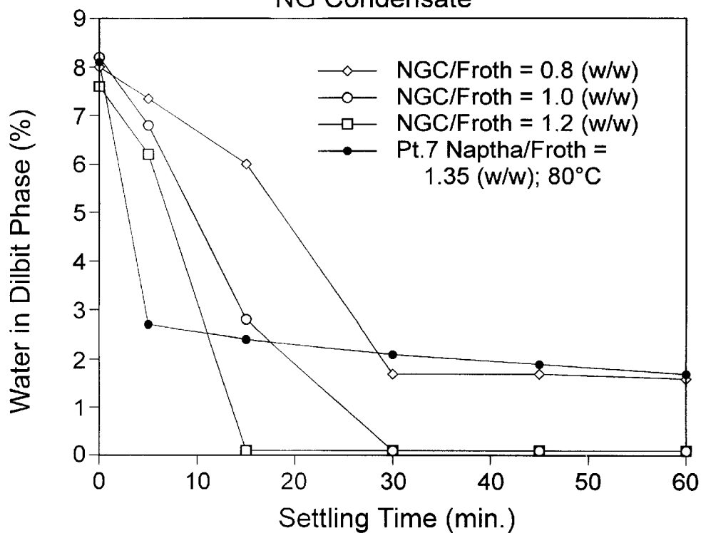
FIG. 4. Water Removal at Different Solvent to Froth Ratios; 40°C Gravity Settling; NG Condensate
