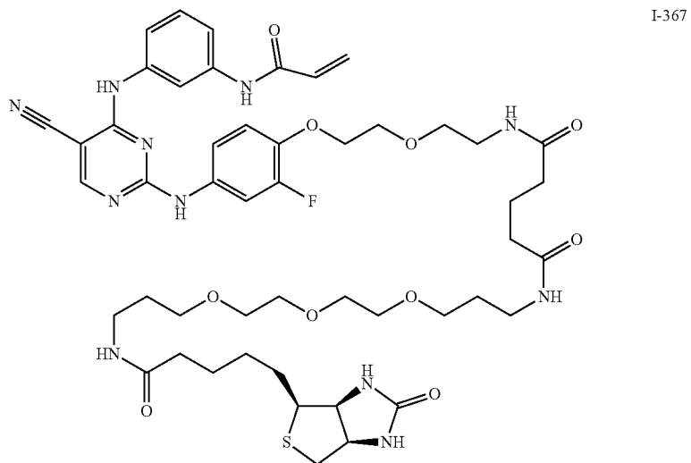
Exemplary Compounds
