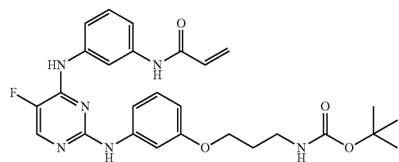
tert-Butyl 3-(3-(4-(3-(2-amino-5-fluoropyrimidin-2-ylamino)phenoxy)propylcarbamate
