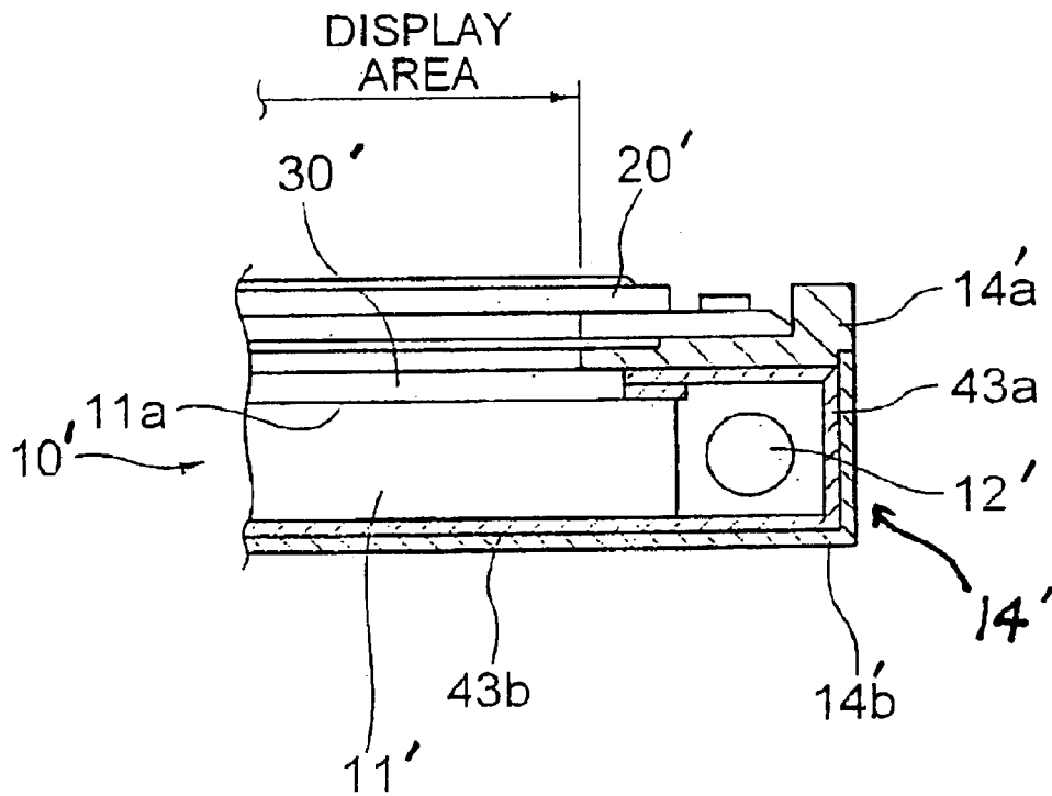
FIG. 8 PRIOR ART
