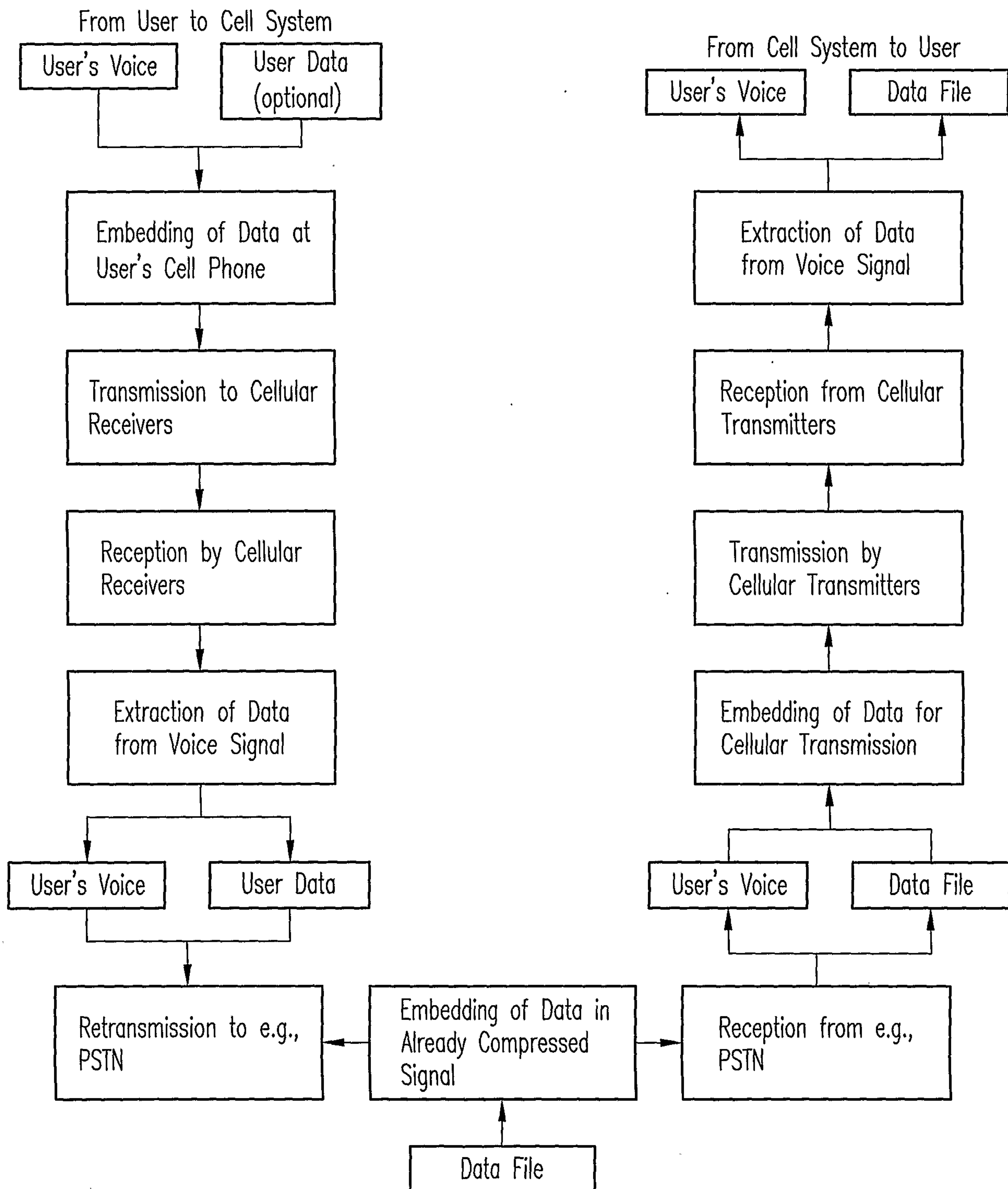
Cellular Network with Data Embedding
