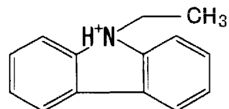
Compound No. A12
