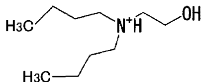
Compound No. A19
