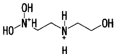
Compound No. A27
