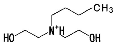
Compound No. A24
