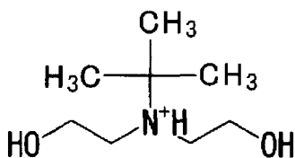
Compound No. A25
