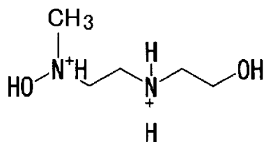
Compound No. A33
