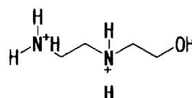
Compound No. A57
