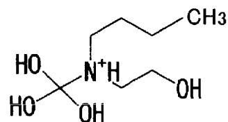
Compound No. A18
