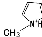
Compound No. A12
