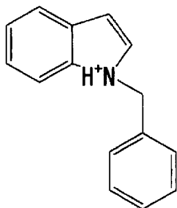
Compound No. A13
