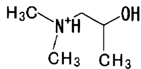
Compound No. A31
