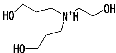
Compound No. A32
