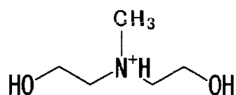
Compound No. A22
