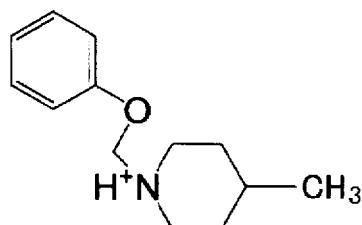
Compound No. A4
