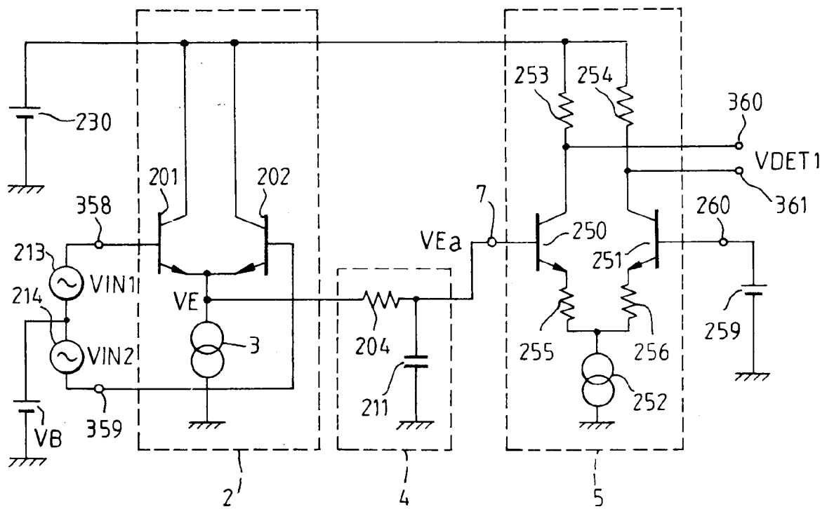
Fig.1 (Prior Art)
