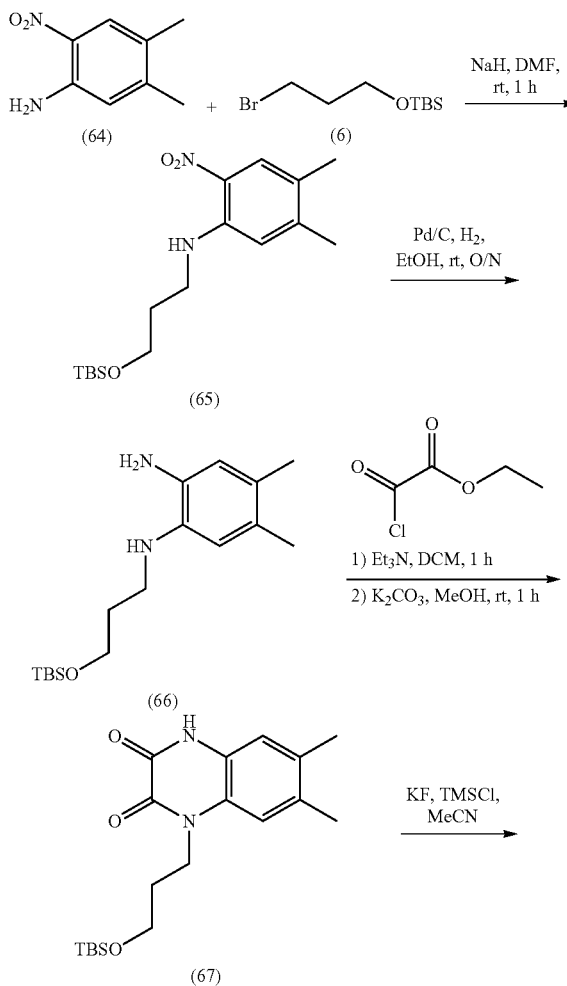
Scheme 30
