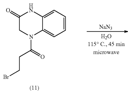
Scheme 26
