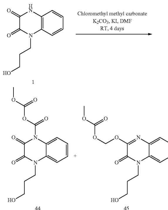
Scheme 43
