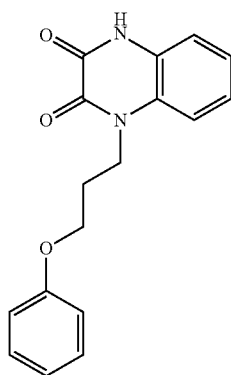
1-(3-phenoxypropyl)quinoxaline-2,3(1H,4H)-dione;
