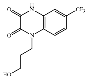
Scheme 35
