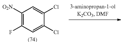
Scheme 33
