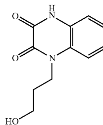
1-(3-hydroxypropyl)quinoxaline-2,3(1H,4H)-dione;
