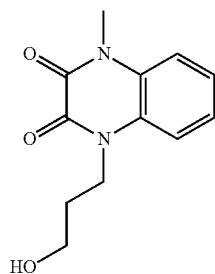
1-(3-hydroxypropyl)-4-methylquinoxaline-2,3(1H,4H)-dione;
