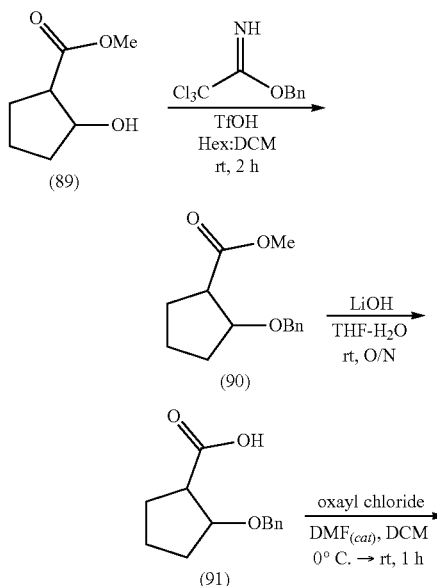
Scheme 38
