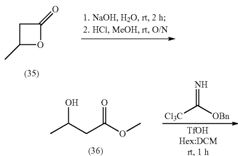
Scheme 23
