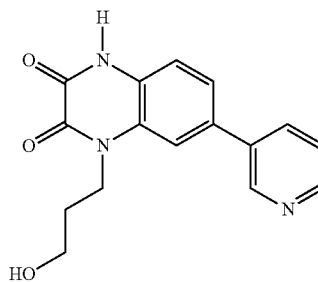
1-(3-hydroxypropyl)-6-methylquinoxaline-2,3(1H,4H)-dione;
