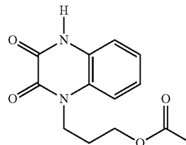
3-(2,3-dioxo-3,4-dihydroquinoxalin-1(2H)-yl)propyl acetate;
