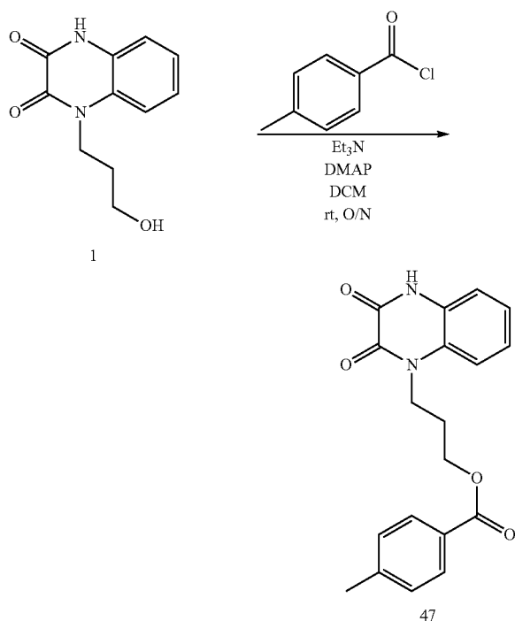
Scheme 45
