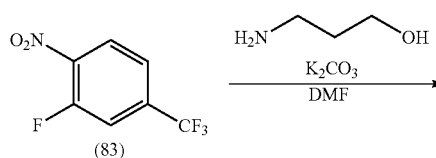
Scheme 36
