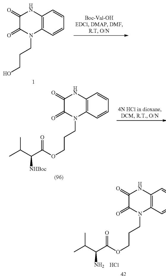
Scheme 41
