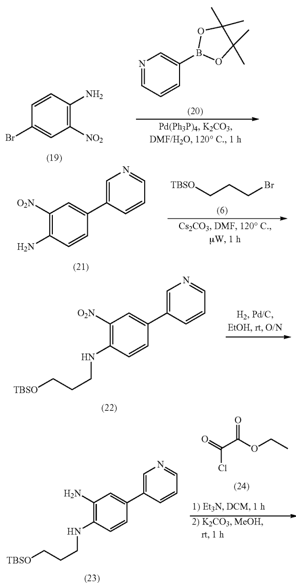
Scheme 17
