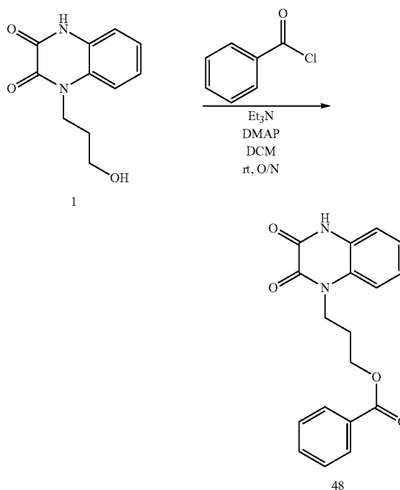
Scheme 46
