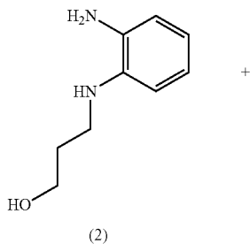
Scheme 16
