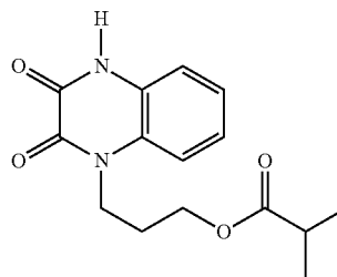
3-(2,3-dioxo-3,4-dihydroquinoxalin-1(2H)-yl)propyl isobutyrate;
