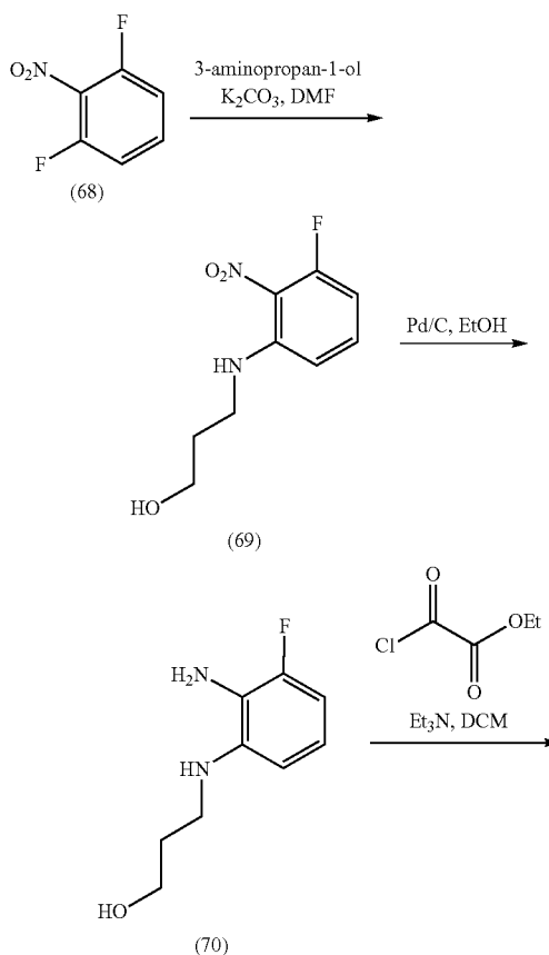
Scheme 31
