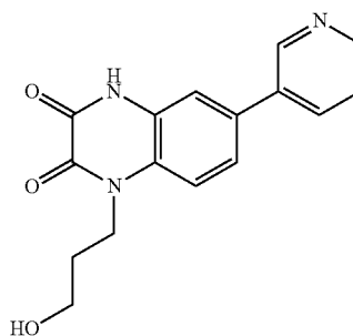
1-(3-hydroxypropyl)-6-(pyridin-3-yl)quinoxaline-2,3(1H,4H)-dione;
