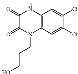
Scheme 33
