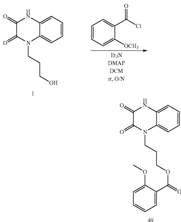
Scheme 47
