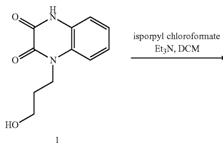
Scheme 42
