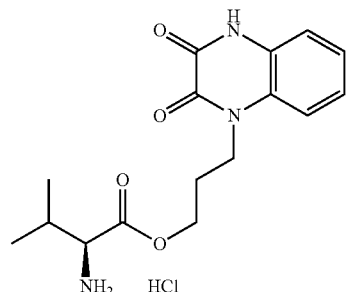
Scheme 41
