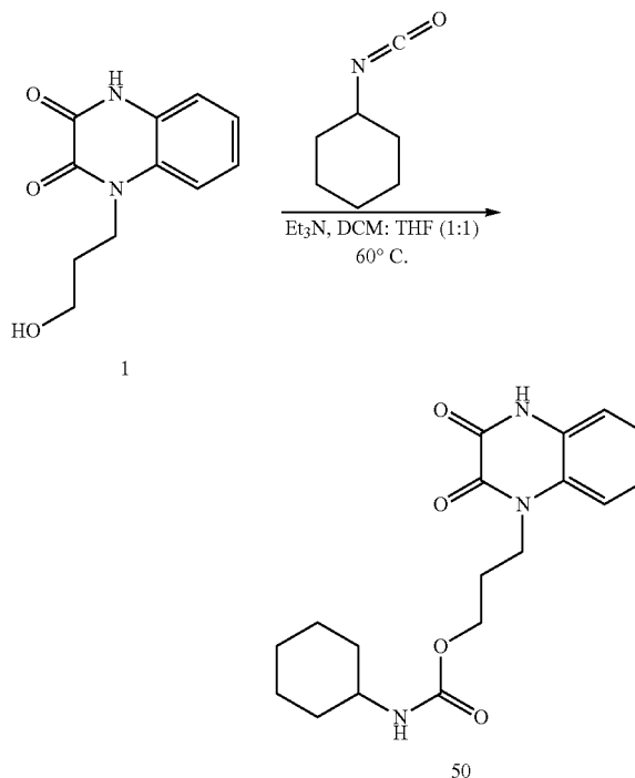
Scheme 48
