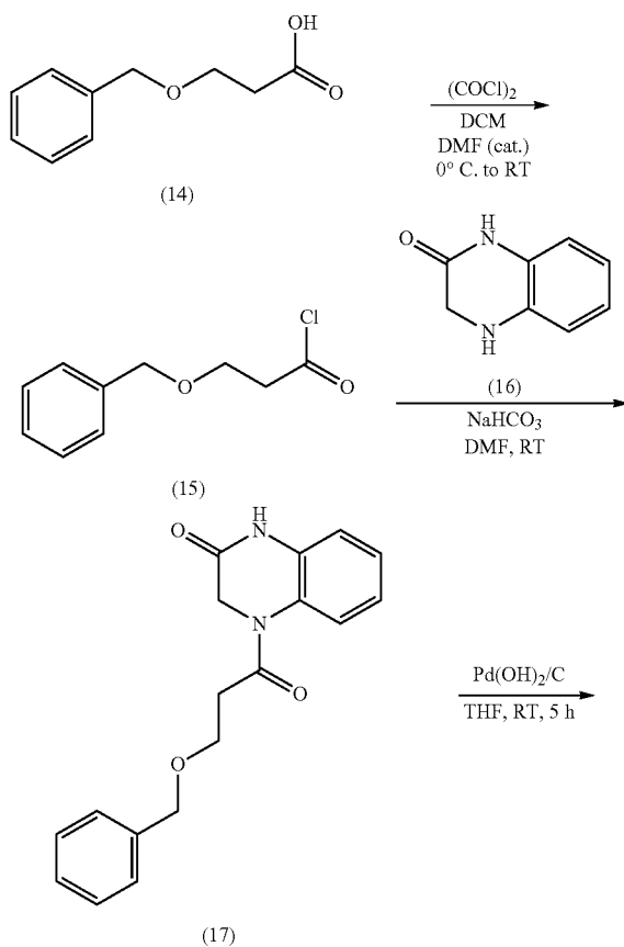
Scheme 15
