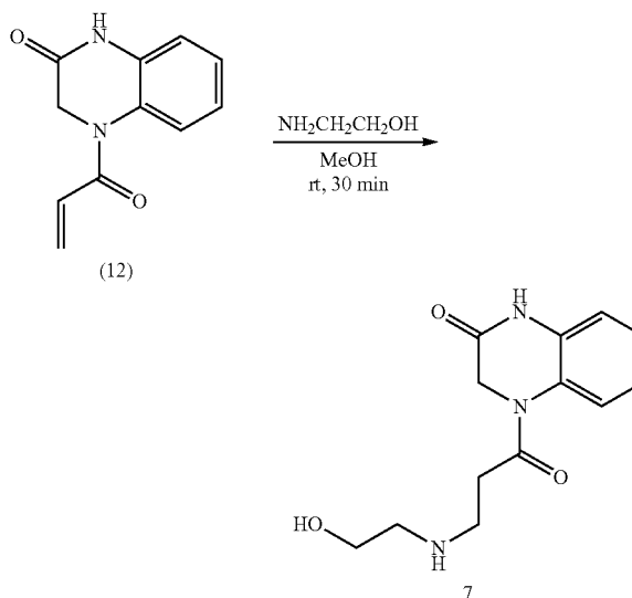
Scheme 12
