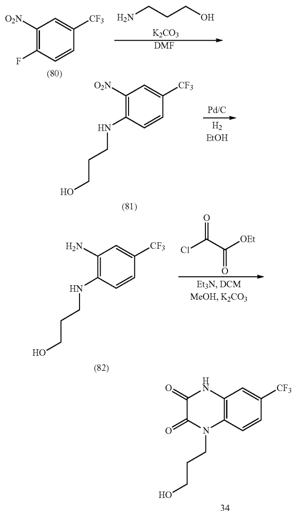
Scheme 35
