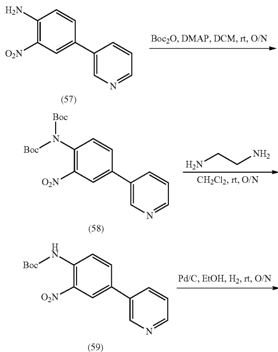
Scheme 29
