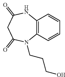
1-(3-hydroxypropyl)-1H-benzo[b][1,4]diazepine-2,4(3H,5H)-dione;
