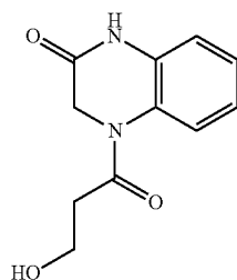
Scheme 15
