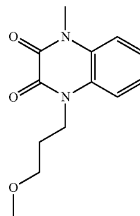
1-(3-methoxypropyl)-4-methylquinoxaline-2,3(1H,4H)-dione;
