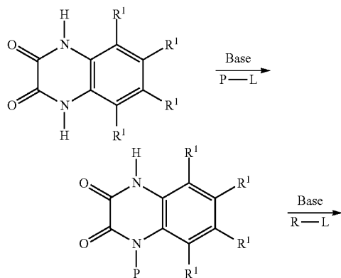
Scheme 3
