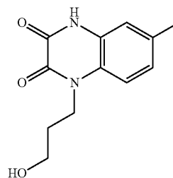
1-(3-hydroxypropyl)-6-methylquinoxaline-2,3(1H,4H)-dione;
