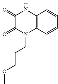
1-(3-methoxypropyl)quinoxaline-2,3(1H,4H)-dione;
