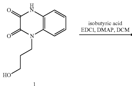
Scheme 40
