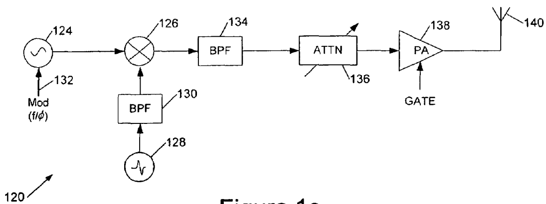
Figure 1c (PRIOR ART)
