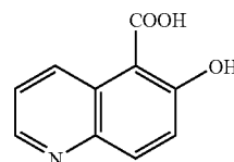
6-hydroxy-quinoline-5-carboxylic acid
