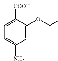
2-ethoxy-4-aminobenzoic acid
