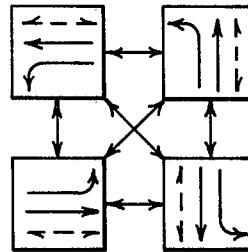
SIGNAL SEQUENCE
