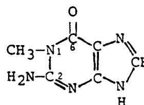
1-Methylguanine
