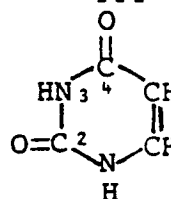
Thymine (5-methyl-2,4-dioxypyrimidine)
