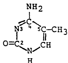
5-Methylcytosine
