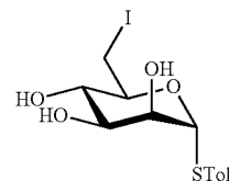
p-Tolyl 6-iodo-1-thio- \alpha -D-mannopyranoside (S2)
