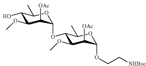
2-O-Acetyl-3-O-methyl- \alpha -D-rhamnopyranoside-(1 \rightarrow 4)-2-(tert-butoxycarbonyl)amino]ethyl 2-O-acetyl-3-O-methyl- \alpha -D-rhamnopyranoside (S12)
