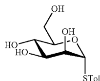
p-Tolyl 1-thio- \alpha -D-mannopyranoside (S1)
