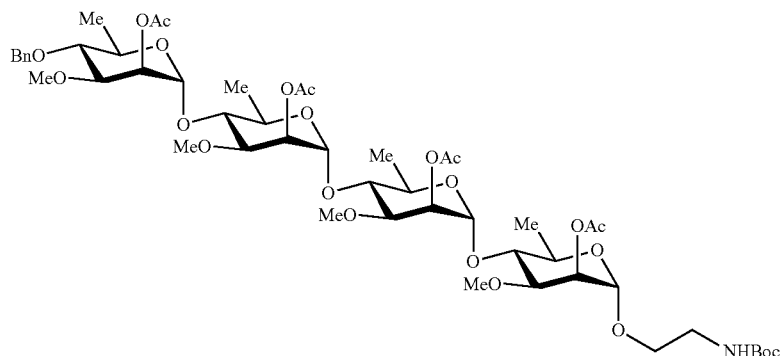
2-O-Acetyl-4-O-benzyl-3-O-methyl- \alpha -D-rhamnopyranoside-(1 \rightarrow 4)-2-O-acetyl-3-O-methyl- \alpha -D-rhamnopyranoside-(1 \rightarrow 4)-2-O-acetyl-3-O-methyl- \alpha -D-rhamnopyranoside-(1 \rightarrow 4)-2-(tert-butoxycarbonyl)amino]ethyl 2-O-acetyl-3-O-methyl- \alpha -D-rhamnopyranoside (S15)
