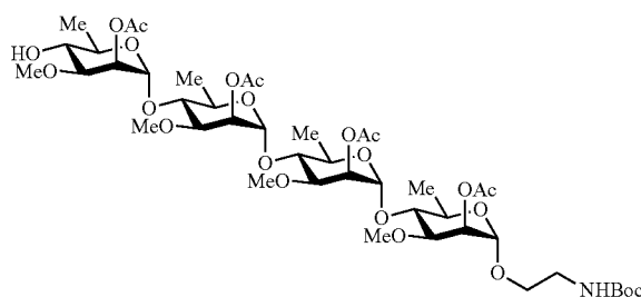
2-O-Acetyl-3-O-methyl- \alpha -D-rhamnopyranoside-(1 \rightarrow 4)-2-O-acetyl-3-O-methyl- \alpha -D-rhamnopyranoside-(1 \rightarrow 4)-2-O-Acetyl-3-O-methyl- \alpha -D-rhamnopyranoside-(1 \rightarrow 4)-2-(tert-butoxycarbonyl)amino]ethyl 2-O-acetyl-3-O-methyl- \alpha -D-rhamnopyranoside (S16)
