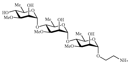
3-O-Methyl- \alpha -D-rhamnopyranoside-(1 \rightarrow 4)-3-O-methyl- \alpha -D-rhamnopyranoside-(1 \rightarrow 4)-2-(tert-butoxycarbonyl)amino]ethyl 3-O-methyl- \alpha -D-rhamnopyranoside (S19)
