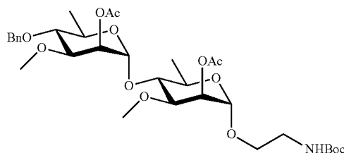
2-O-Acetyl-4-O-benzyl-3-O-methyl- \alpha -D-rhamnopyranoside-(1 \rightarrow 4)-2-(tert-butyloxycarbonyl)amino]ethyl 2-O-acetyl-3-O-methyl- \alpha -D-rhamnopyranoside (S11 (Same as 23 Above))
