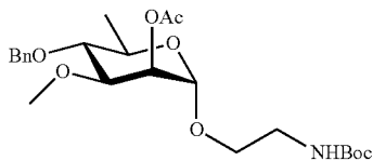
2-(tert-Butyloxycarbonylamido)ethyl 2-O-acetyl-4-O-benzyl-3-O-methyl- \alpha -D-rhamnopyranoside (S9 (Same as 21 Above))
