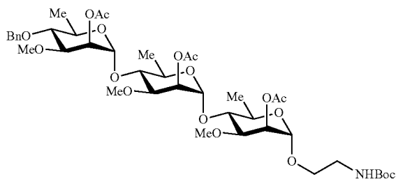
2-O-Acetyl-4-O-benzyl-3-O-methyl- \alpha -D-rhamnopyranoside-(1 \rightarrow 4)-2-O-acetyl-3-O-methyl- \alpha -D-rhamnopyranoside-(1 \rightarrow 4)-2-(tert-butoxycarbonyl)amino]ethyl 2-O-acetyl-3-O-methyl- \alpha -D-rhamnopyranoside (S13)
