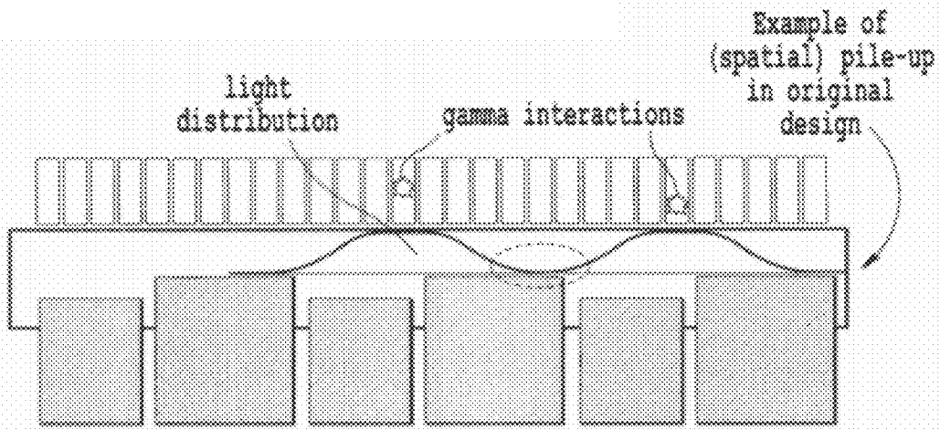
Fig. 4A ORIGINAL DESIGN (NON-SEGMENTED), SIDE VIEW
