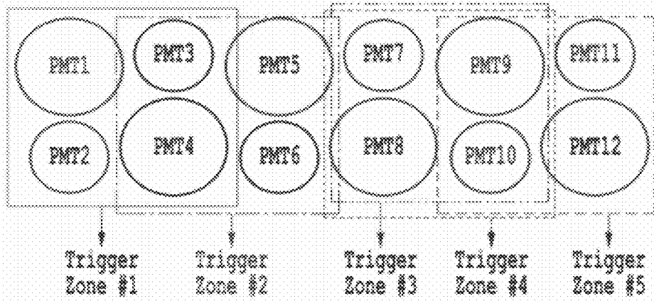
Fig. 4B TRIGGER ZONES (OVERLAPPING), TOP VIEW
